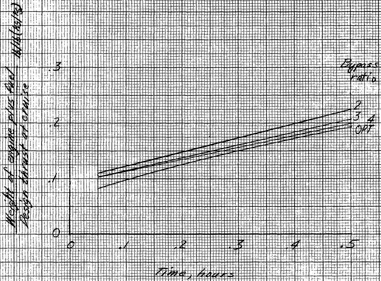
Figure 12. Optimum and fixed bypass ratio dry turbofan engines scaled to produce 20000 lb (9100 kg) net thrust at M=0.3 , sea-level using H_2 fuel. Weight factor = 1.0. Turbine inlet temperature = 2500°F (1510°C).
