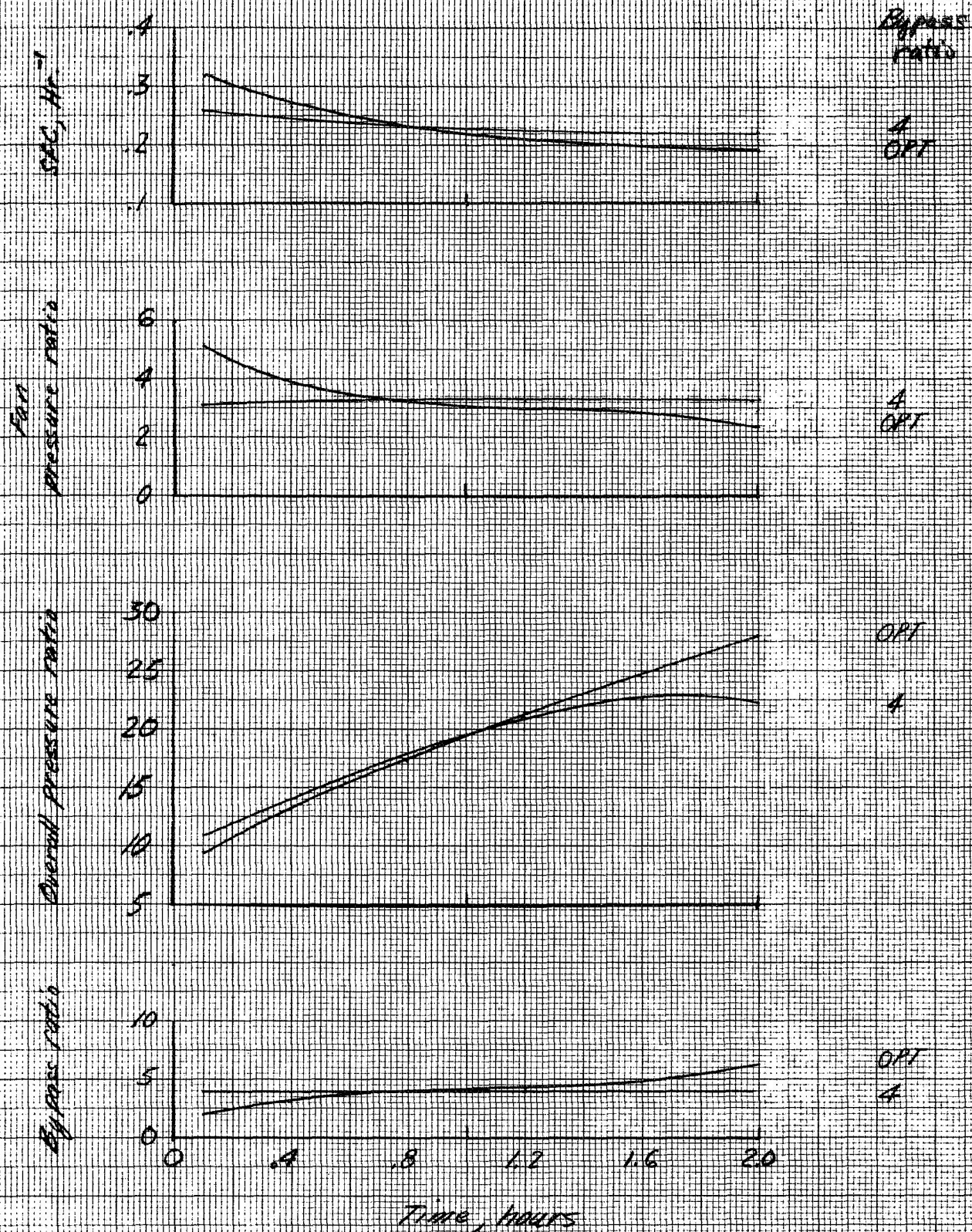
Figure 5.- Engine parameters for dry turbofan engines scaled to produce 25000lb (11300kg) net thrust at M=0.4 , 20000 feet (6100m) using H_2 fuel. Weight factor = 1.0. Turbine inlet temperature = 2500°R (1370°C)
