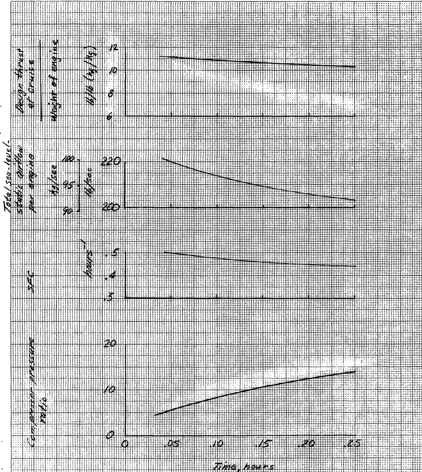
Figure 10- Engine parameters for dry turbojets scaled to produce 20000 lb (9160 kg) net thrust at M=0.3 , sea-level using H_2 fuel. Weight factor = 1.0, turbine-inlet temperature = 2500^\circ C ( 4500^\circ F )
