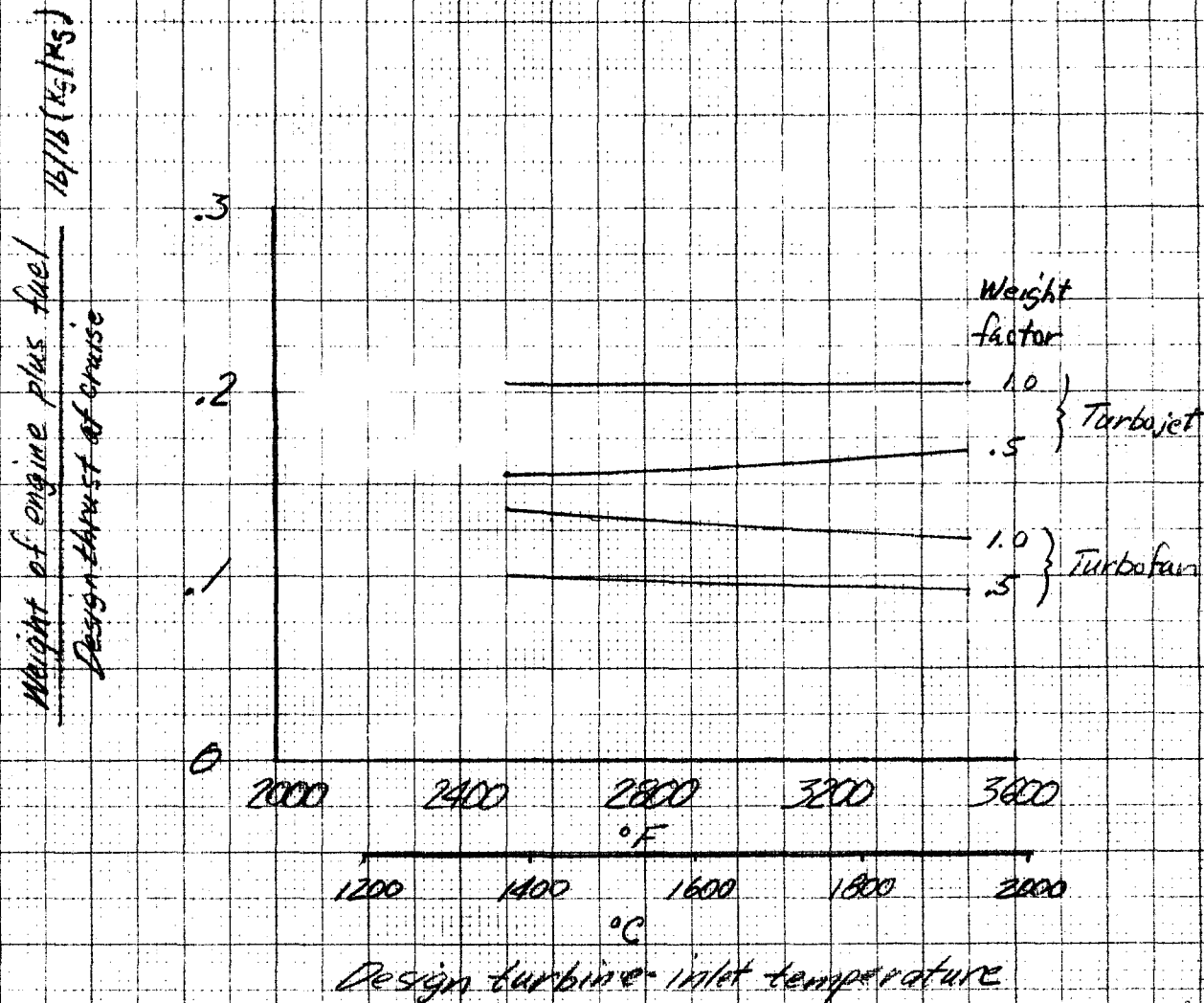
Figure 14. - Summary of optimized turbafans and turbojets scaled to produce 30000 lb (1360 kg) jet thrust at M=0.3 , sea-level. H_2 fuel. Cruise time = .25 hours.
