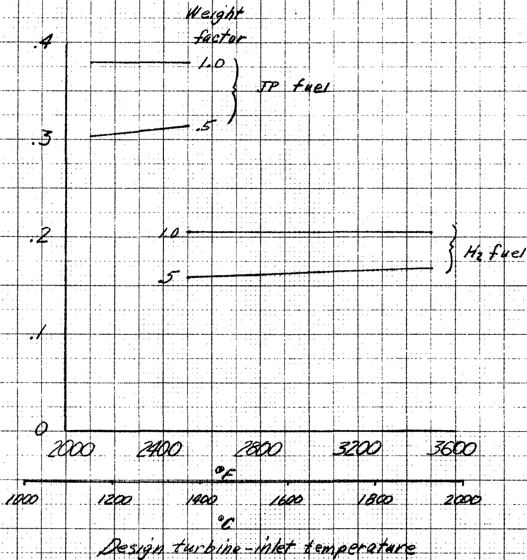
Figure 11. - Summary of optimized turbojet engines scaled to produce 30000 lb (9160 kg) net thrust at M=0.3 , sea-level. Cruise time = .25 hours.
