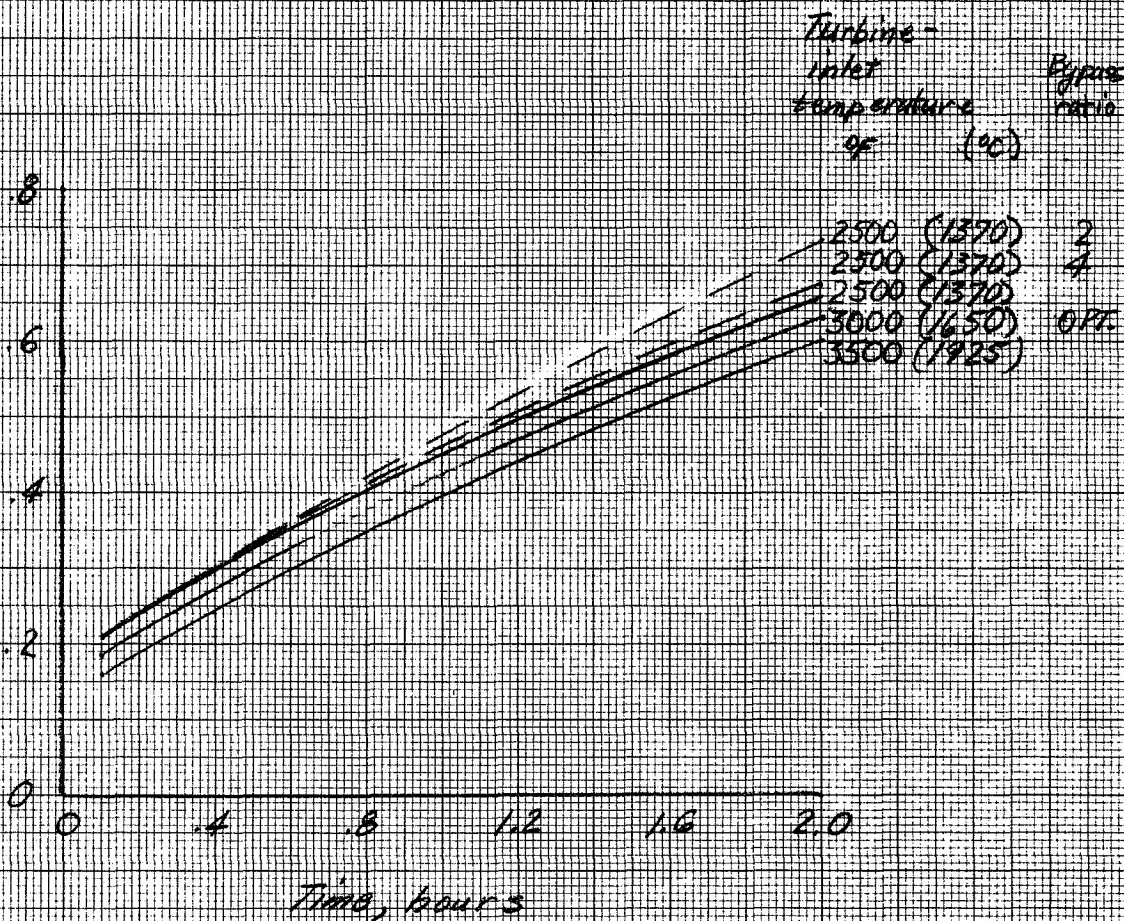
Figure 4.- Comparison of optimum and fixed bypass ratio dry turbofan engines scaled to produce 25000 lb (11300 kg) net thrust at M=0.8 , 20000 feet (6100m) using H_2 fuel. Weight factor = 1.0.
