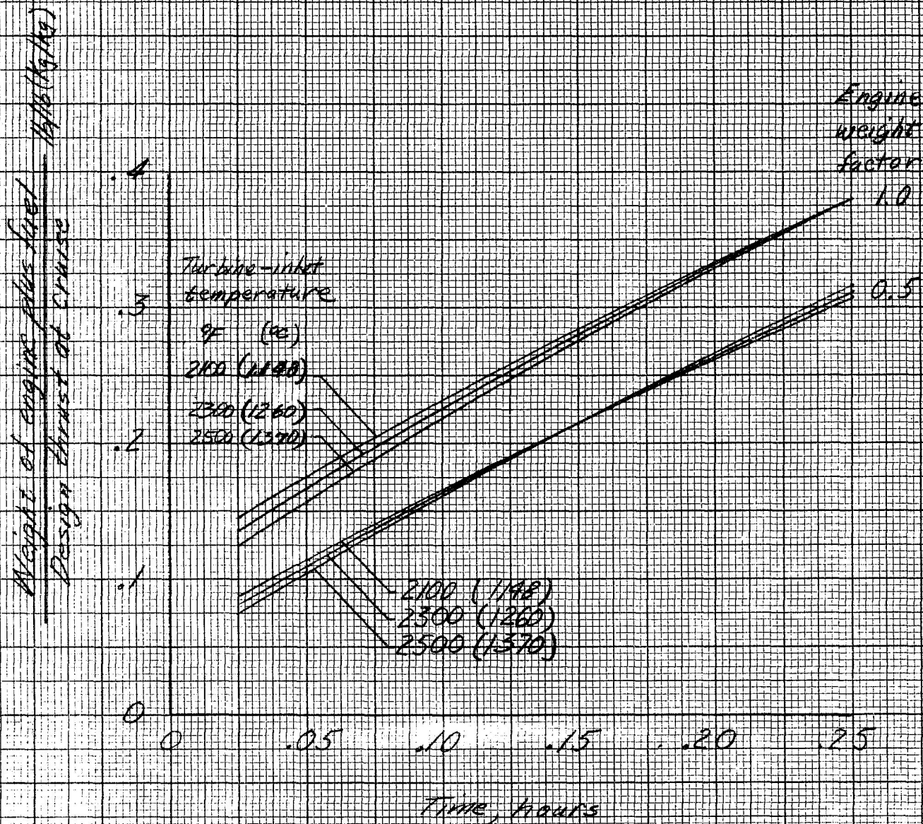
Figure 7.- Optimum dry turbojet engine scaled to produce 20000N(4500kg) net thrust at MN=0.3 , sea-level using JP.
