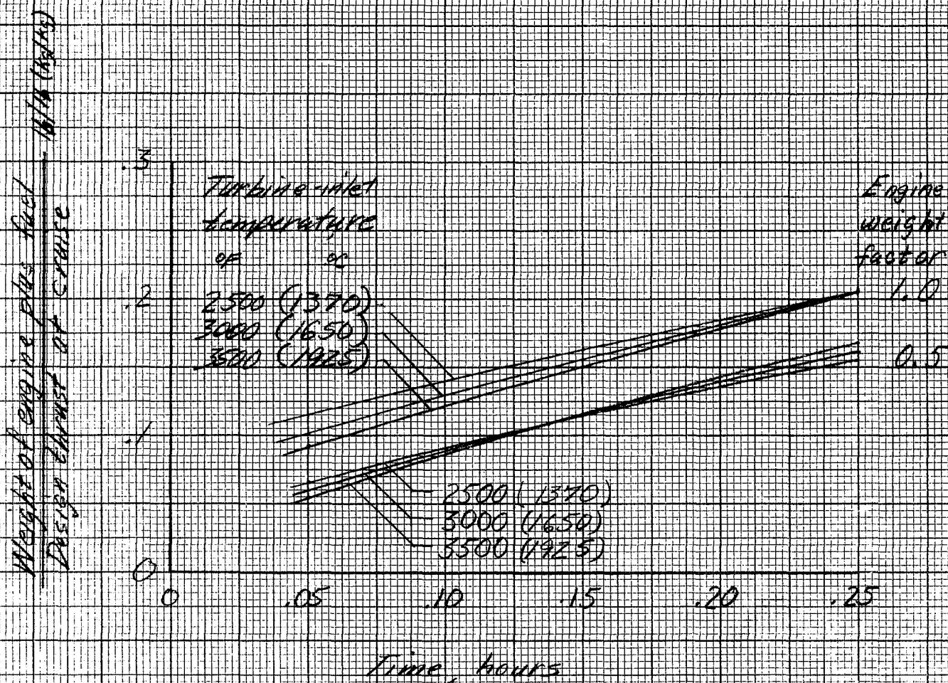
Figure 9.- Optimum dry turbojet engine scaled to produce 20000 lb (9160 kg) net thrust at M=0.3 , sea level using H_2 fuel.
