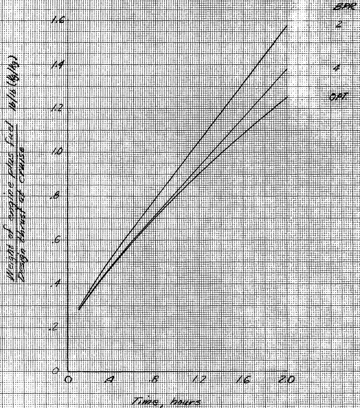
Figure 3.- Comparison of optimum and fixed bypass ratio dry turbofan engines scaled to produce 25000 lb (11300kg) net thrust at M=0.4 , 20000 feet (6100m) using JP fuel. Weight factor = 1.0. Turbine inlet temperature = 2500°F (1370°C).
