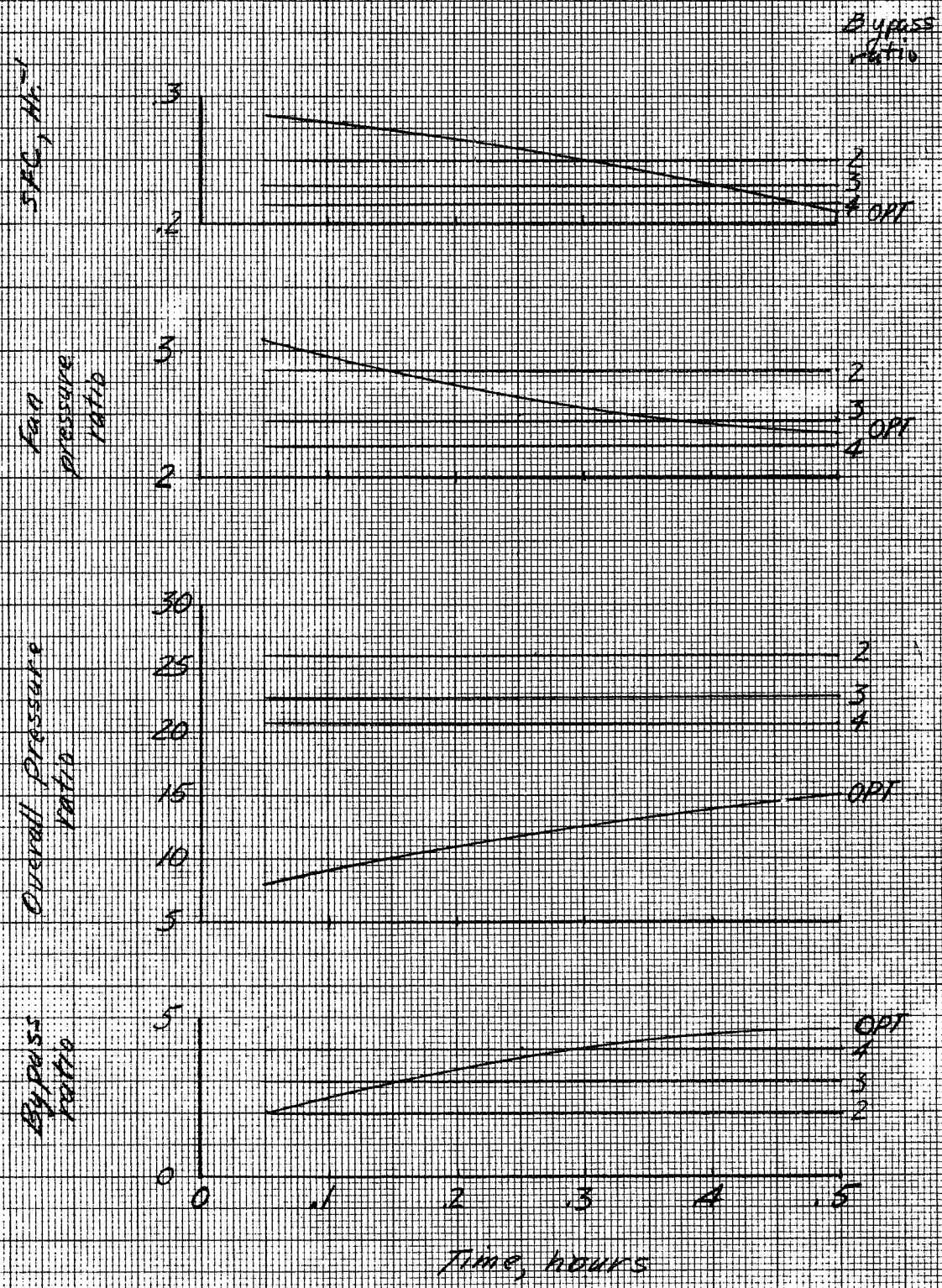
Figure 13.- Engine parameters for dry turbofan engines scaled to produce 20000lb (9160kg) net thrust at M=0.3 , sea-level using H_2 fuel. Weight factor = 1.0. Turbine inlet temperature = 2500°R (1370°C)
