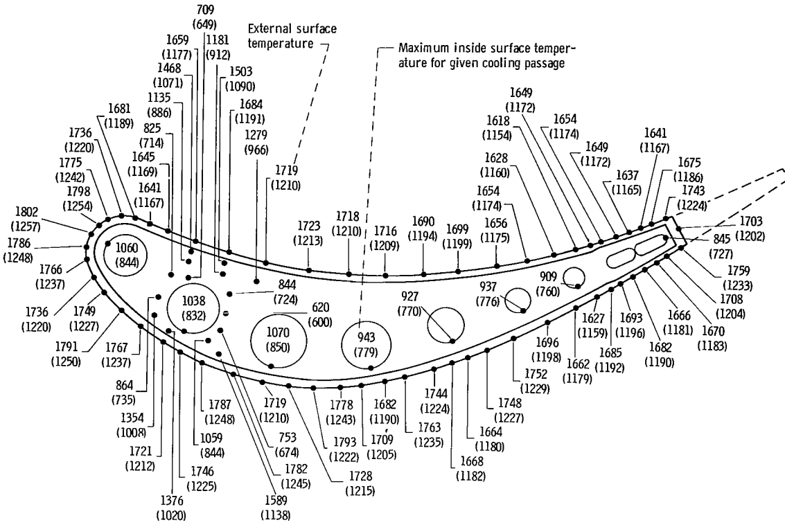
Figure 6. - Temperature distribution in methane-cooled vane under cruise conditions. (Temperatures are in °F (K).)
