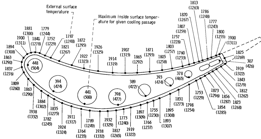
Figure 7. - Temperature distribution in methane-cooled vane under takeoff conditions. (Temperatures are in °F (K).)
