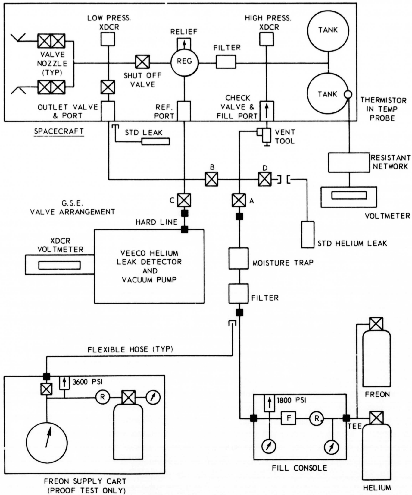
Figure 3. ACS Fill Procedure Equipment Setup
