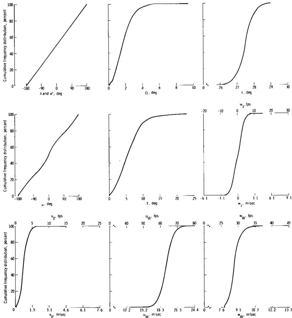
Figure A-1. - Cumulative frequency distributions of impact parameters for a fully developed sea with a 28.5-knot surface wind and a 1-percent two-parachute probability.
