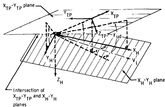
(b) Local horizontal and impact-tangent-plane axis systems.
