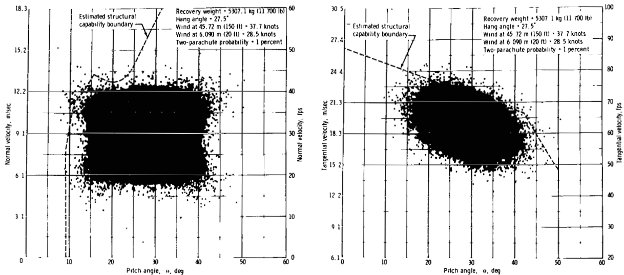
(a) Normal velocity compared with impact angle.
