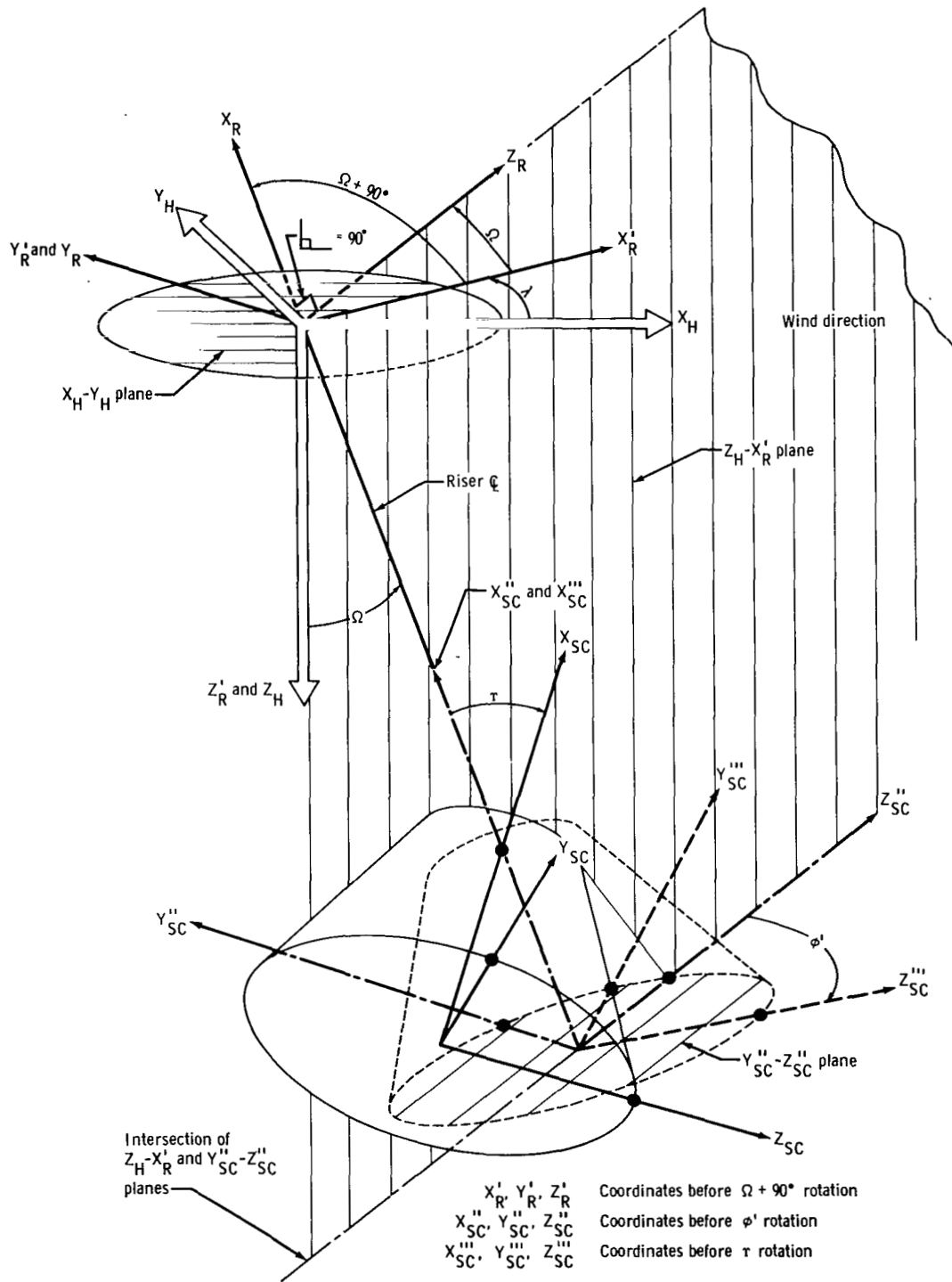
(a) Local horizontal, riser, and spacecraft axis systems.
