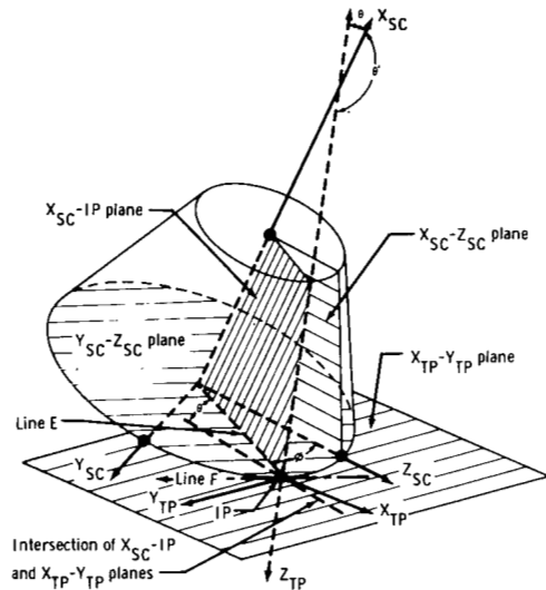
Figure 2. - Angular relation of the spacecraft to the impact tangent plane.
