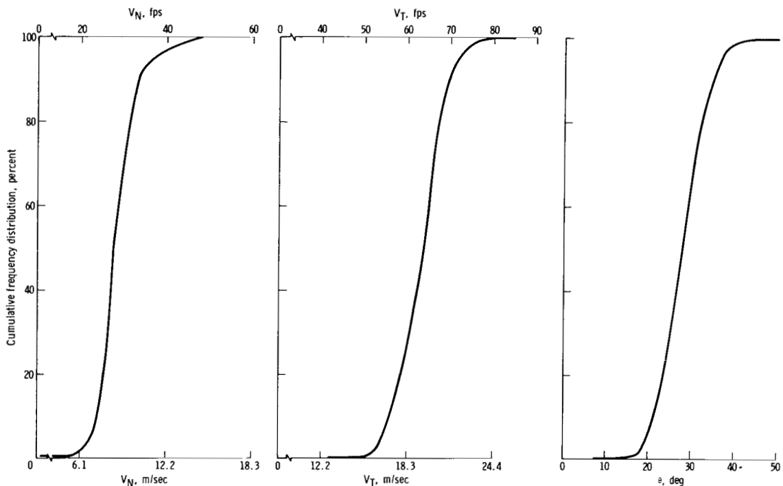
Figure A-2. - Cumulative frequency distributions of water impact conditions for a fully developed sea with a fixed 28.5-knot surface wind and a 1-percent two-parachute probability.
