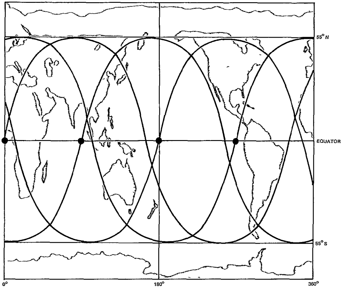
Exhibit 6 Orbital Pattern Four Satellites
