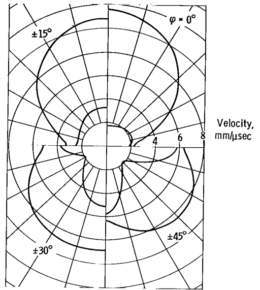
Figure 3. - Velocity surfaces for 55 percent graphite fiber-epoxy matrix plates at various layup angles.
