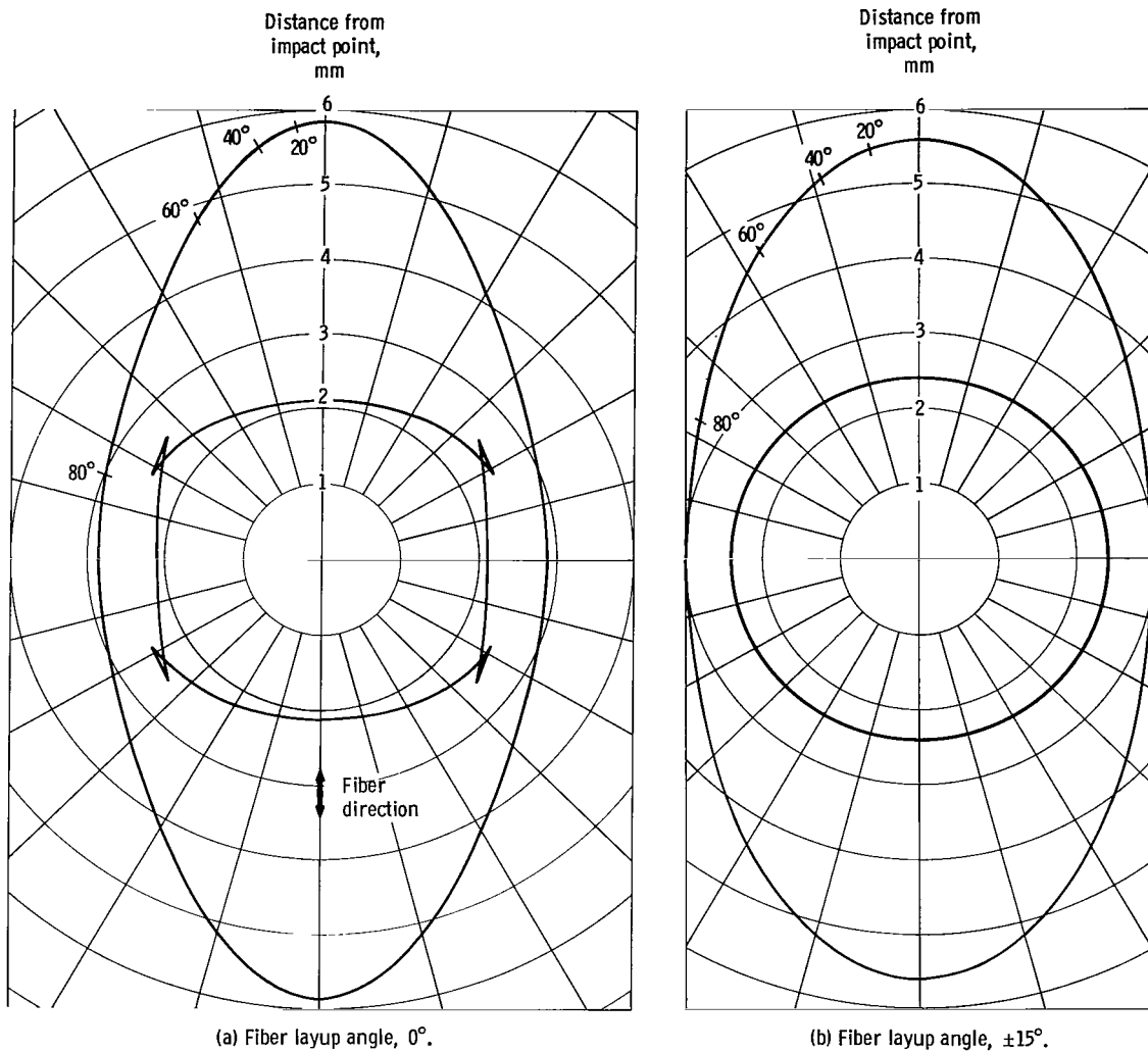
Figure 7. - Wave surfaces at 1.15 microseconds after impact for 55 percent glass fiber - epoxy matrix plates.
