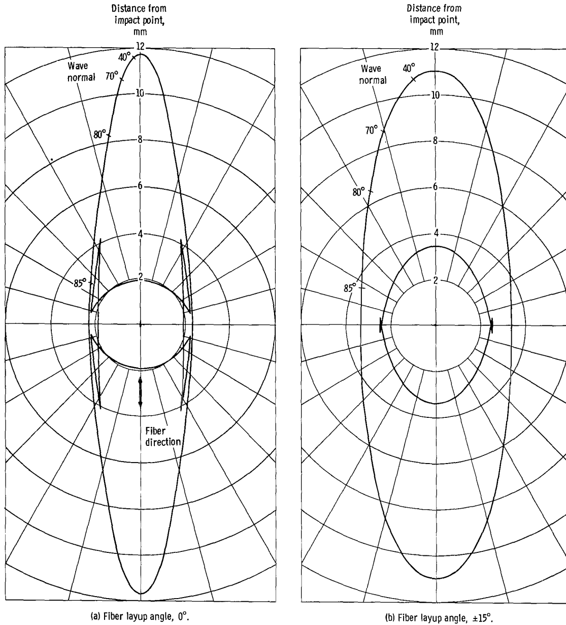
Figure 4. - Wave surfaces at 1 microsecond after impact for 55 percent graphite fiber - epoxy matrix plates.
