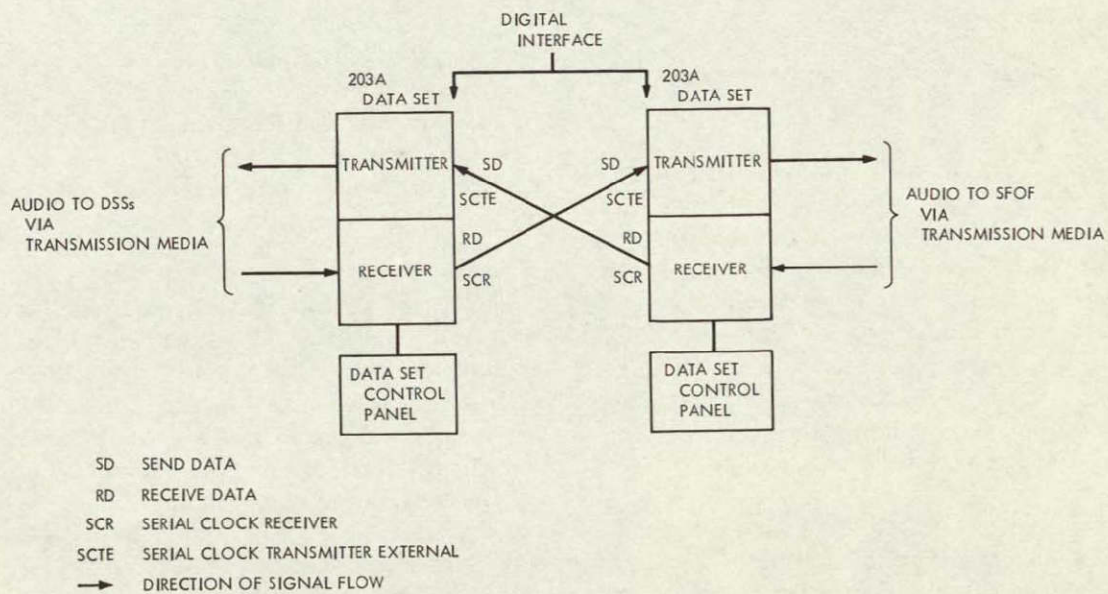
Fig. 2. Interconnect diagram
