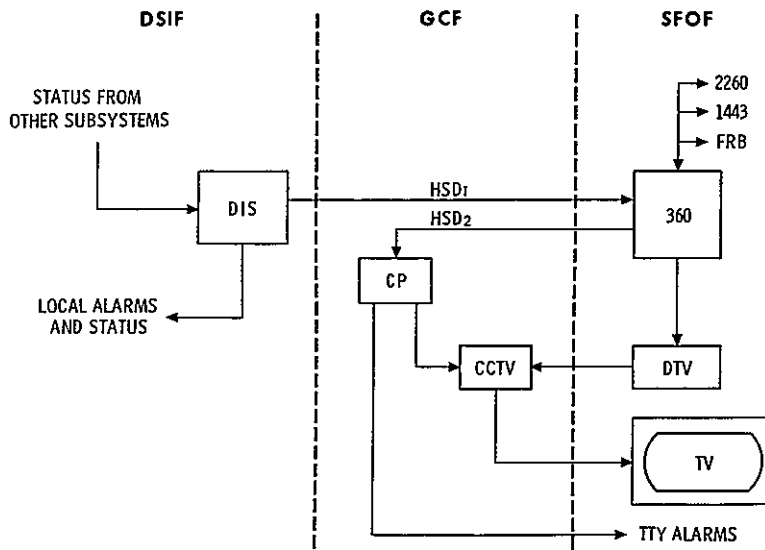
Fig 6 Monitor system
