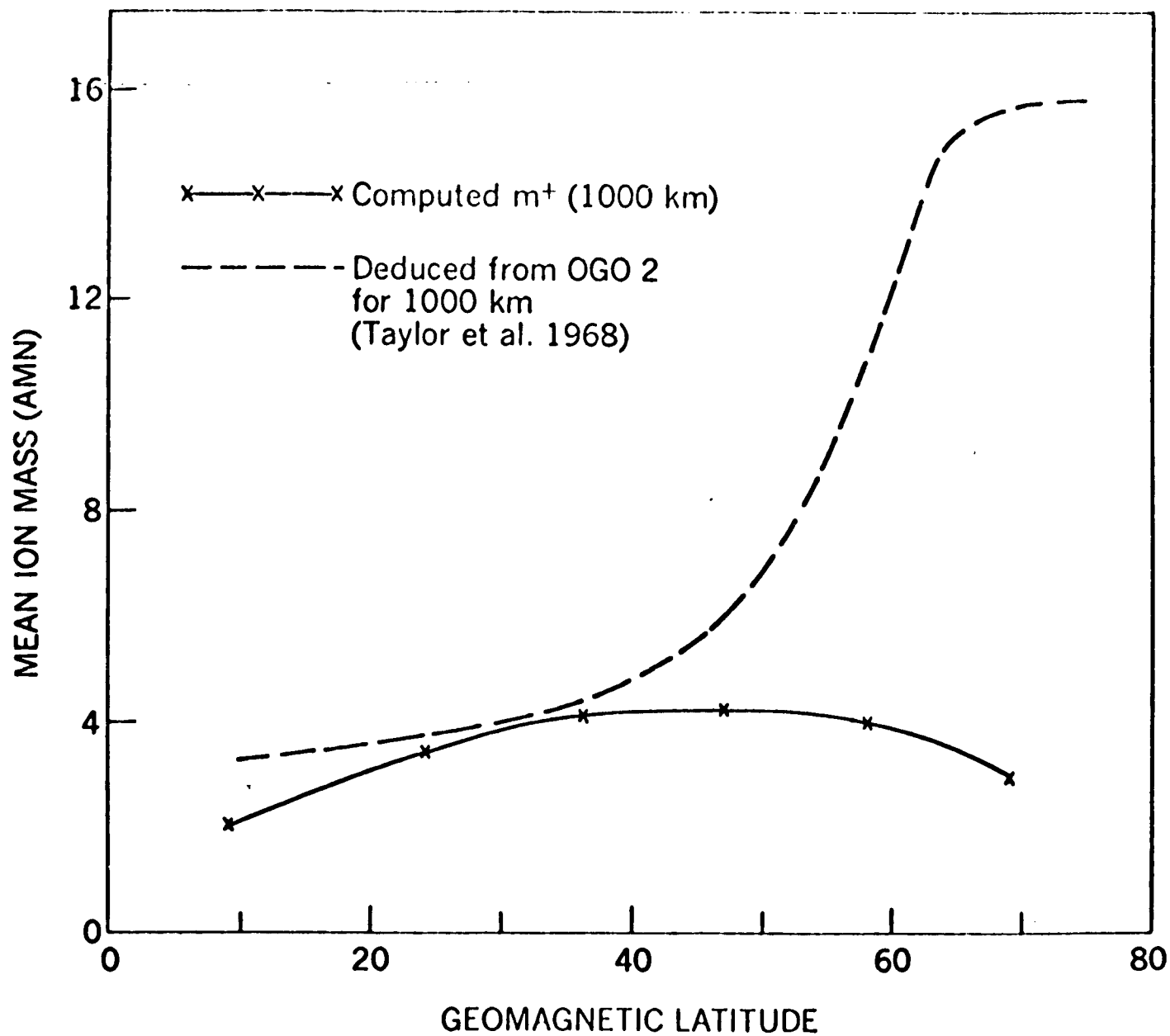
Figure 6. Computed mean ion mass at 1000 km. For comparison the mean ion mass deduced for 1000 km from OGO 2 results (Taylor et al., 1968) is shown for dusk, October 1965.
