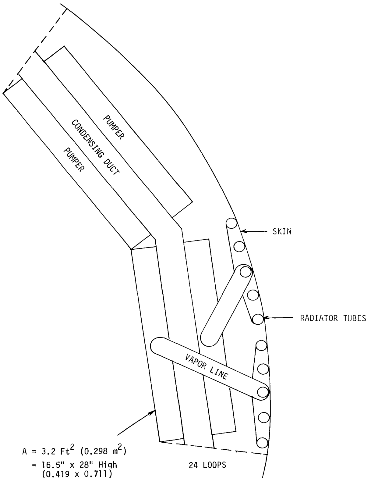
FIGURE 5-11. TWENTY-FOUR LOOP SYSTEM - RADIATOR COUPLING
