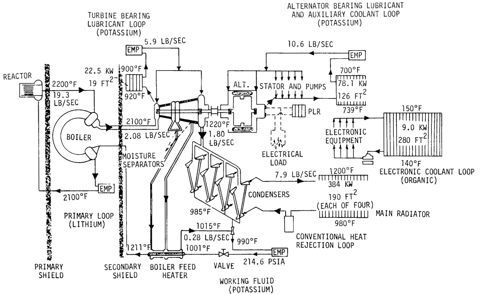
Figure 2-1. ADVANCED RANKINE POWER SYSTEM NOMINAL 300 KW e
