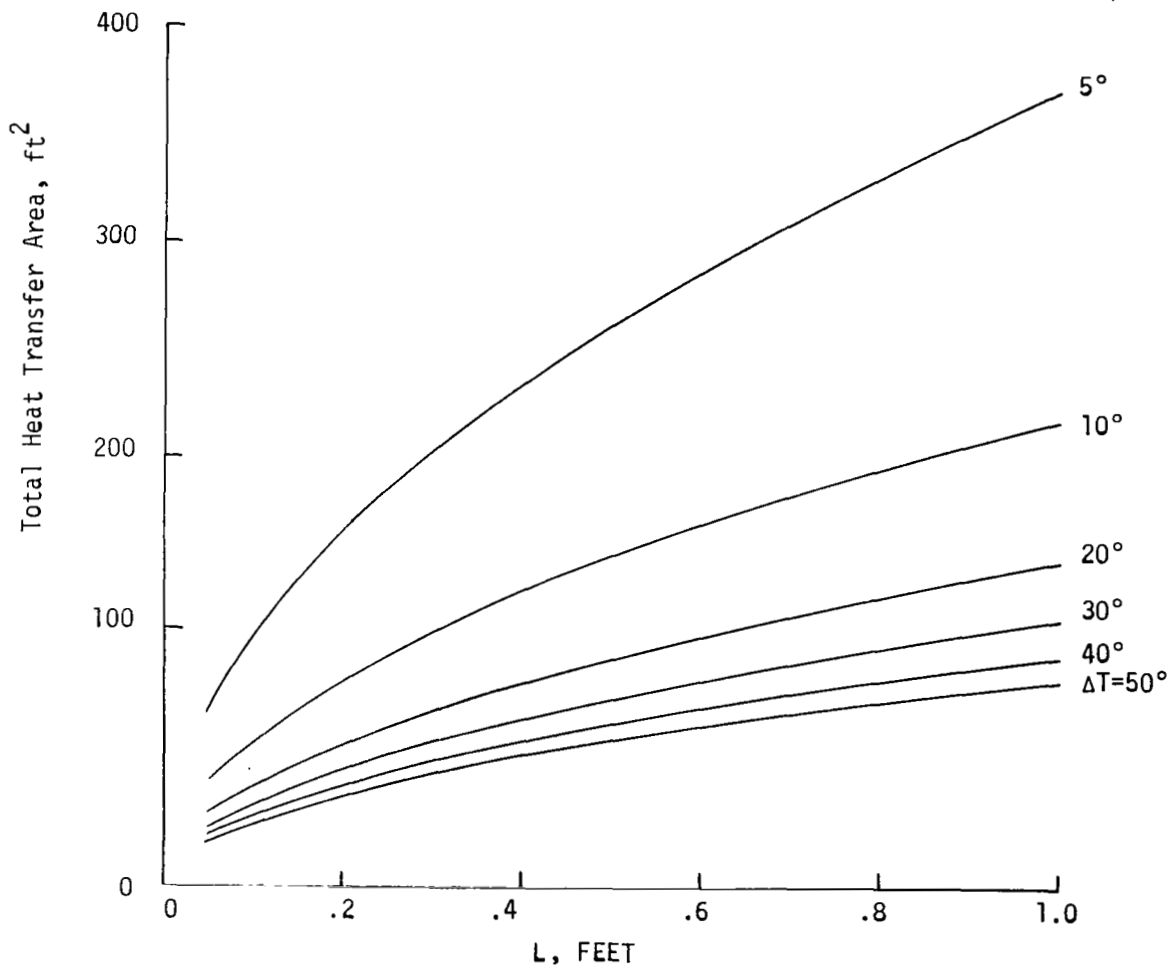
FIGURE A-4. CAPILLARY PUMP HEAT TRANSFER AREA VERSUS L FOR VARIOUS TEMPERATURE DIFFERENCES (TUNGSTEN FINS)
