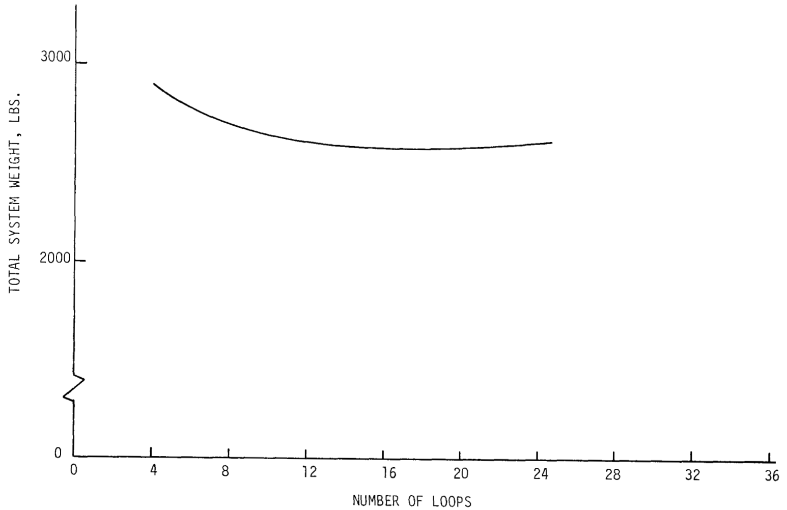
FIGURE 5-3. TOTAL HEAT REJECTION SYSTEM WEIGHT VERSUS NUMBER OF LOOPS
