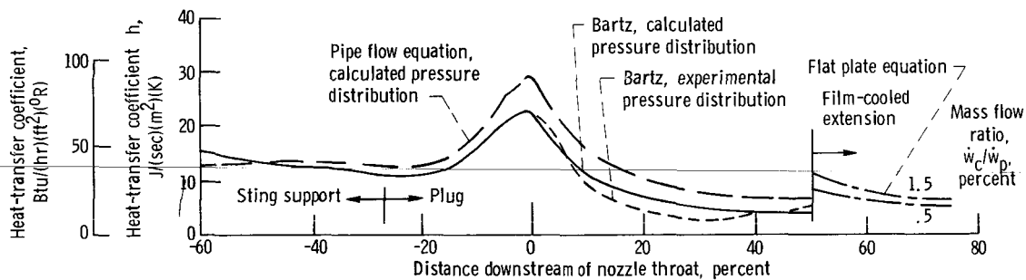
Figure 17. - Comparison of heat-transfer coefficients. Supersonic cruise; primary total temperature, 1345 K (2425° R); Mach 2.7; coolant total temperature, 533 K (960° R).
