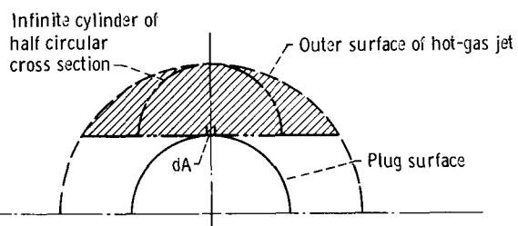
(c) Assumed hot-gas infinite cylinder of half cross section geometry (section A-A).
