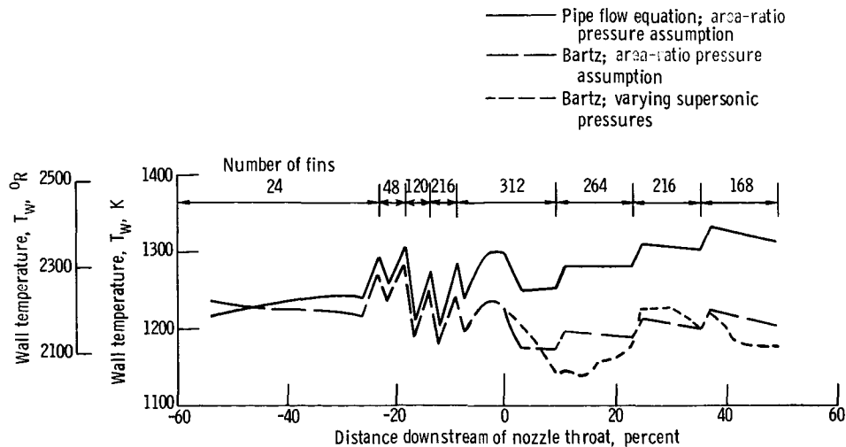
Figure 9. - Effect of heat-transfer coefficient on wall temperature. Sea-level takeoff; maximum afterburning; primary static temperature, 1945 K (3500° R); 2 percent coolant from compressor discharge.
