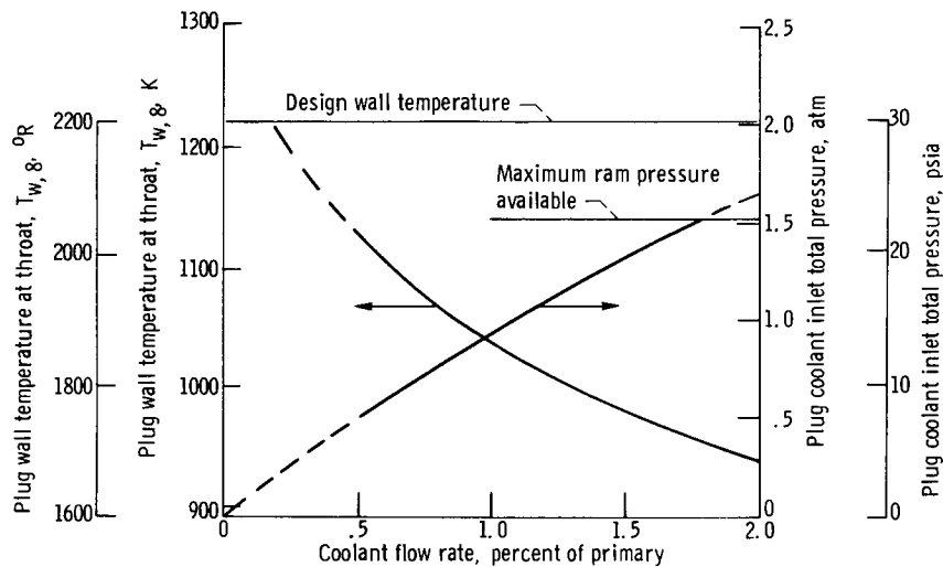
Figure 18. - Effect of coolant flow rate on plug throat wall temperature and required coolant inlet pressure. Supersonic cruise point; primary total temperature, 1345 K (2425 o R). Mach 2.7; ram cooling air; coolant total temperature, 533 K (960 o R).
