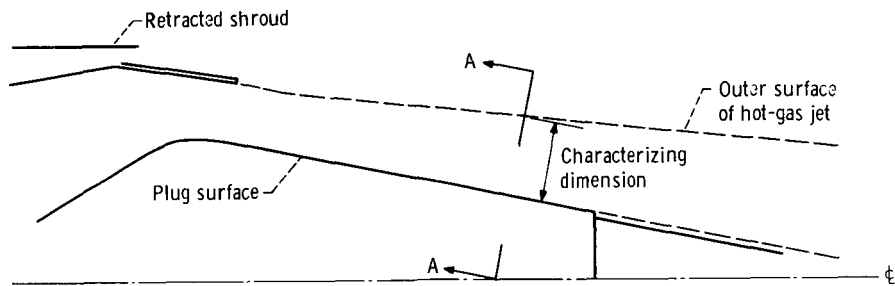
(a) Hot-gas jet geometry.
