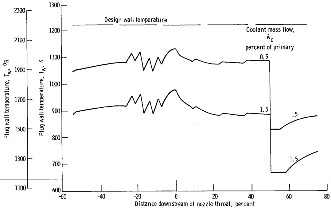
Figure 19. - Wall temperatures at supersonic cruise. Primary total temperature, 1345 K (2425 o R); Mach 2.7; ram air coolant; pipe flow equation.
