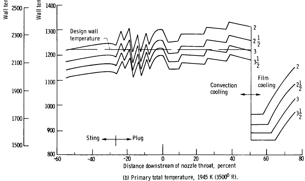
Figure 10. - Effect of coolant flow rate on plug wall temperature. Sea-level takeoff; Mach 0; pipe flow equation (compressor exit coolant); coolant inlet temperature, 667 K (1200 ^{\circ} R); emissivity, 0.65.
