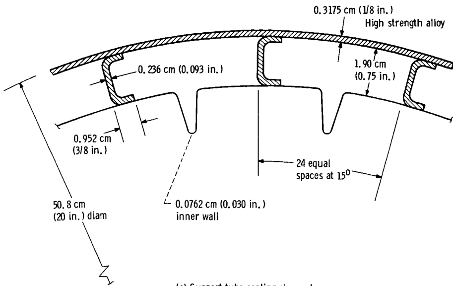
(a) Support tube cooling channels.
