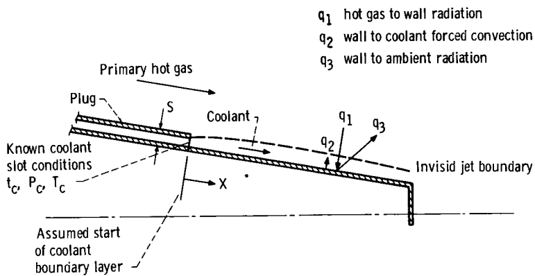
(b) Film cooling ( q_1 = q_2 + q_3 ).
