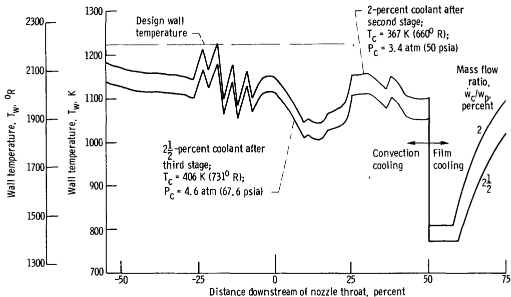
Figure 15. - Resulting wall temperatures using compressor interstage bleed. Sea-level takeoff; maximum afterburning, primary total temperature, 1945 K (3500 ^{\circ} R).
