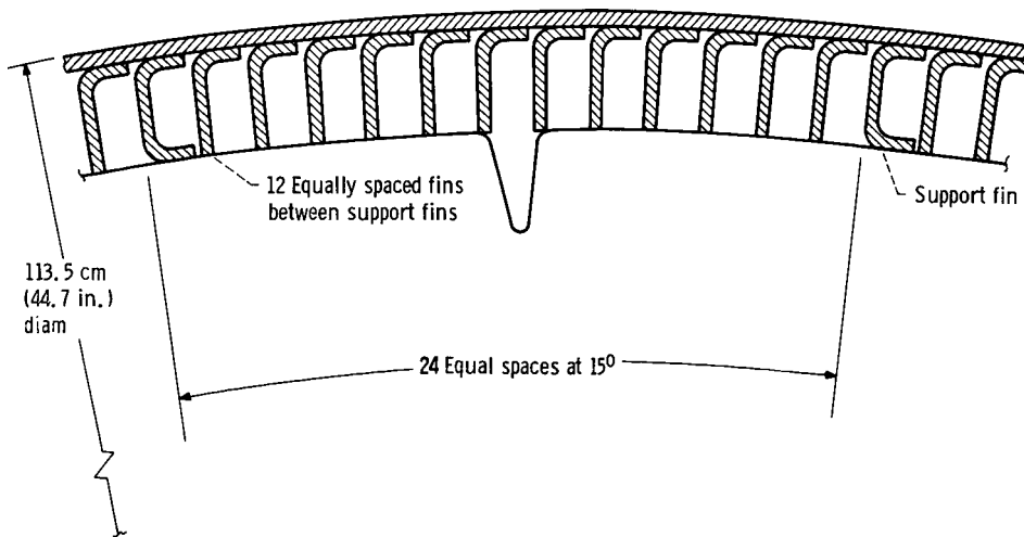
(b) Cooling channels at maximum plug diameter.
