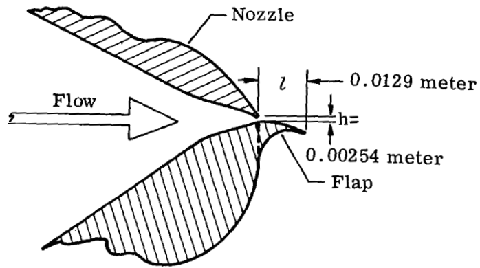
(a) Short internally blown flap.
