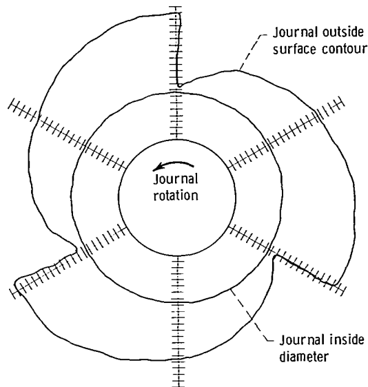
Figure 2. - Circumferential surface profile trace of journal 8. Scale, 0.013 millimeter (500 \mu n.) per division.
