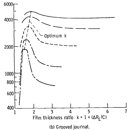
Figure 8. - Whirl onset speed as function of film thickness ratio.
