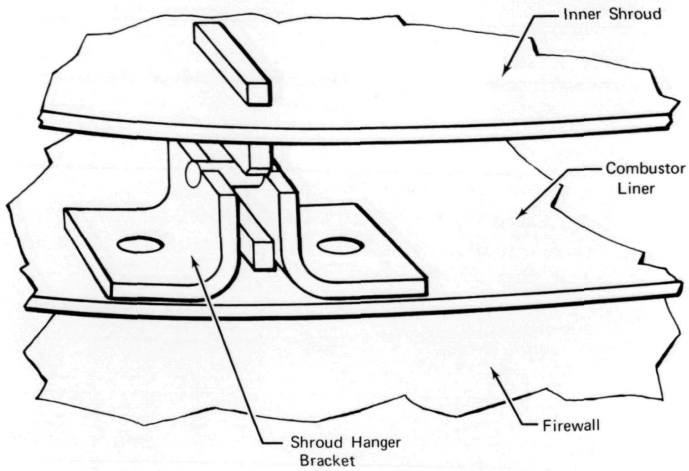
Figure 18. Shroud Hanger Bracket
