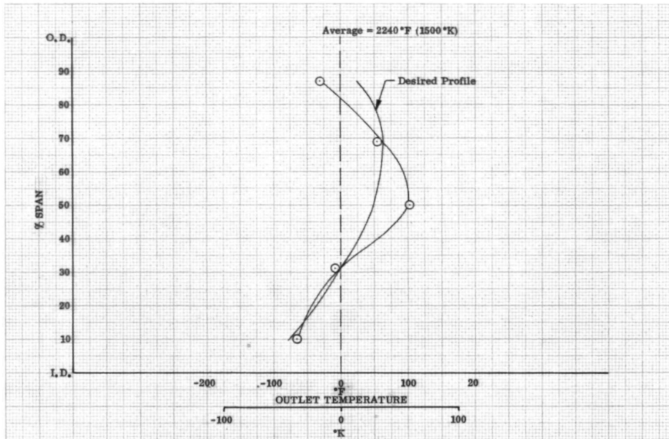
Figure 12. Outlet Radial Temperature Profile; DF 88196 Model 8 Combustor Installed in 7-deg (0.122-rad) ECA Diffuser
