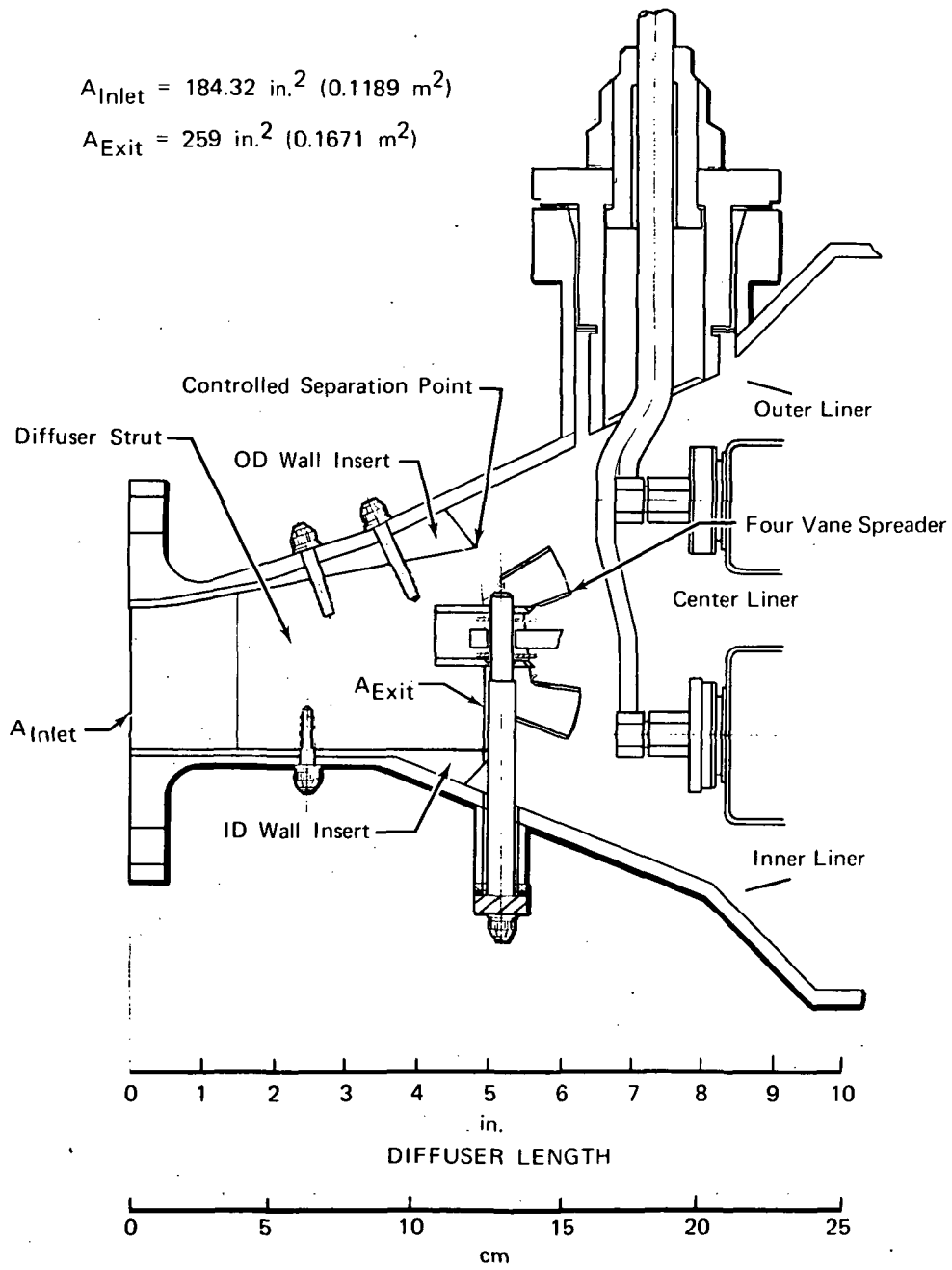
Figure 3. 9-deg (0.157-rad) ECA Dump Diffuser FD 56940A
