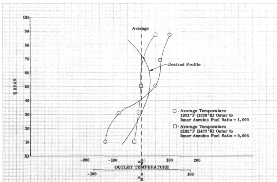
Figure 15. Outlet Radial Temperature Profile; DF 88199 Model 8 Combustor Installed in 14-deg (0.244-rad) Diffuser
