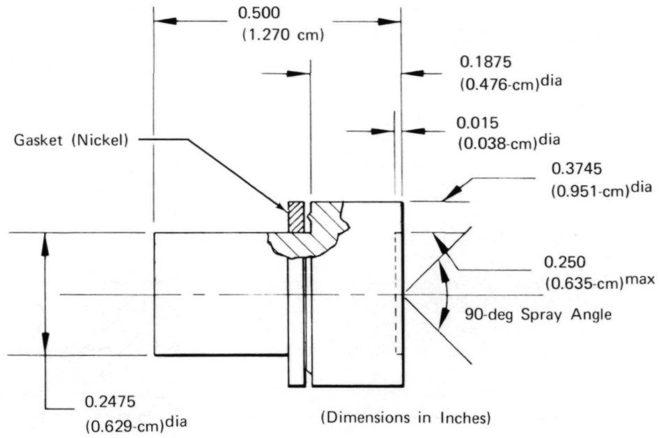
Figure 4. Fuel Nozzle
