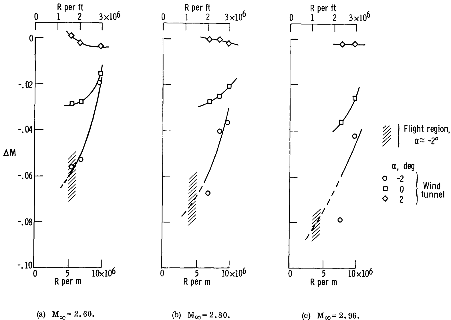
Figure 12. Variation of Mach number position error for the compensated probe with Mach number, Reynolds number, and angle of attack.
