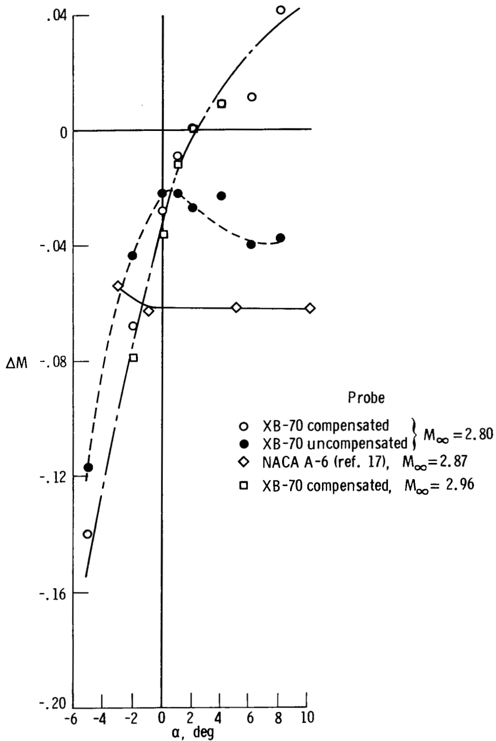
Figure 15. Effect of angle of attack on the Mach number position error for three types of pitot-static airspeed probes as obtained from Langley wind-tunnel calibrations.
