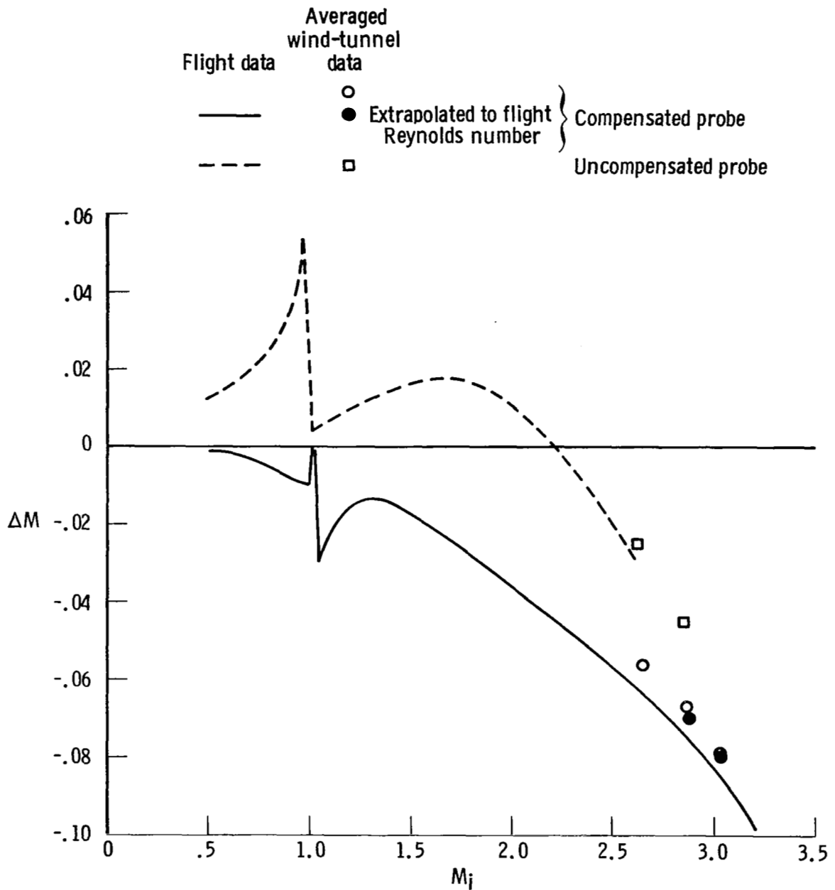
(a) Variation of Mach number position error with indicated Mach number.
