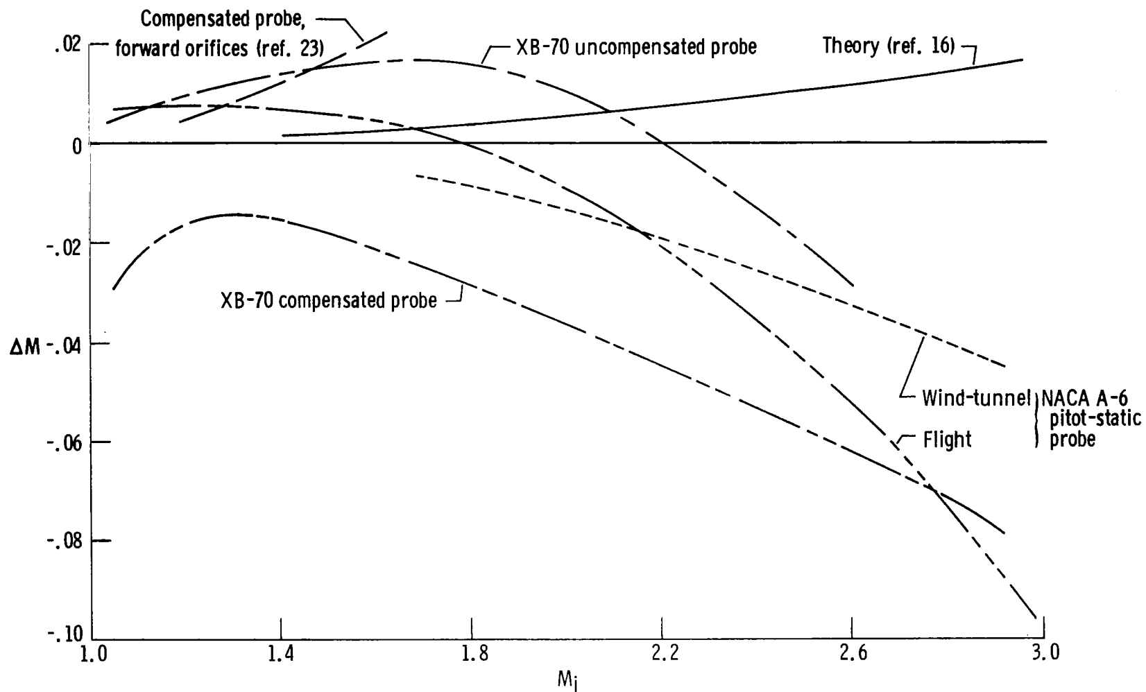
Figure 20. Comparison of supersonic position errors obtained from theory, wind-tunnel tests, and flight data for several types of nose-boom-mounted pitot-static airspeed probes.
