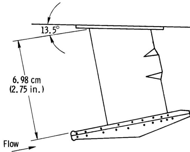
(b) Sketch of probe showing dimensions.
