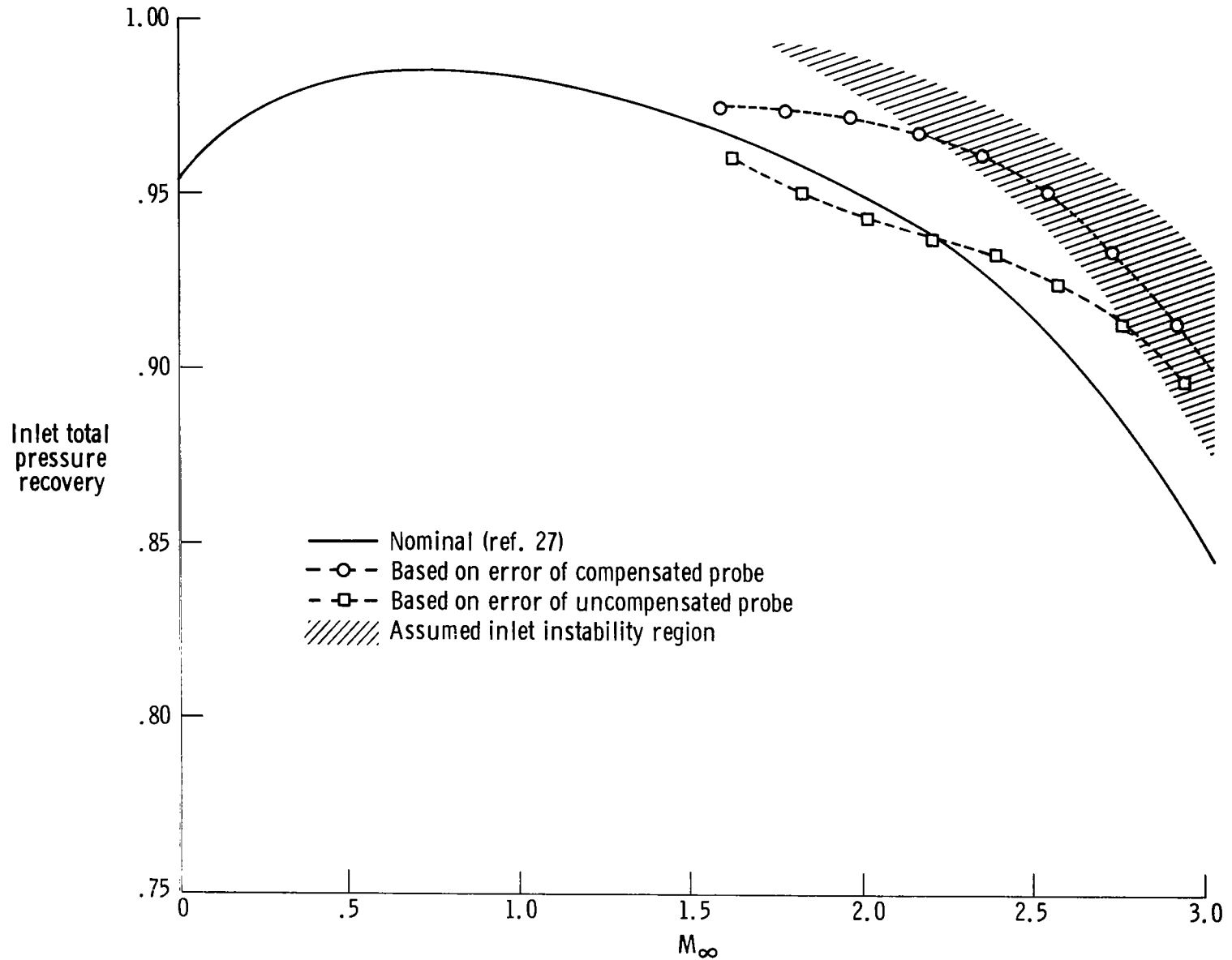
Figure 21. Effects of airspeed probe position error for the S_1/S_2 configuration in establishing supersonic inlet pressure recovery.
