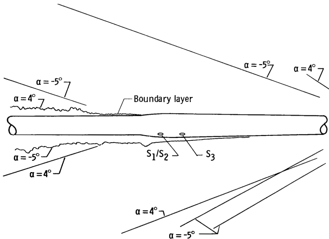
(b) Laminar boundary layer over static ports. R per meter = 4.862 \times 10^6 ( R per foot = 1.482 \times 10^6 ).
