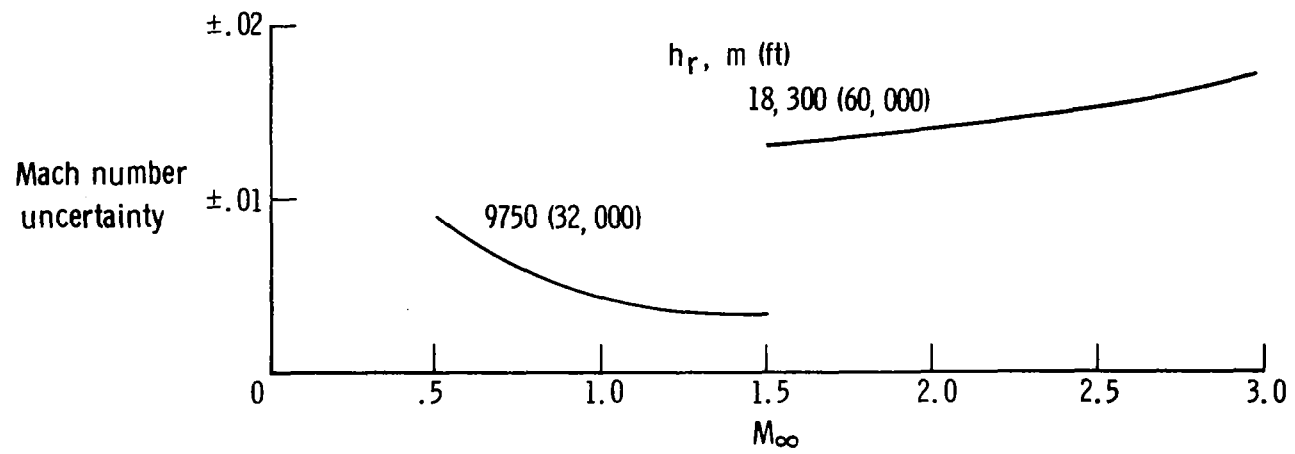
Figure 8. Uncertainties in Mach number and altitude resulting from inaccuracies in the airspeed pressure transducers used on the XB-70 airplane.
