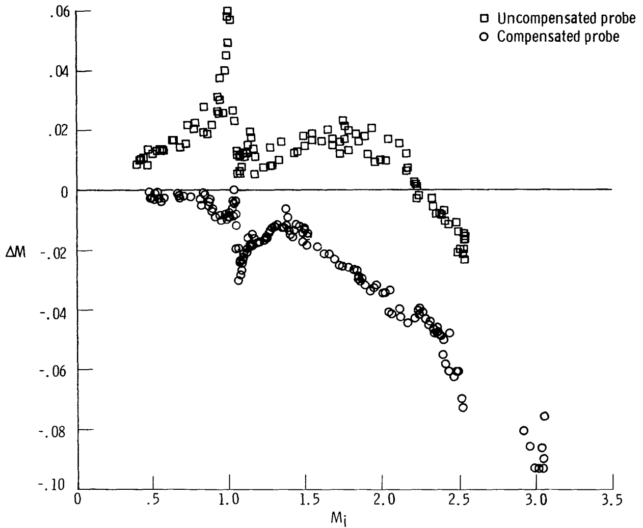
Figure 13. Variation of Mach number position error with Mach number for the two pitot-static probes used on the XB-70. S_1/S_2 configuration.
