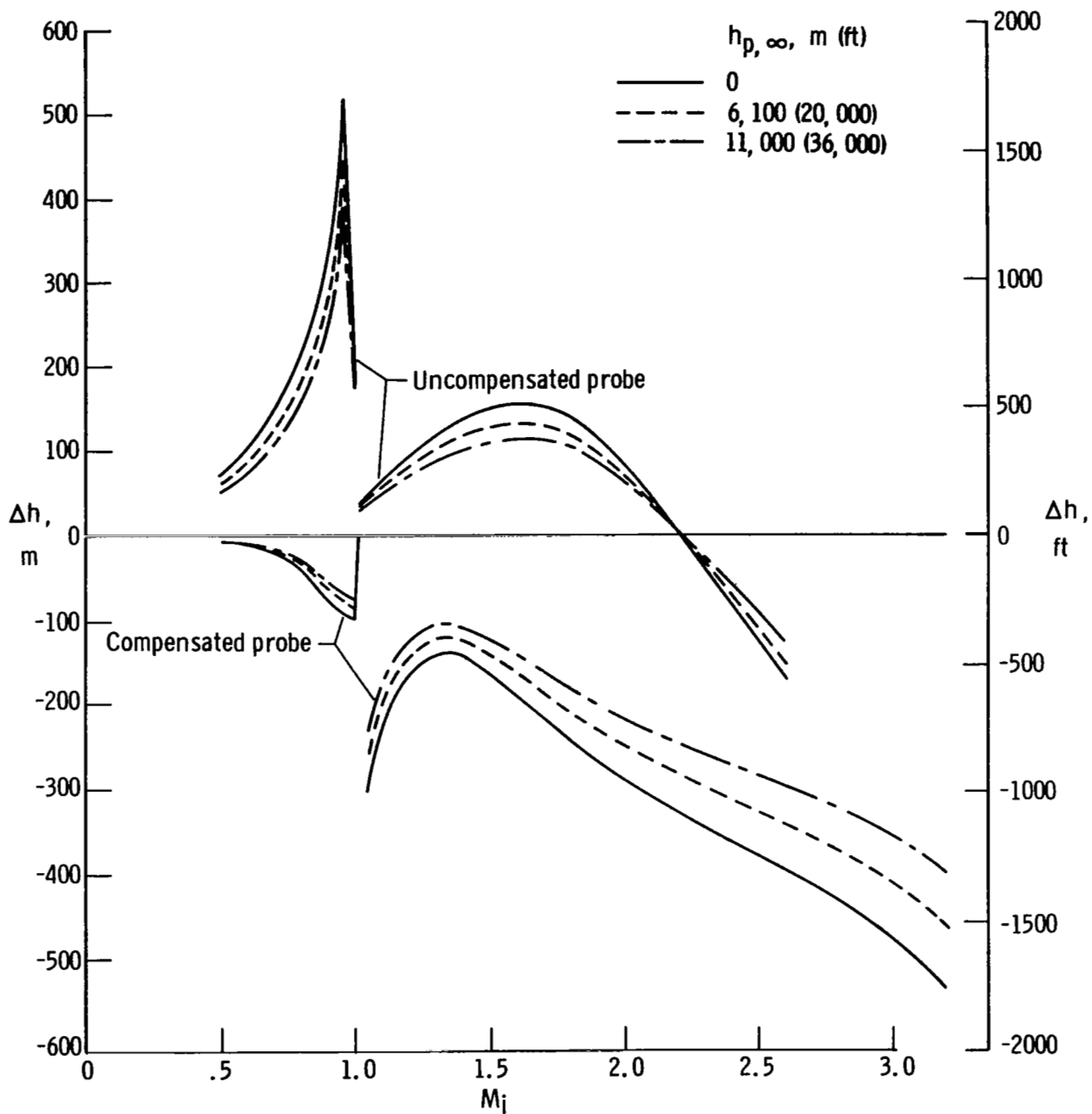
(c) Variation of pressure-altitude position error with indicated Mach number.
