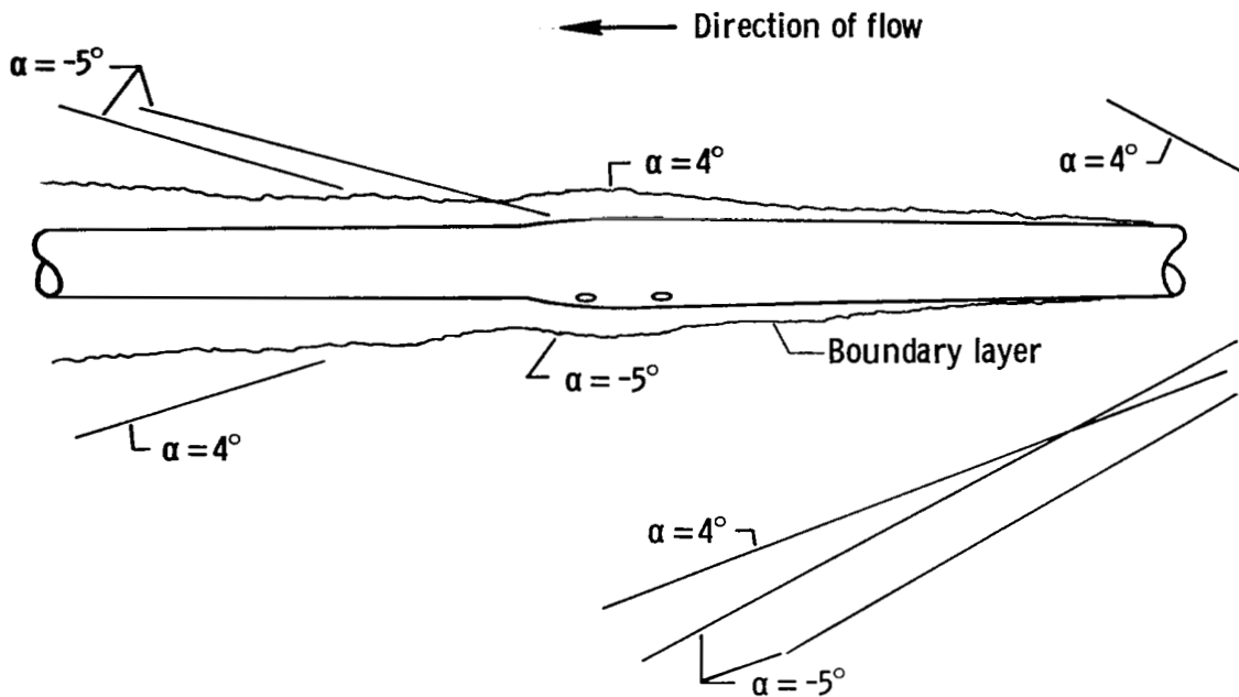
(a) Turbulent boundary layer over static ports. R per meter = 13.1 \times 10^6 ( R per foot = 4 \times 10^6 ).
