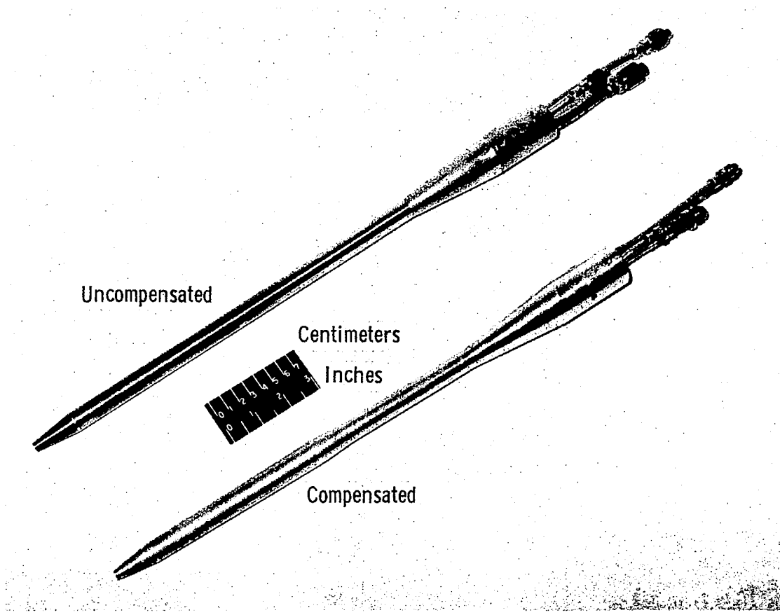
Figure 2. XB-70 compensated and uncompensated pitot-static (airspeed) probes.
