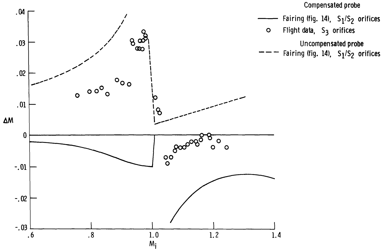
Figure 19. Comparison of position errors for the S_3 orifices on the compensated pitot-static probe with those for the S_1/S_2 orifices on the compensated and uncompensated pitot-static probes.
