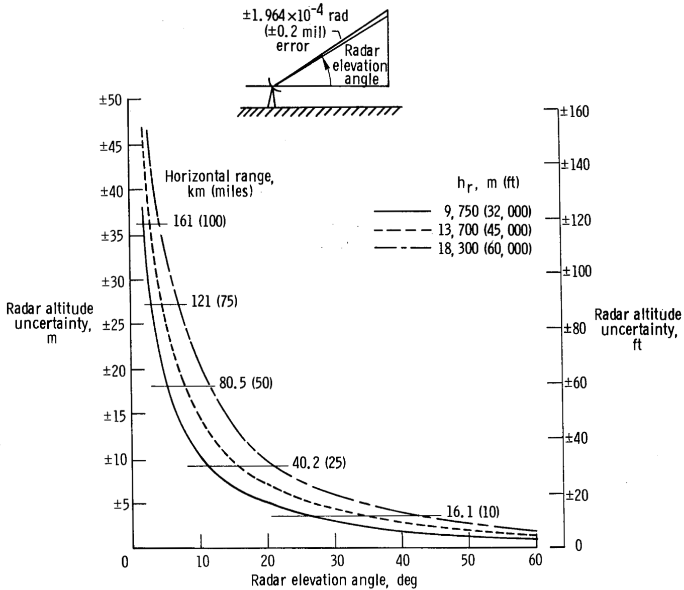
Figure 9. Effect of \pm 1.964 \times 10^{-4} -radian ( \pm 0.2 -mil) error in radar elevation angle on radar altitude uncertainty.
