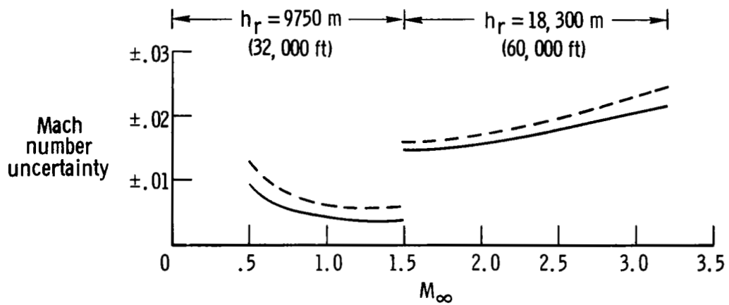
Figure 10. Effect of reference pressure error on the uncertainties in Mach number and altitude measurements.
