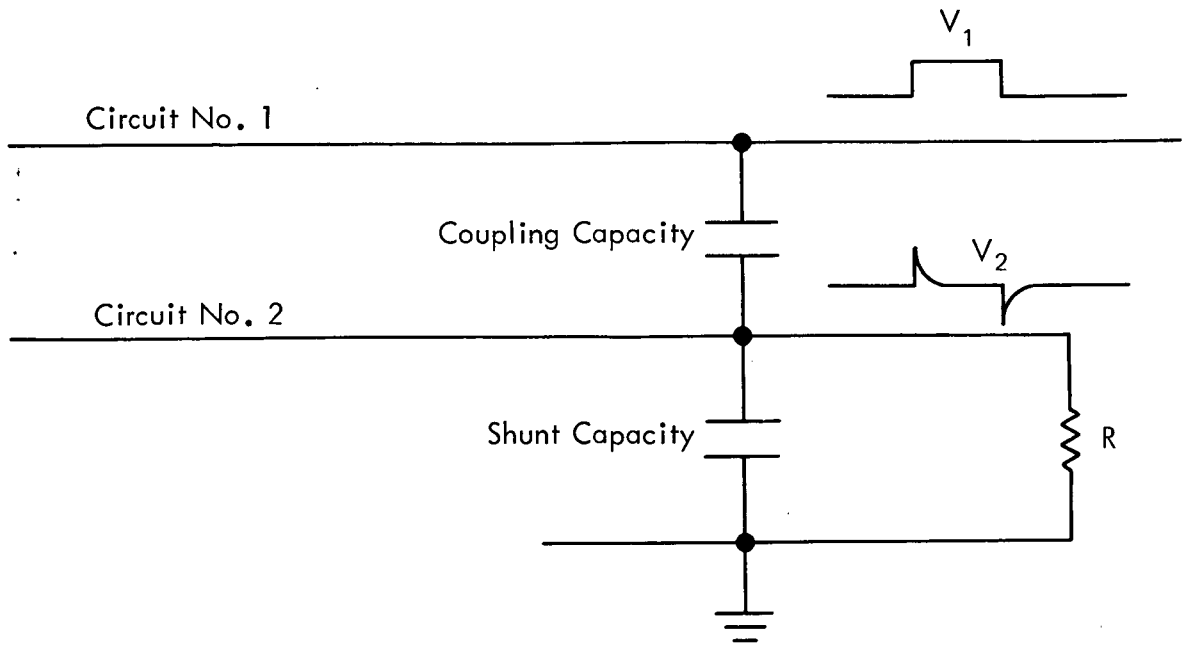
Figure 4. - Capacitive coupling.
