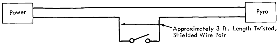
Figure 1. - Block diagram of pyro-power configuration.
