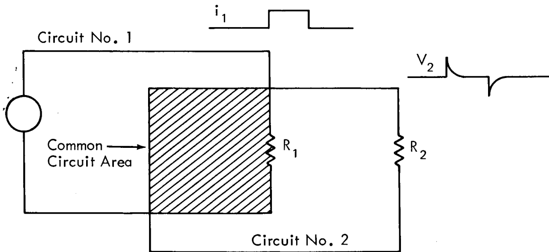
Figure 5. - Inductive coupling.
