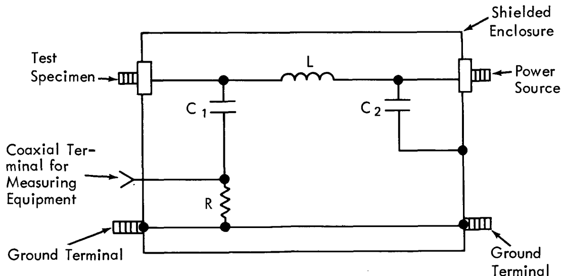
Figure 6. - Line impedance stabilization network.
