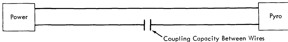
Figure 2. - Equivalent circuit of pyro-power configuration.
