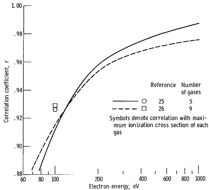
Figure 8. - Variation in coefficient of correlation of sensitivity with ionization cross section at various electron energies for Alphasatron gage.
