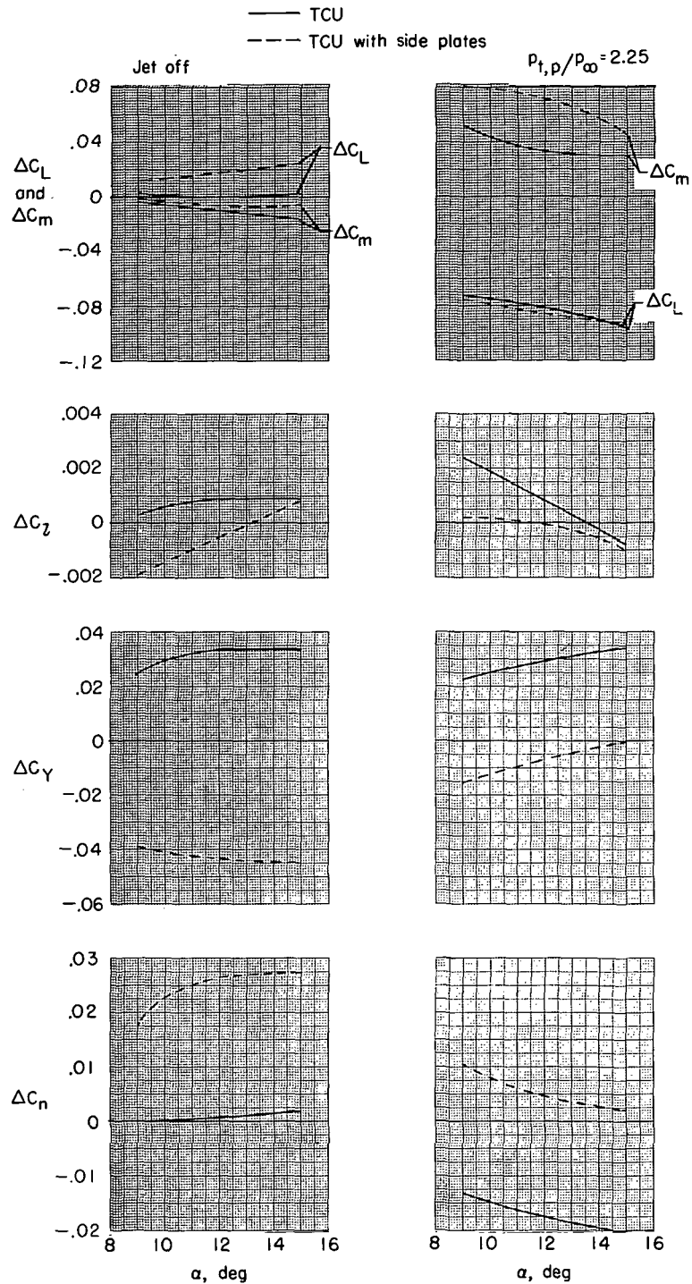
(a) M = 0.23 ; \beta = 10^\circ ; \delta_f = -30^\circ ; \delta_s = -20^\circ ; \delta_h = -10^\circ ; \delta_b = 75 percent.
