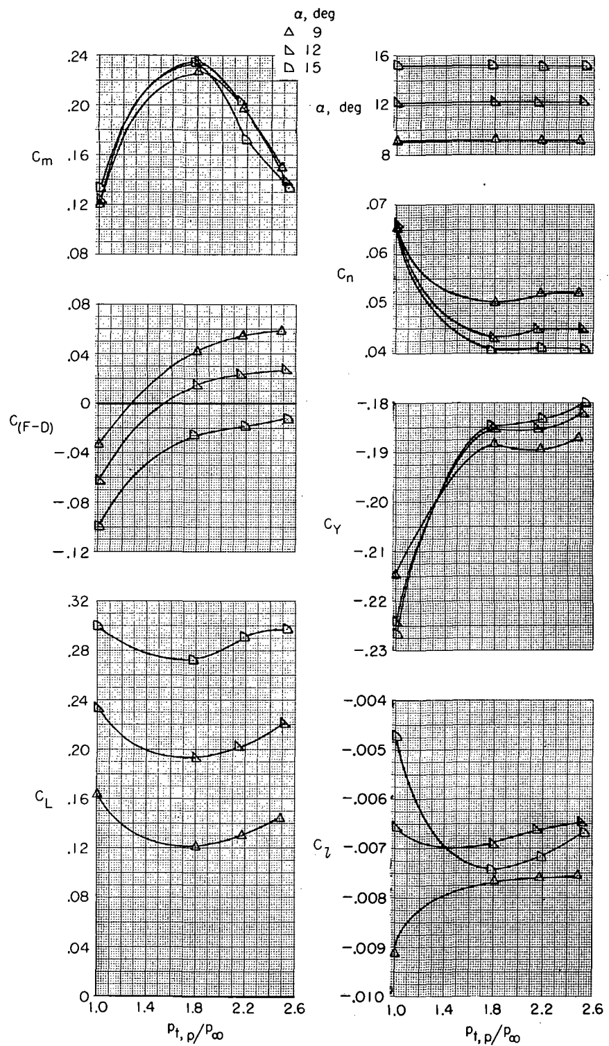
(q) \beta = 10^\circ ; \delta_b = 75 percent; \delta_h = -10^\circ ; \delta_r = -15^\circ ; \delta_{du} with side plates.
