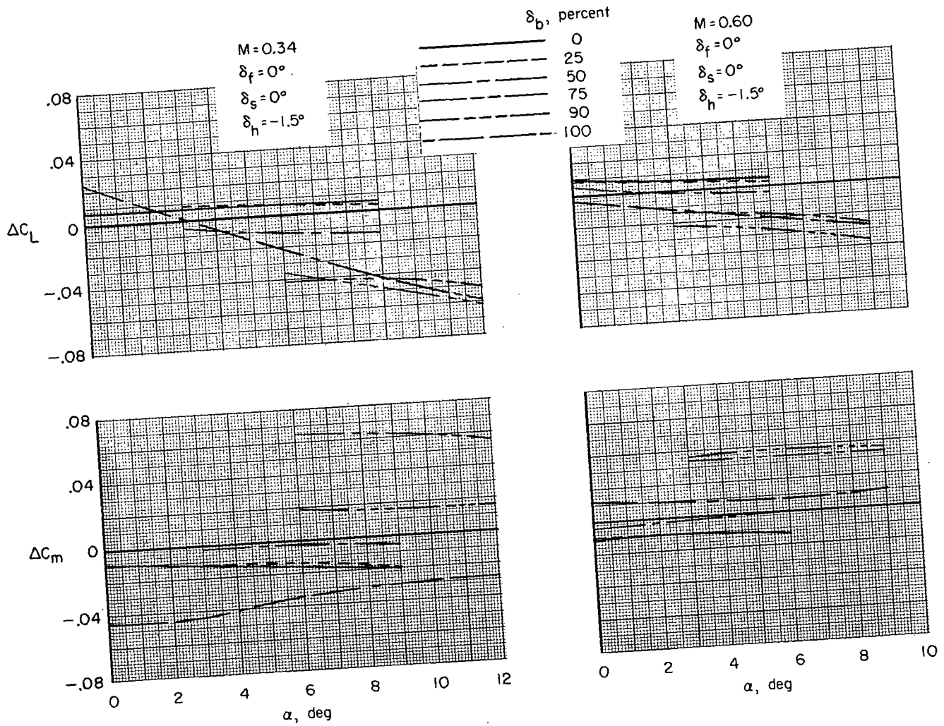
(b) M = 0.34 and 0.60 . Figure 45.- Continued.
