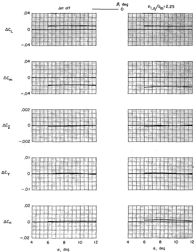
(a) M = 0.23 ; \delta_f = -30^\circ ; \delta_s = -20^\circ ; \delta_h = -10^\circ ; \delta_p = 0 percent.
