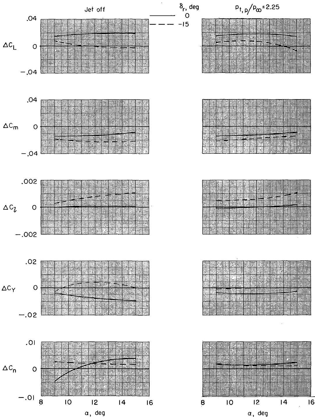
(a) M = 0.23 ; \beta = 10^\circ ; \delta_f = -30^\circ ; \delta_s = -20^\circ ; \delta_h = -10^\circ .
