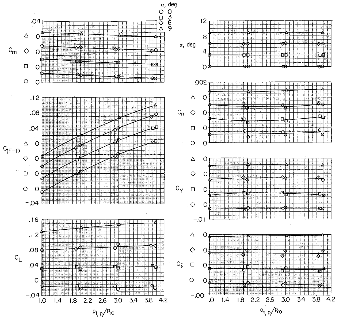
(c) M = 0.60 ; military power.
