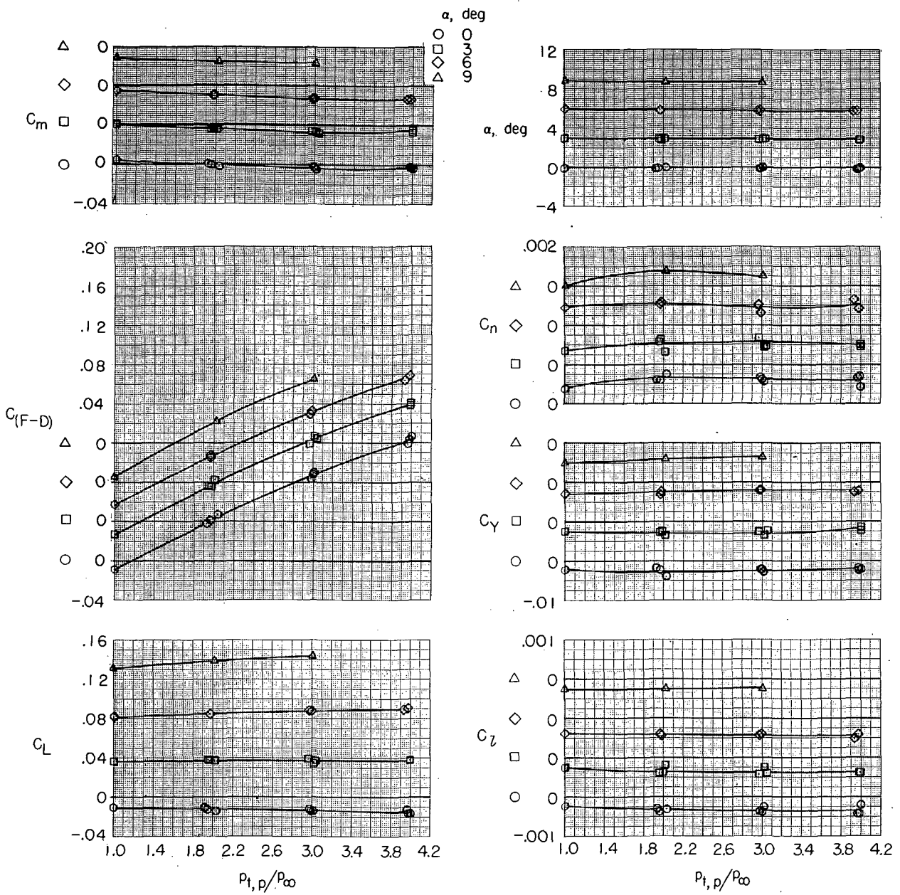
(c) M = 0.60 ; military power.
