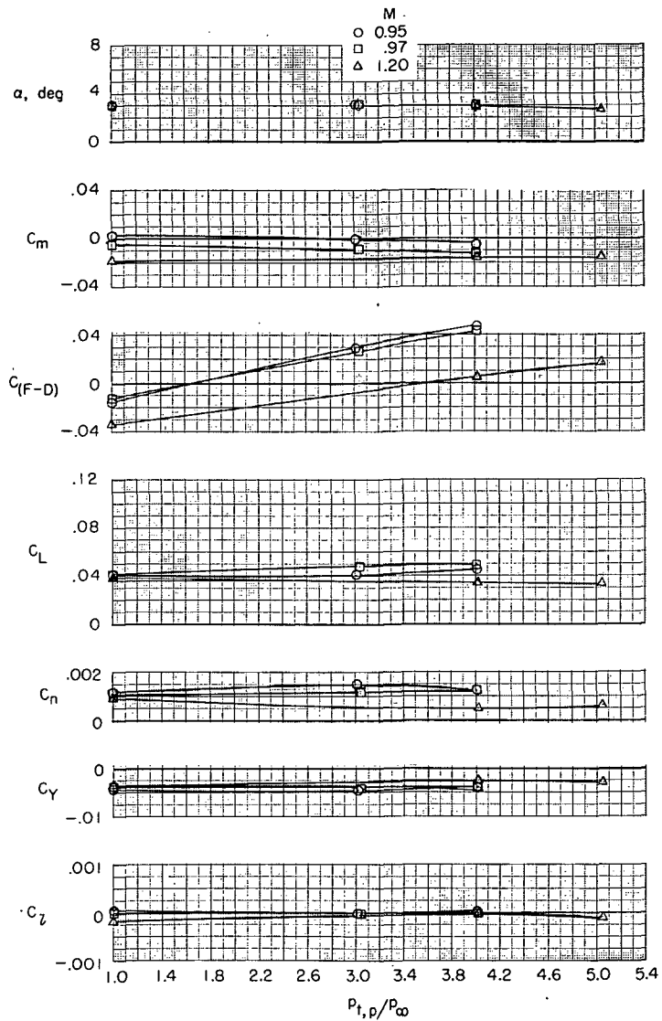
(e) M = 0.95 to 1.20 ; military power.
