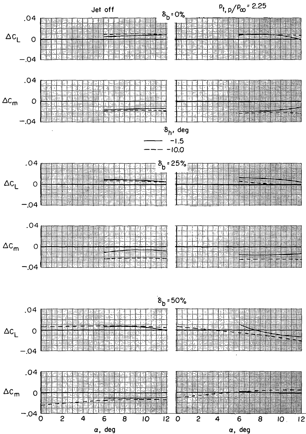
(a) M = 0.23 ; \delta_f = -30^\circ ; \delta_s = -20^\circ .
