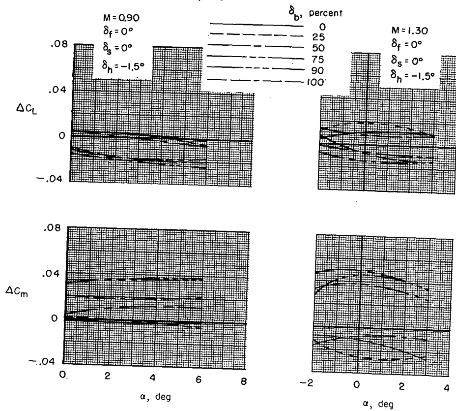
(c) M = 0.90 and 1.30 .
