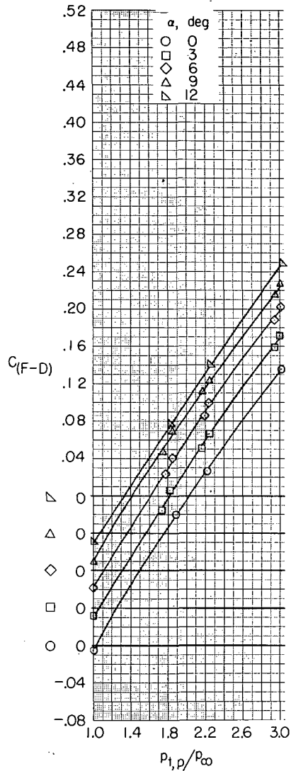
(b) M = 0.35 ; military power.
