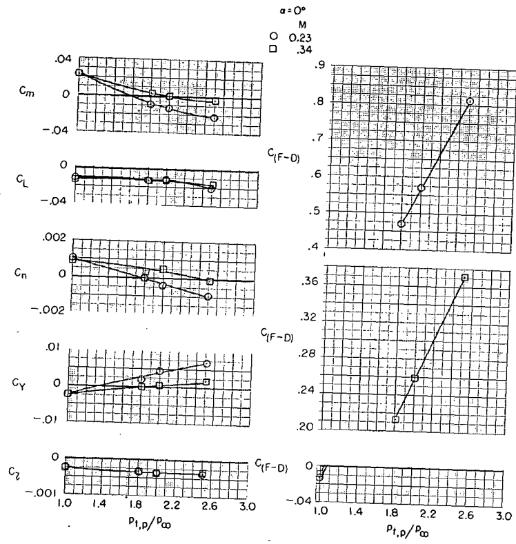
(g) M = 0.23 and 0.34 ; afterburning power.
