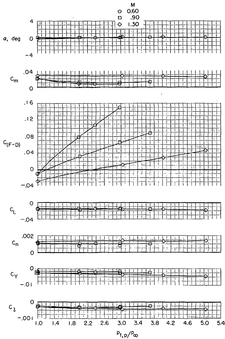
(h) M = 0.60, 0.90, \text{ and } 1.30 ; afterburning power.
