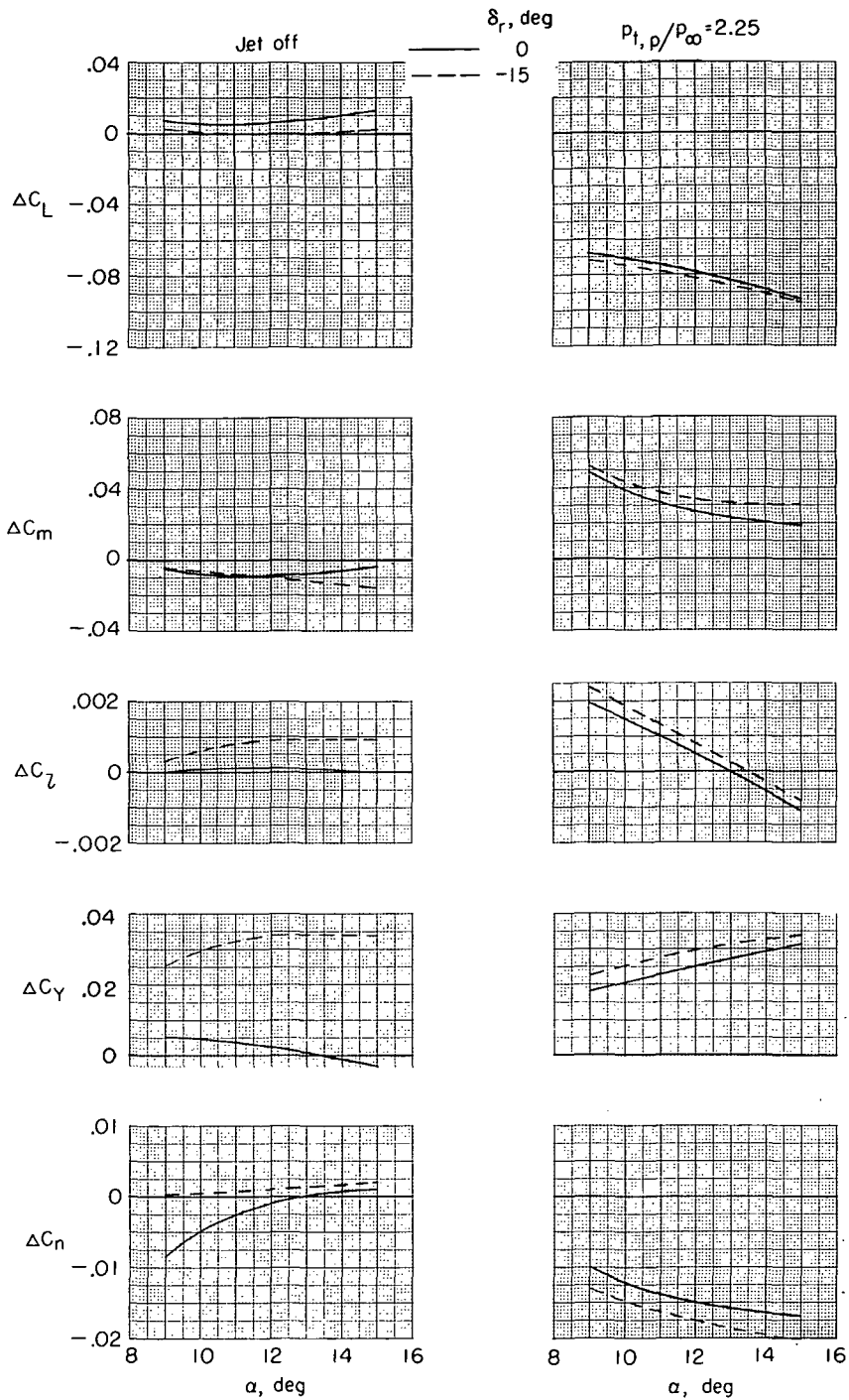
(a) M = 0.23 ; \beta = 10^\circ ; \delta_f = -30^\circ ; \delta_s = -20^\circ ; \delta_h = -10^\circ ; \delta_b = 75 percent.
