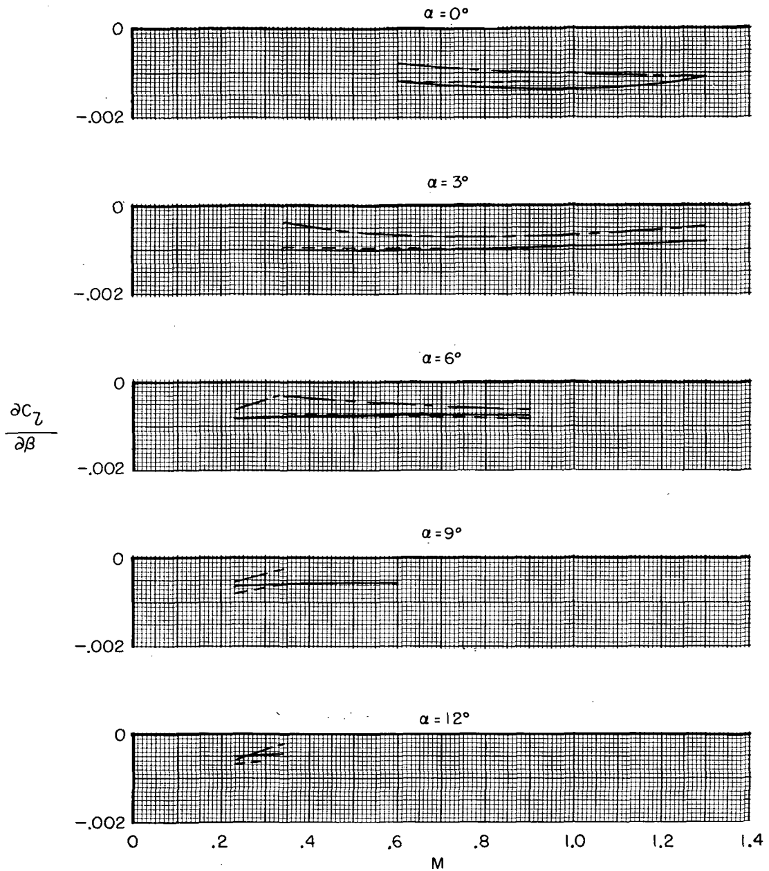
(b) Rolling-moment derivative.
