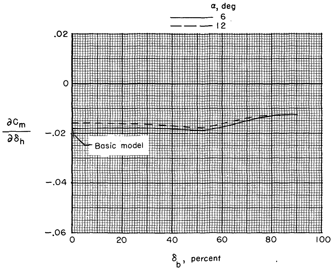
Figure 49.- Effect of blocker-door closure on stabilizer effectiveness. M = 0.23 ; \beta = 0^\circ ; \delta_f = -30^\circ ; \delta_s = -20^\circ ; \delta_r = 0^\circ ; \delta_{du} = 32.5^\circ ; \delta_{dl} = 52.5^\circ ; and military power.
