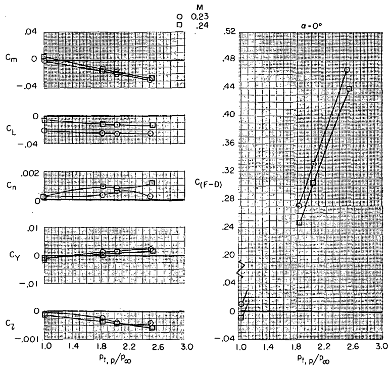
(a) M = 0.23 and 0.24 ; military power.
