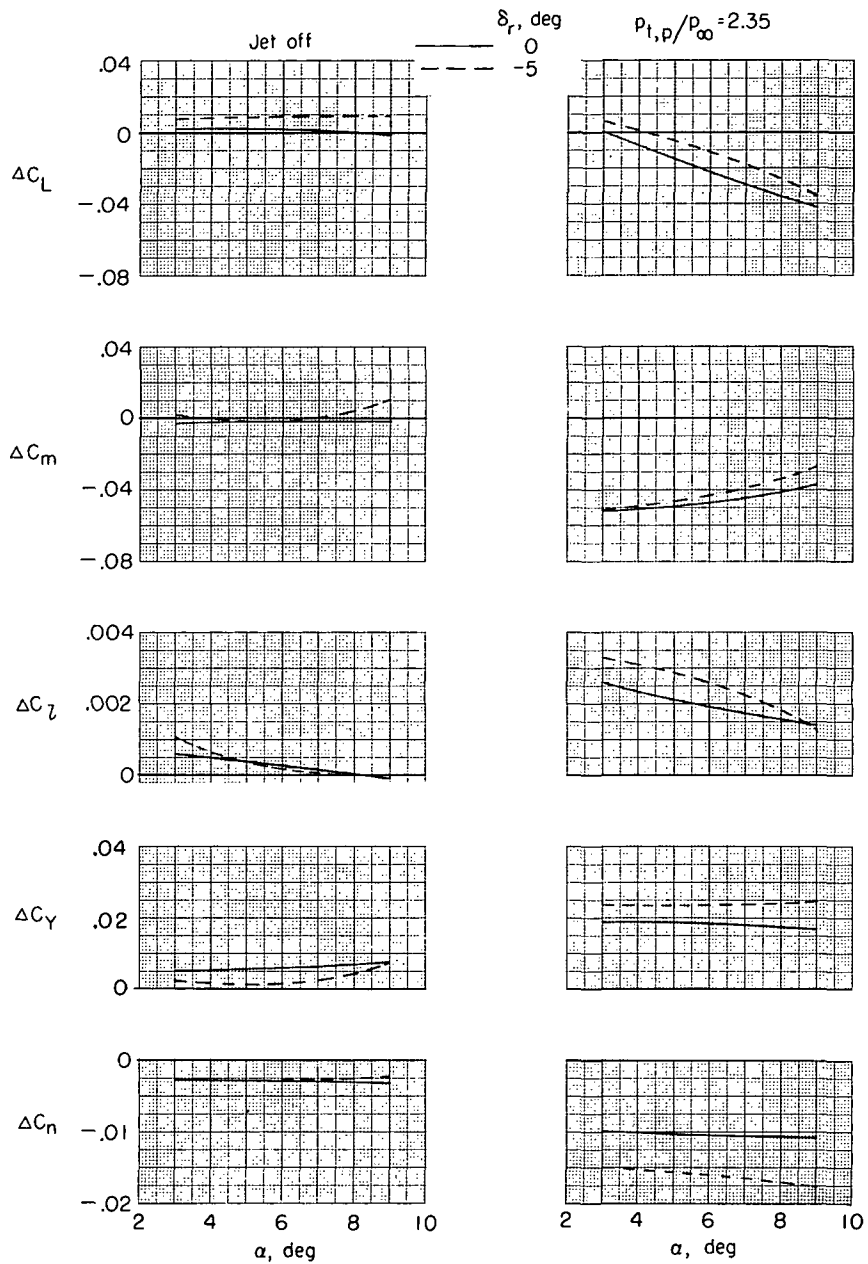
(c) M = 0.34 ; \beta = 5^\circ ; \delta_f = 0^\circ ; \delta_s = 0^\circ ; \delta_h = -1.5^\circ ; \delta_b = 100 percent.
