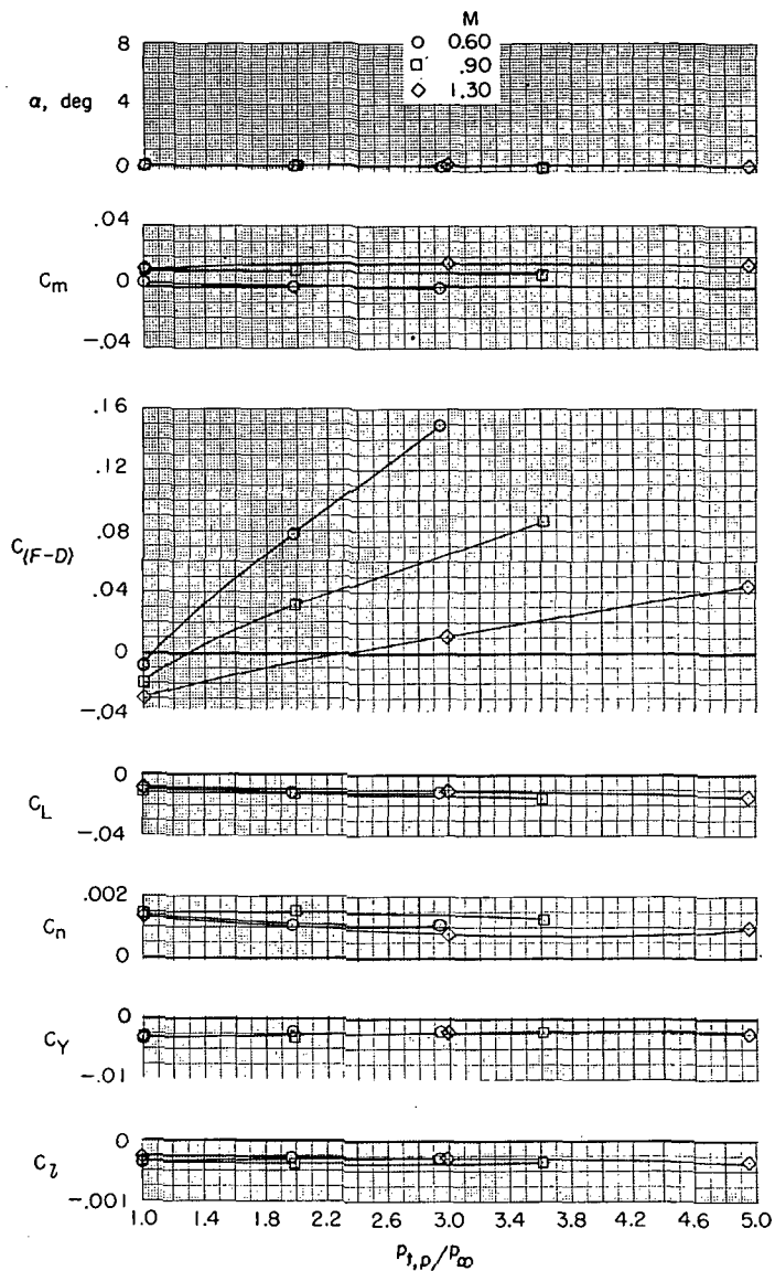
(g) M = 0.60, 0.90, \text{ and } 1.30 ; afterburning power.
