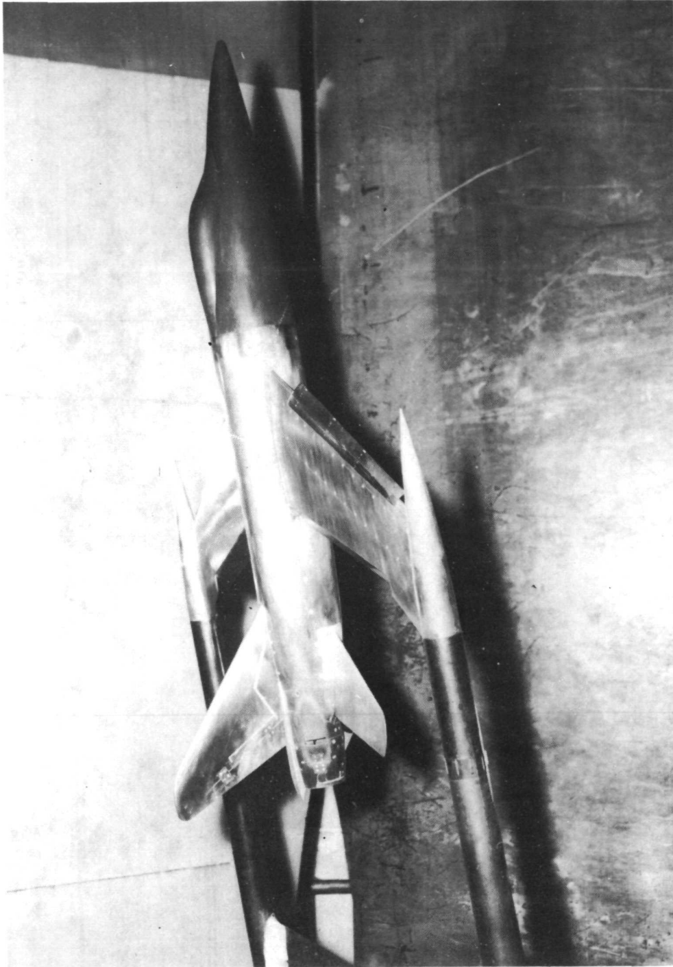
(a) Approach configuration with thrust control unit deployed.
