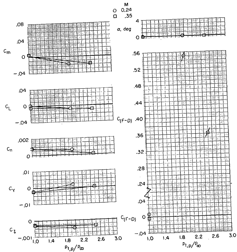
(f) M = 0.24 and 0.35 ; afterburning power.
