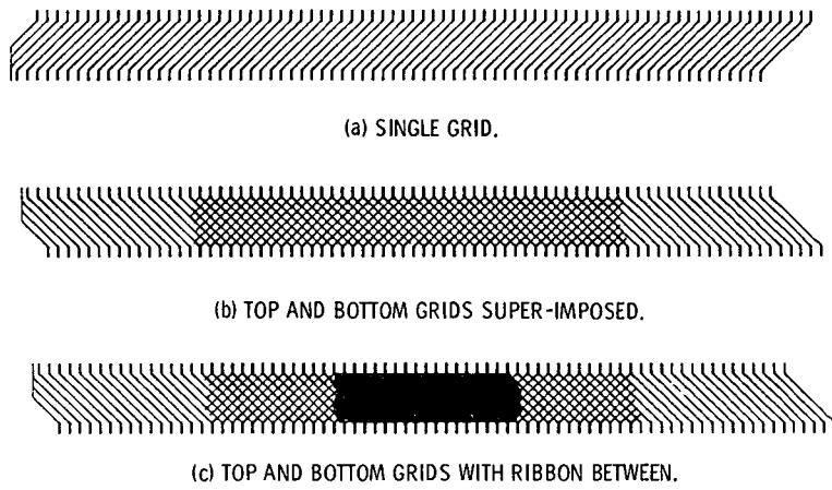
Figure 3. - Photographic film masks used with photoresist process.
