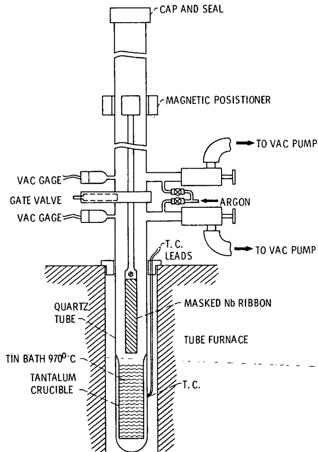
Figure 4. - Nb_3Sn diffusion reaction apparatus.
