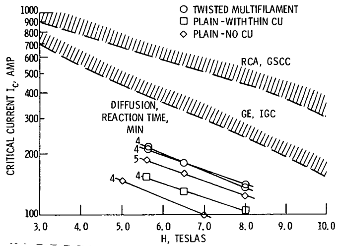
Figure 6. - I_c vs H for 1.27 cm wide Nb 3 Sn ribbon.
