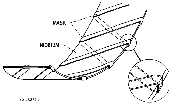
Figure 1. - Mask forming twisted path on Nb ribbon.
