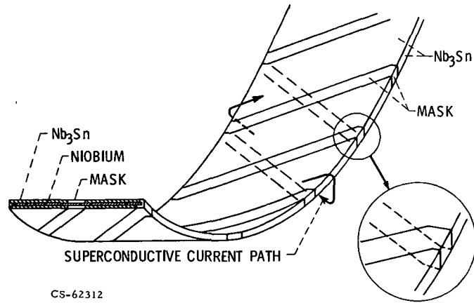
Figure 2. - Twisted filamentary Nb_3Sn ribbon.
