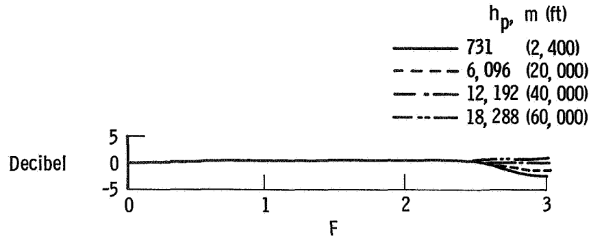
(b) Electrostatic altitude sensitivity response.
