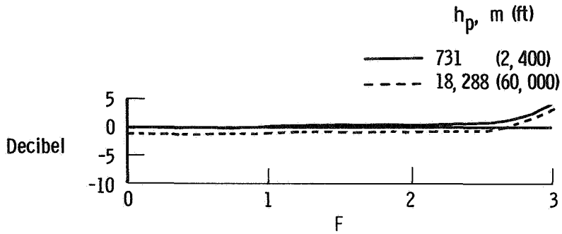
(b) Electrostatic altitude sensitivity response.
