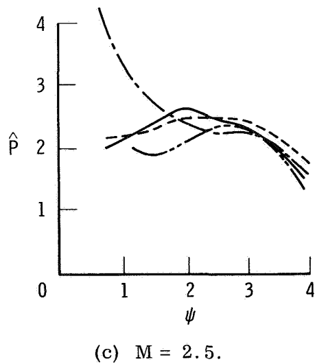
Figure 27. Comparison of the estimated power-spectral-density measurements from the AR, BBN, Kistler, and ES transducers. Data corrected to location 1.
