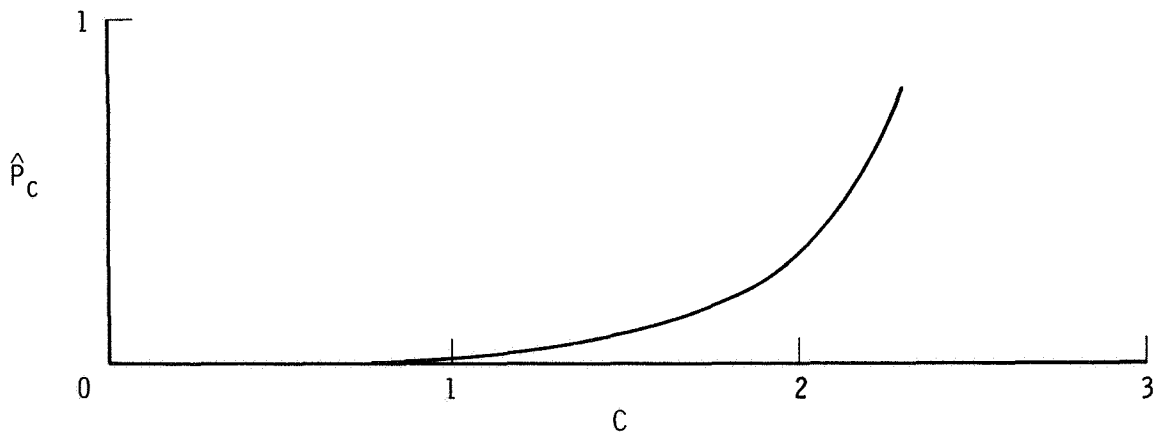
Figure 19. Corcos size correction to estimated power spectral density as a function of a nondimensional frequency parameter.
