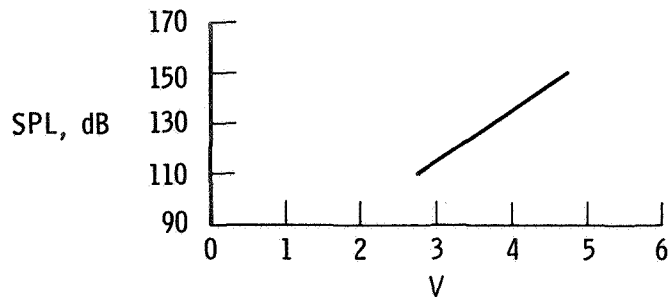
(a) Transducer sensitivity (-62 dB ref. 1 volt/N/m 2 ).
