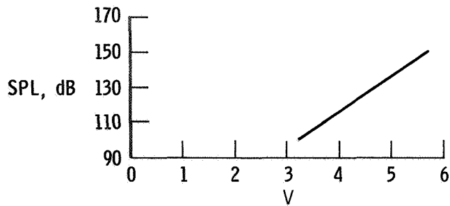
(a) Transducer sensitivity (-42 dB ref. 1 volt/N/m 2 ).
