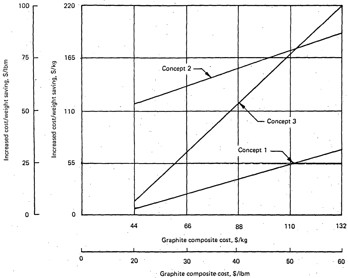
FIGURE 33.—EFFECT OF GRAPHITE COMPOSITE PRICE ON THE COST OF WEIGHT SAVING
