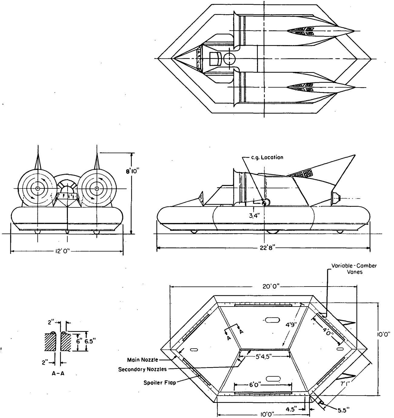
Figure 1.- Principal dimensions and general arrangement of GEM III.
