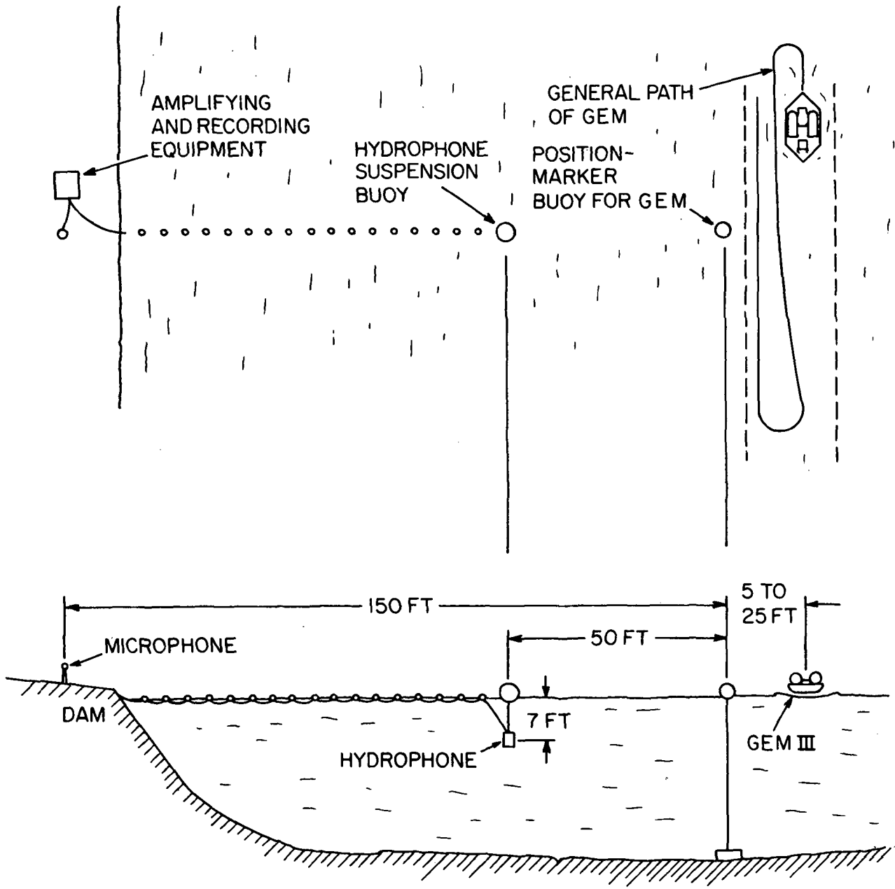
Figure 2.- Relative positions of microphone, hydrophone, and GEM.
