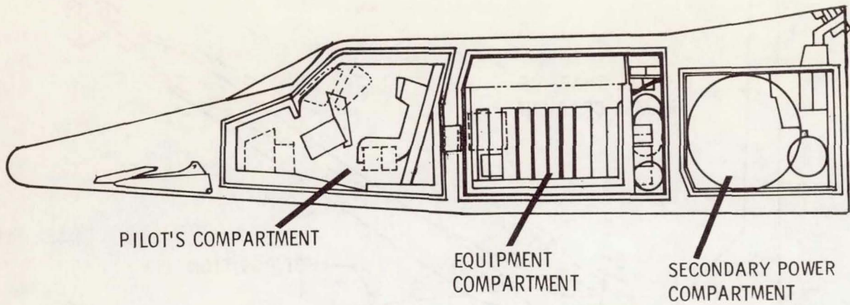
Figure 12. Inboard Profile
