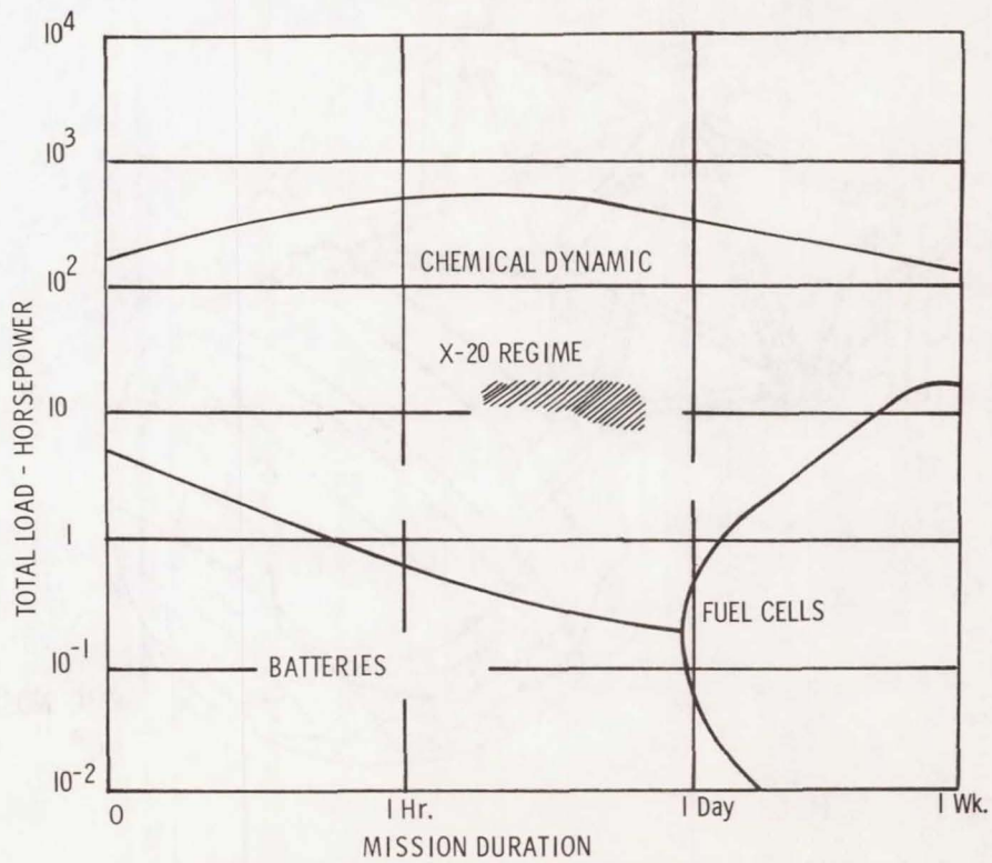
Figure 19. Source of Secondary Power Generation
