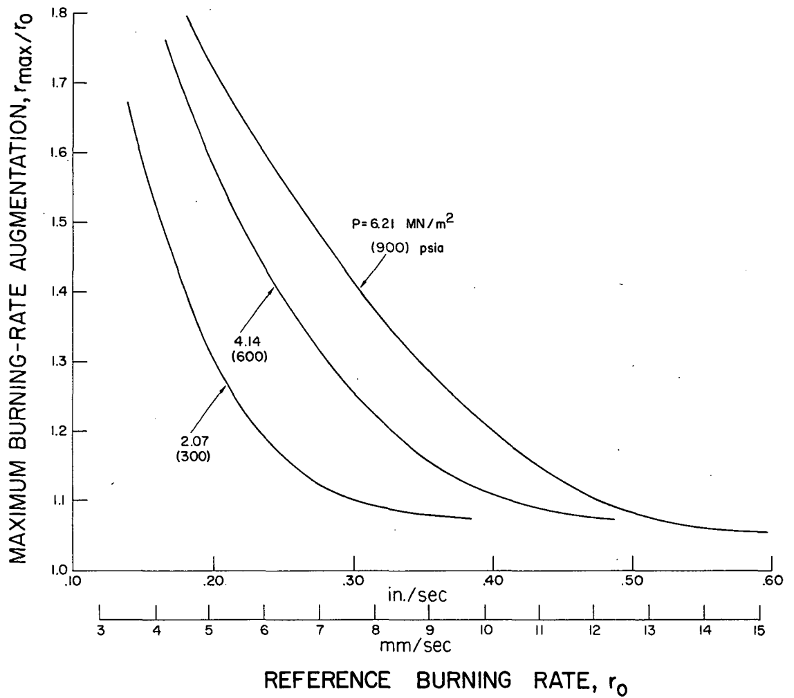
Figure 7.- Effect of pressure on maximum rate augmentation at 100g normal acceleration.
