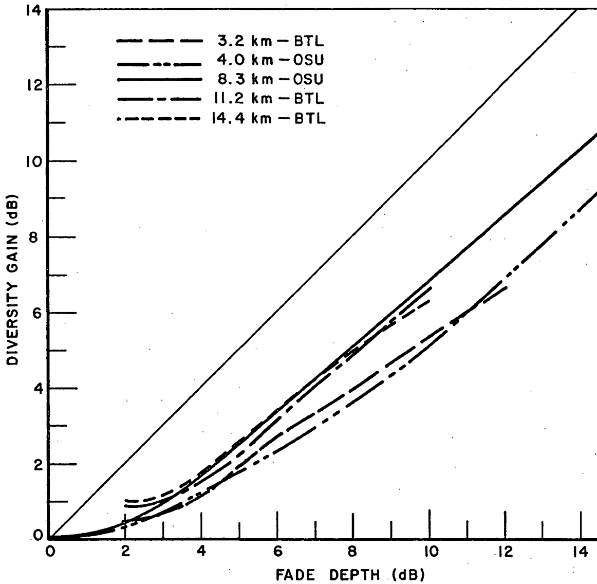
Fig. 7. Comparison of BTL and OSU diversity data.
