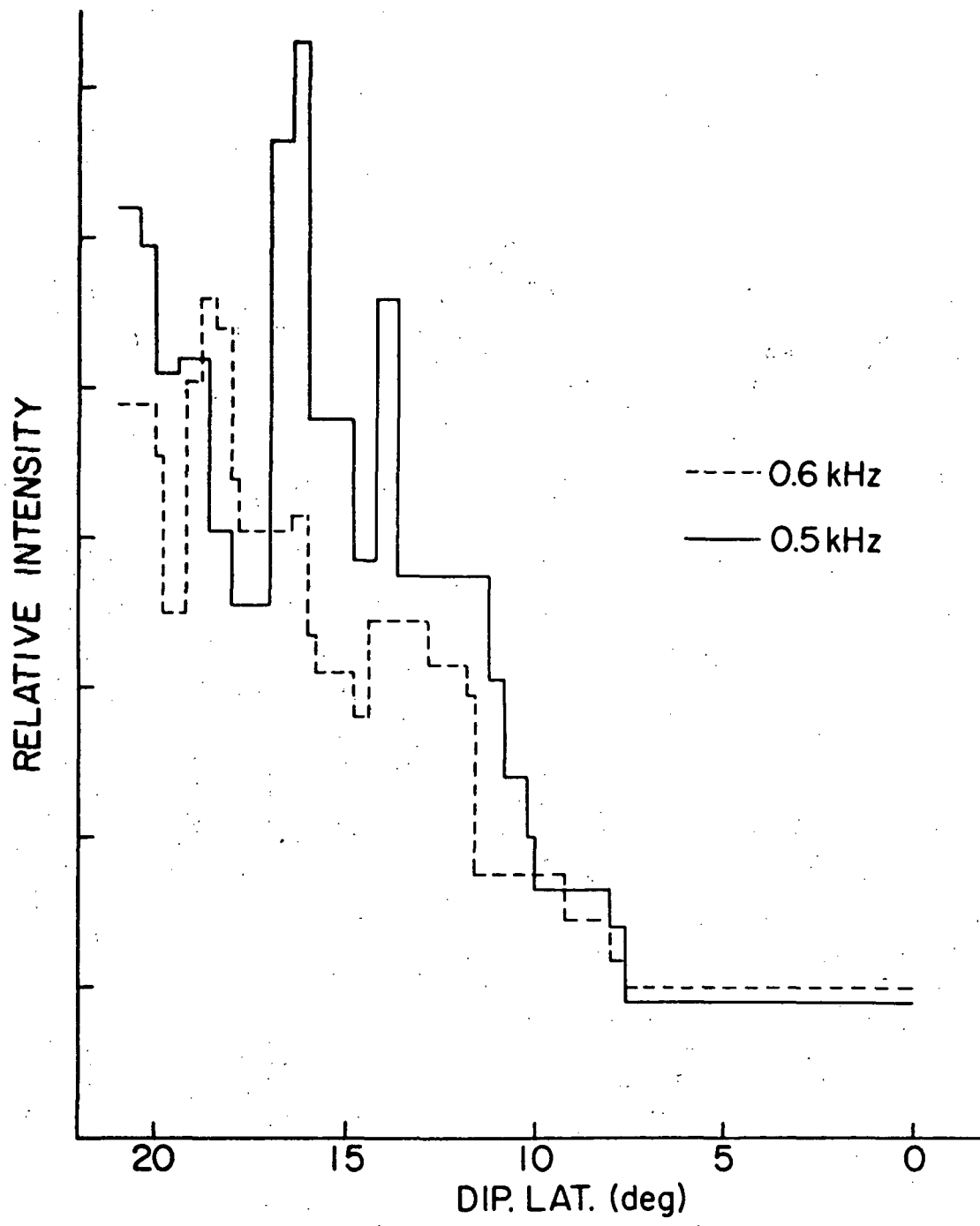
FIGURE 35. RELATIVE INTENSITIES OBTAINED FROM THE DISTRIBUTION OF POINTS OF FIG. 34 VS DIPOLE LATITUDE. The variation in intensity is consistent with the equatorial erosion.
