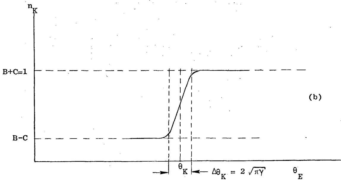
FIGURE 41a,b. FUNCTIONS USED TO SIMULATE THE EQUATORIAL ANOMALY (a) AND THE PLASMAPAUSE (b) IN THE MODEL IONOSPHERE.
