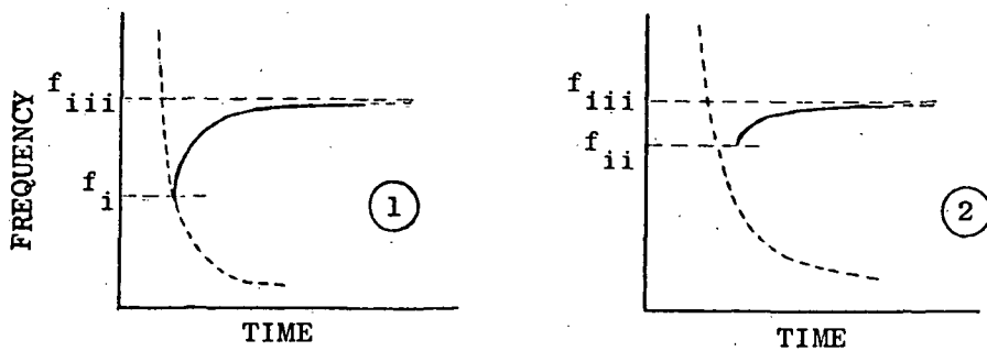
FIGURE 15. CURVES OF THE CHARACTERISTIC FREQUENCIES ALONG A FIELD-ALIGNED TRANSEQUATORIAL RAY PATH AND CORRESPONDING SPECTRA OF TWO 1^- PROTON WHISTLERS RECEIVED AT POSITIONS ① AND ②.
