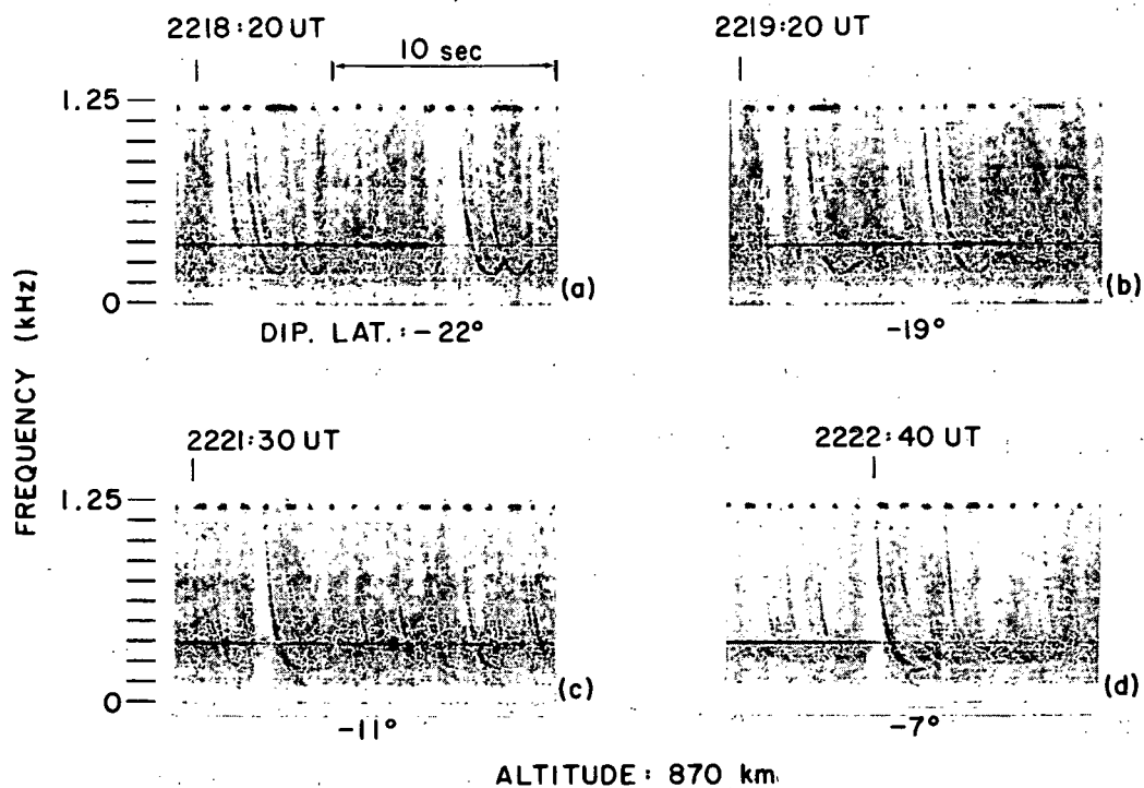
FIGURE 22. TRANSITION FROM SIMPLE ION CUTOFF WHISTLERS (IN (a) AND (b)) TO HYBRID FORMS (IN (c) AND (d)) WHEN THE VEHICLE APPROACHES THE EQUATOR.
