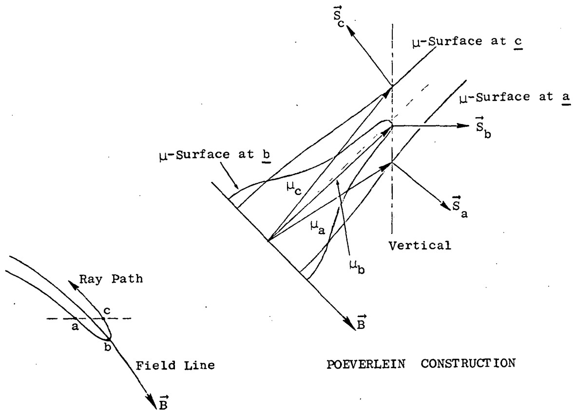
FIGURE 16. MECHANISM OF REFLECTION OF A WAVE IN THE SLOW MODE WITH LARGE WAVE NORMAL ANGLES, ACROSS THE TWO-ION RESONANCE LEVEL.
