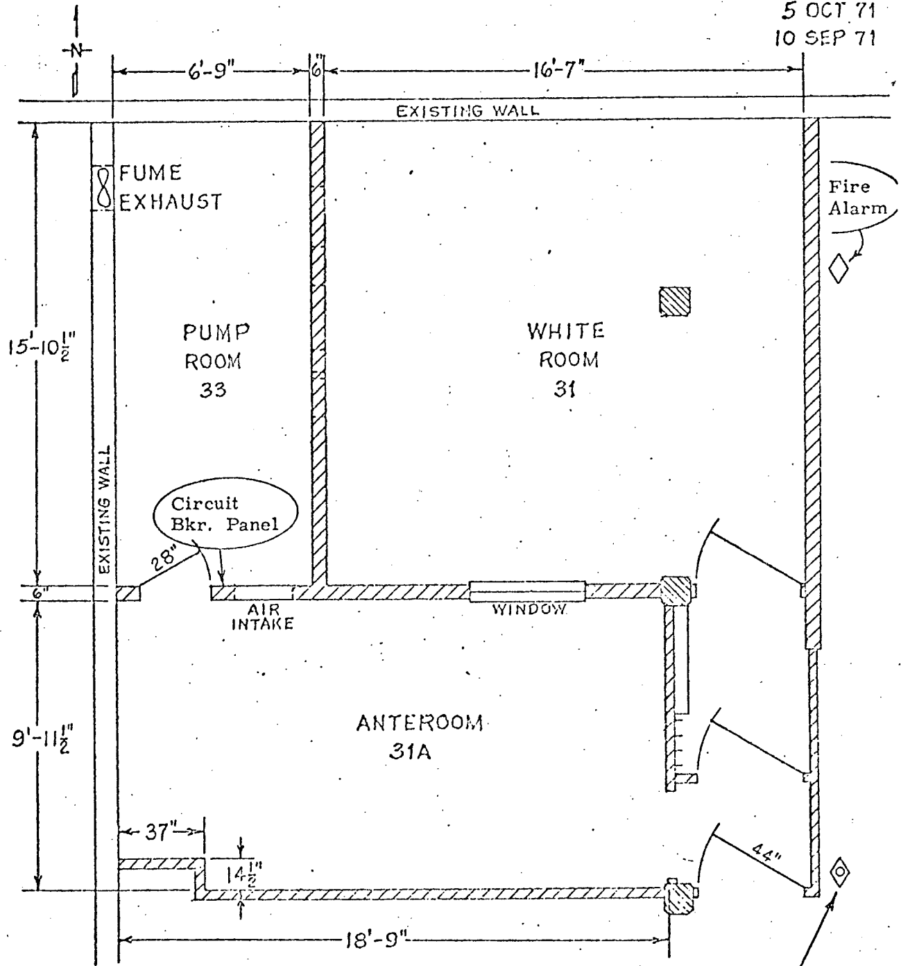
PLAN CALIBRATION FACILITY SAFETY/CONSTRUCTION LAYOUT SCALE: 1/4" = 1 FT.
