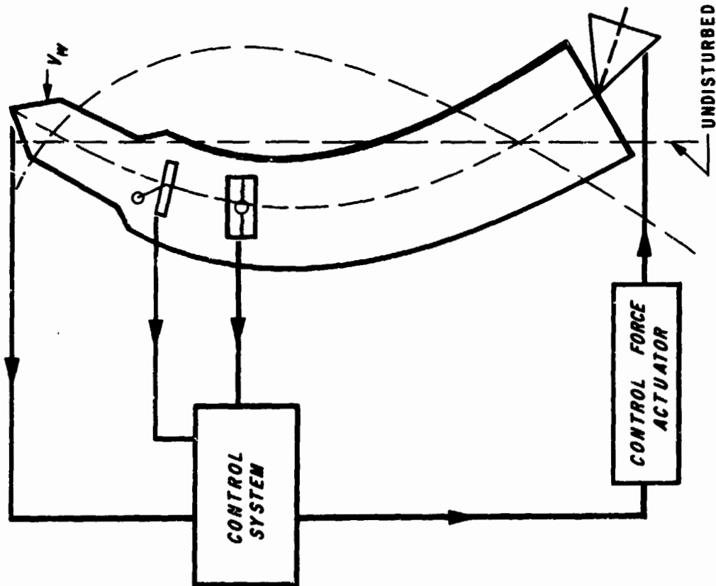
Figure 3. Feedback control system with bending.
