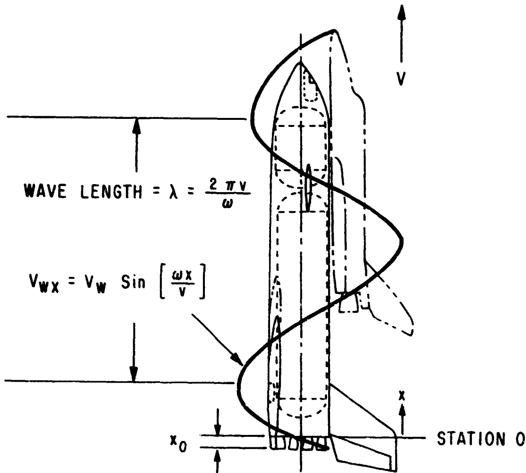
Figure 6. Gust penetration.
