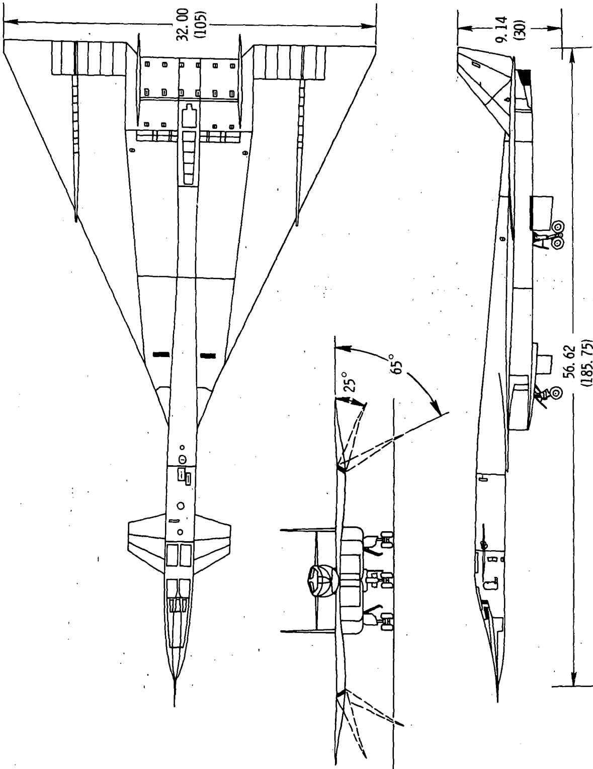
Figure 2. Three-view drawing of the XB-70-1 airplane. Dimensions in meters (feet) except as otherwise noted.
