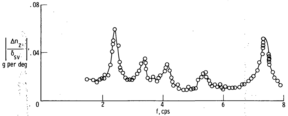
(j) Left wing; FS 55.17 m (2172 in.); BP 9.53 m (375 in.).
