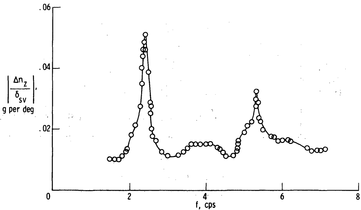
(g) Left wing; FS 56.18 m (2212 in.); BP 7.11 m (280 in.).
