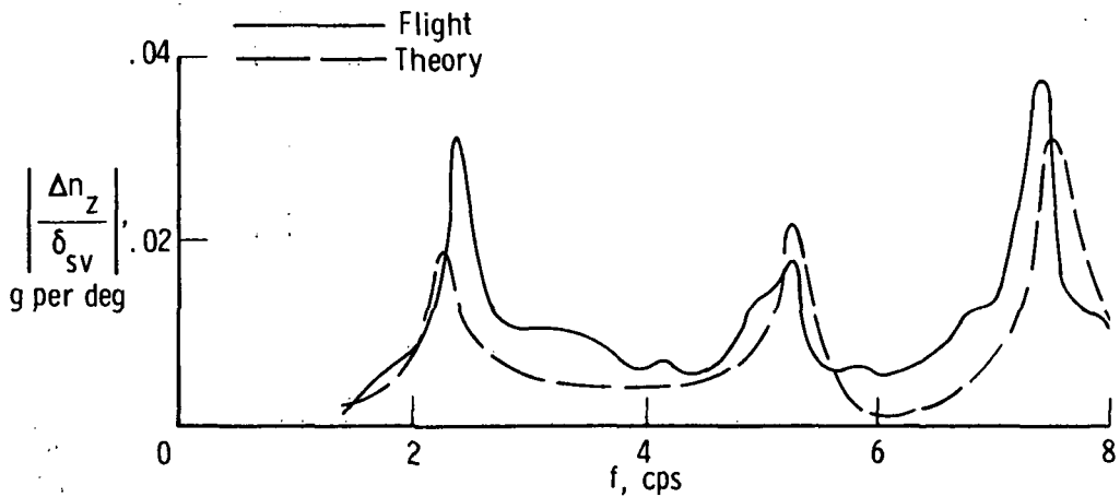
(b) Near center of gravity; FS 37.72 m (1485 in.).
