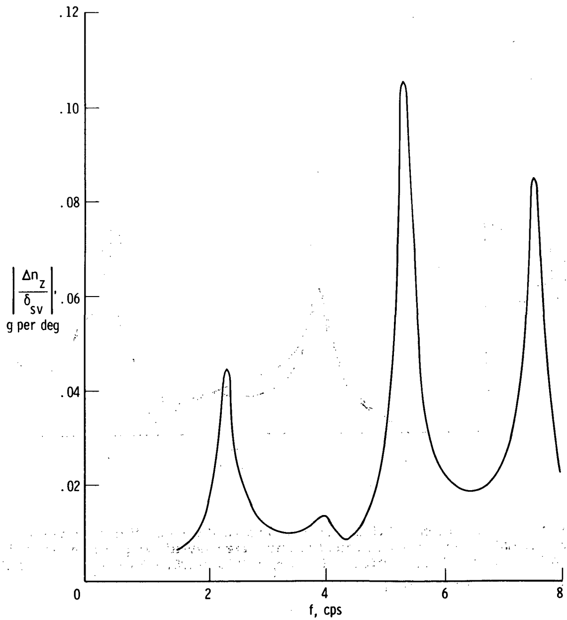
(e) Wing accelerometer; FS 56.18 m (2212 in.); BP 7.11 m (280 in.).
