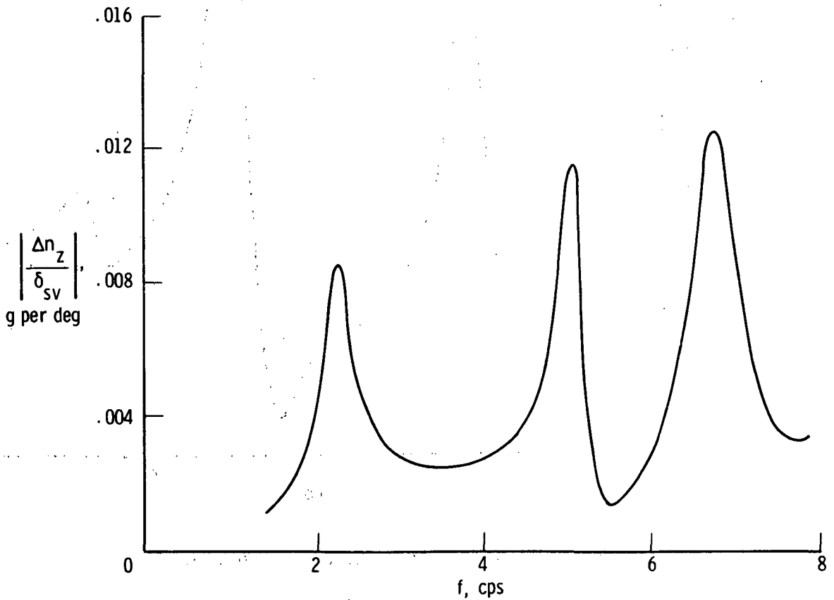
(d) Near center of gravity; FS 37.72 m (1485 in.).
