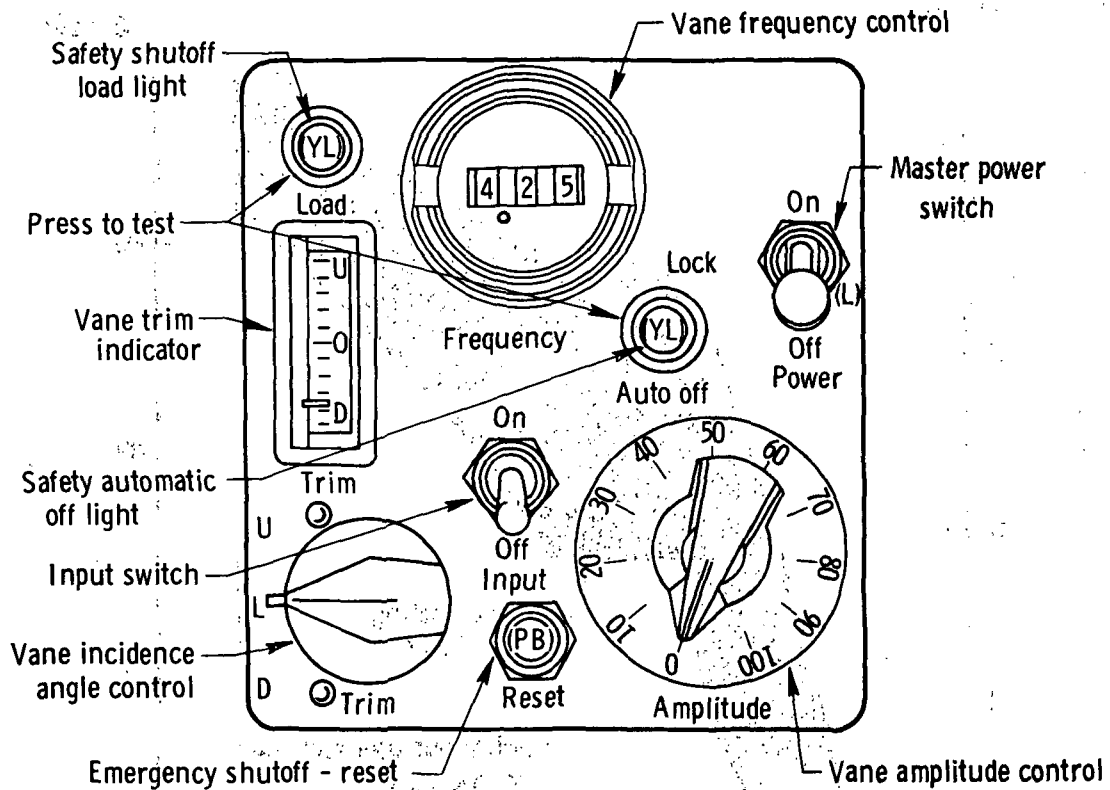
Figure 26. Shaker vane cockpit controls and display panel.
