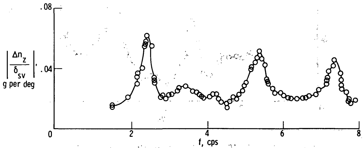
(g) Right wing; FS 56.18 m (2212 in.); BP 7.11 m (280 in.).
