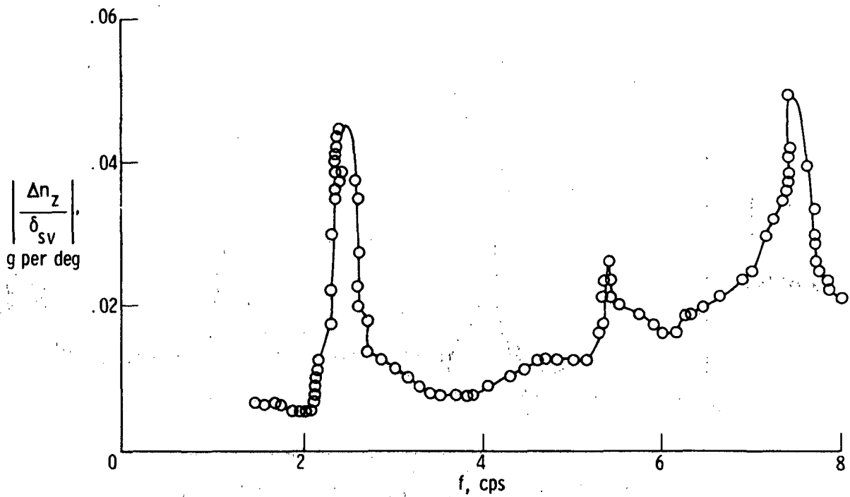
(f) Right canard tip; FS 15.70 m (618 in.); HS 4.32 m (170 in.).
