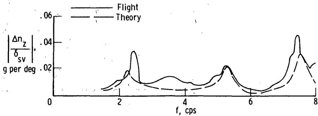
(c) Center of gravity; FS 41.99 m (1653 in.).
