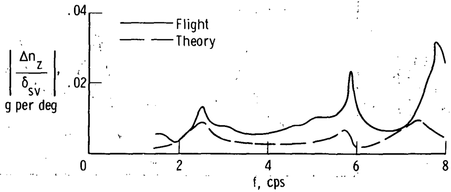
(c) Center of gravity; FS 41.99 m (1653 in.).
