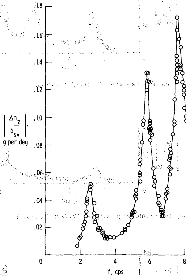
(a) Fuselage nose; FS 4.95 m (194.75 in.).
