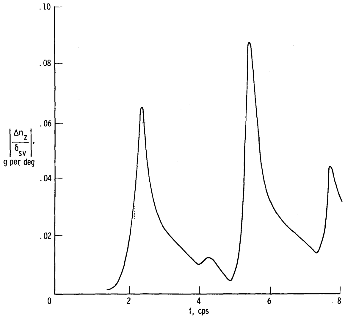
(b) Pilot's station; FS 11.12 m (438 in.).
