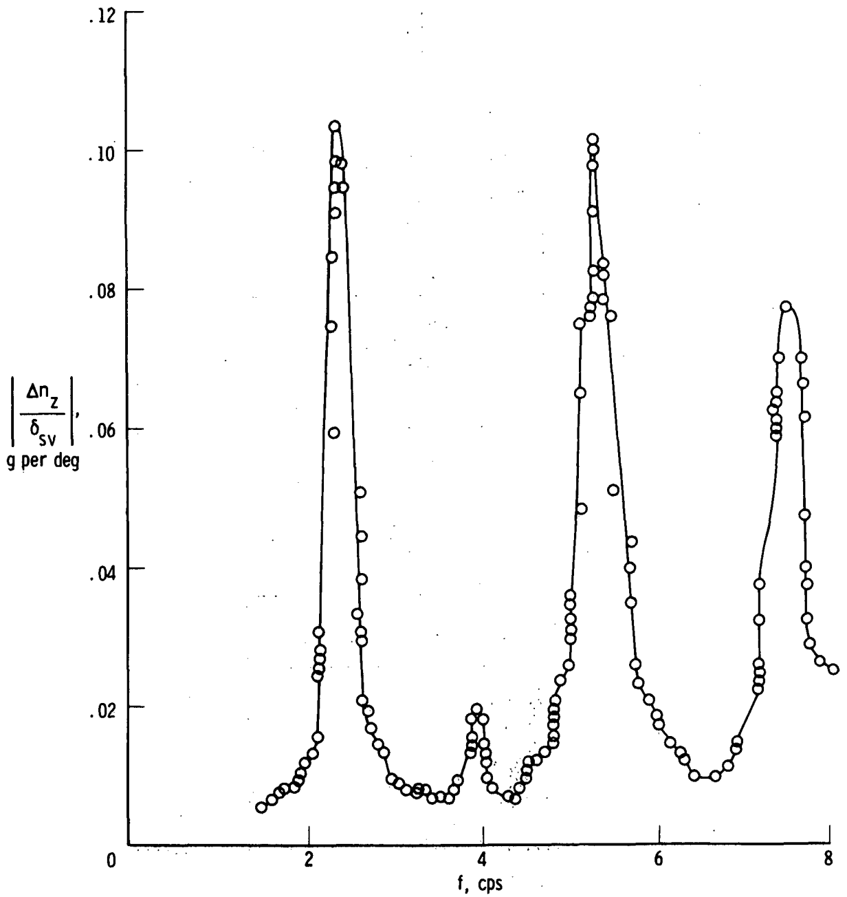
(a) Fuselage nose; FS 4.95 m (194.75 in.).
