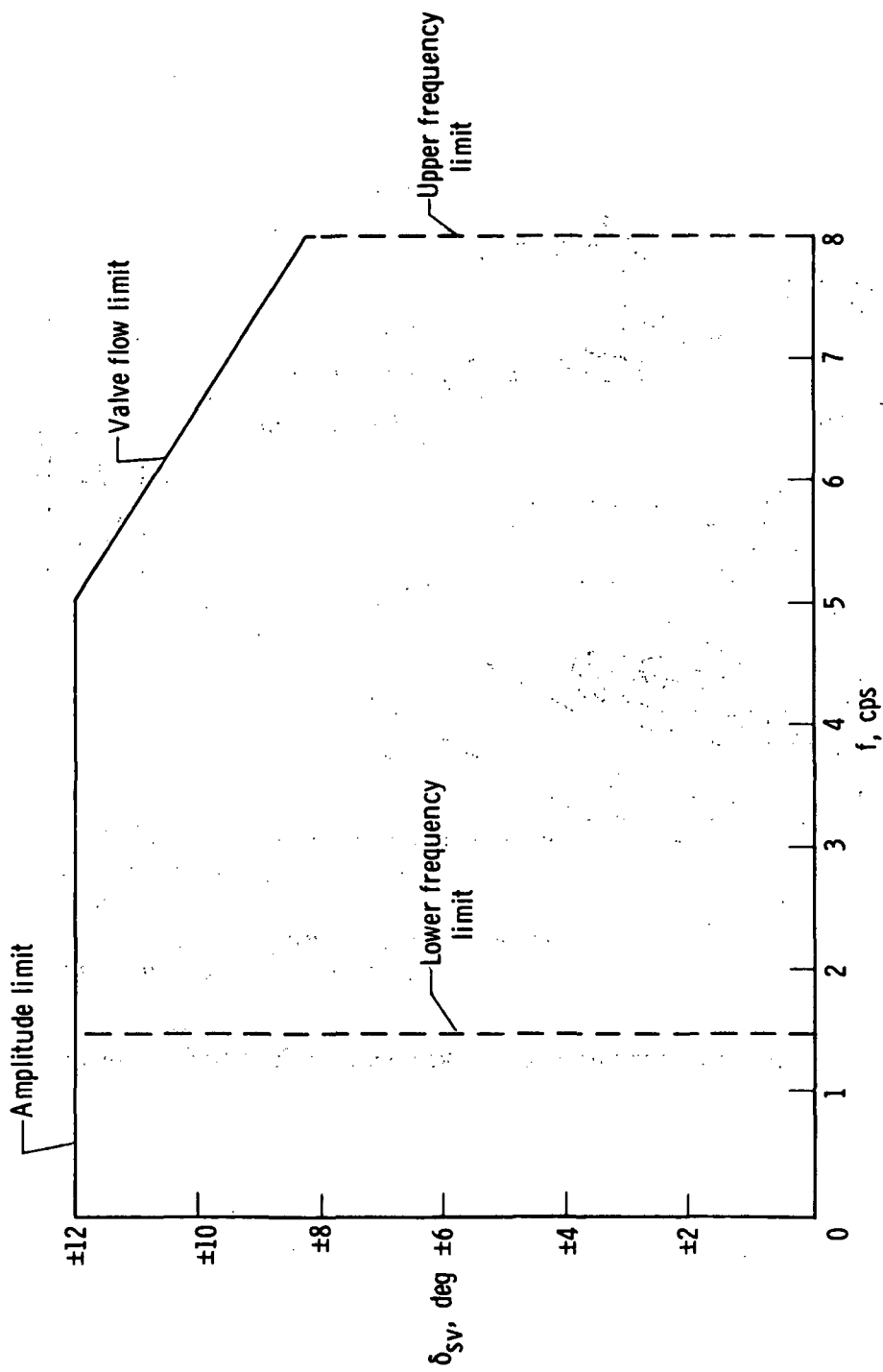
Figure 23. Variation of maximum shaker vane amplitude with vane oscillating frequency.
