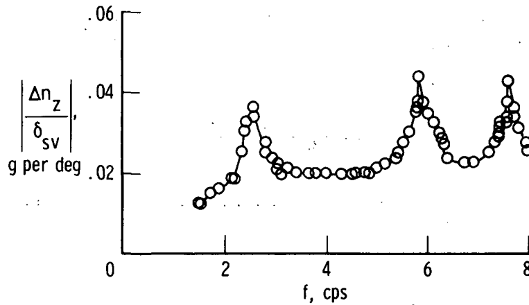
(i) Right wing; FS 56.18 m (2212 in.); BP 7.11 m (280 in.).
