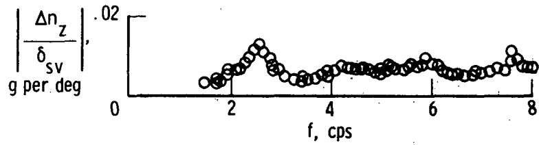
(e) Aft fuselage; FS 51.70 m (2035.5 in.).
