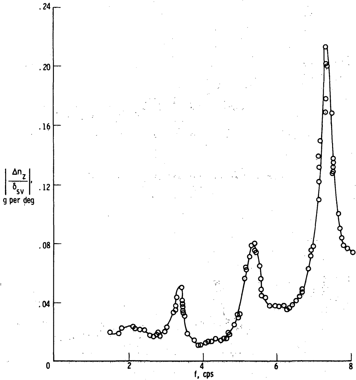
(i) Right wing; FS 46.23 m (1820 in.); BP 9.53 m (375 in.).
