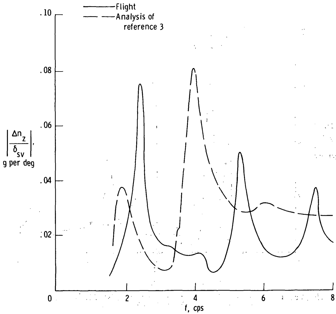
(c) Mediumweight; M = 1.59 ; h_p = 11,918 m (39,100 ft); \delta_t = 65^\circ .
