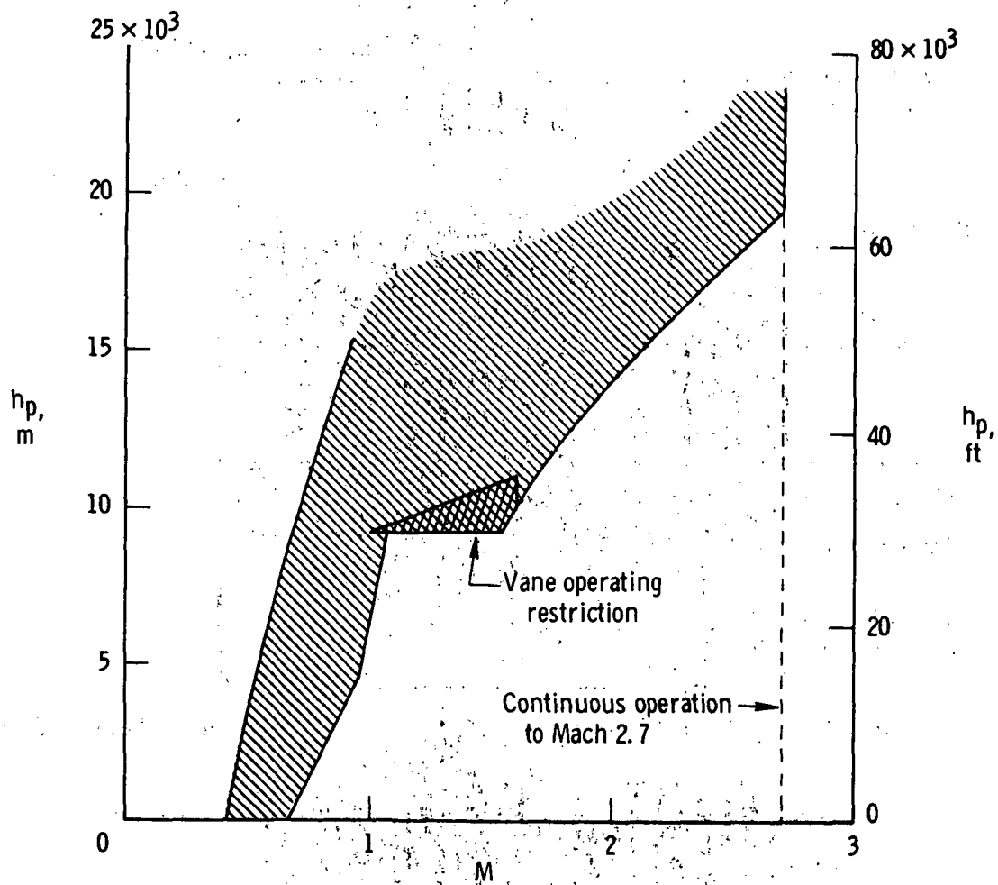
Figure 25. Operational range of the shaker vane.
