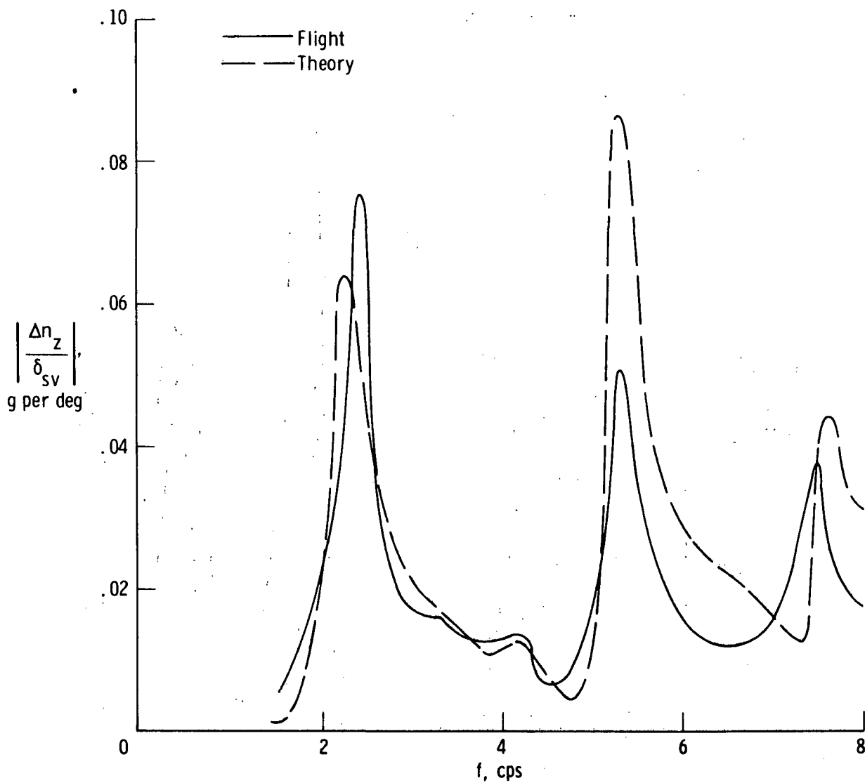
(c) Mediumweight; M = 1.59 ; h_p = 11,918 m (39,100 ft); \delta_t = 65^\circ .
