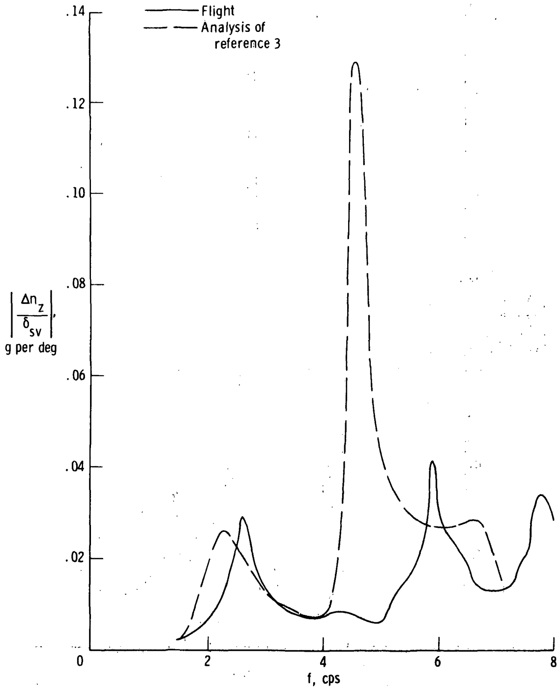
(b) Lightweight; M = 0.86 ; h_p = 7620 m (25,000 ft); \delta_t = 25^\circ .
