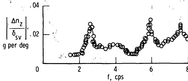
(l) Left wing; FS 55.17 m (2172 in.); BP 9.53 m (375 in.).
