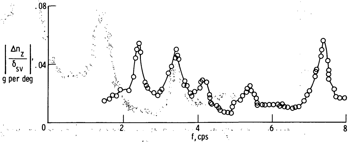
(k) Right wing; FS 55.17 m (2172 in.); BP 9.53 m (375 in.).
