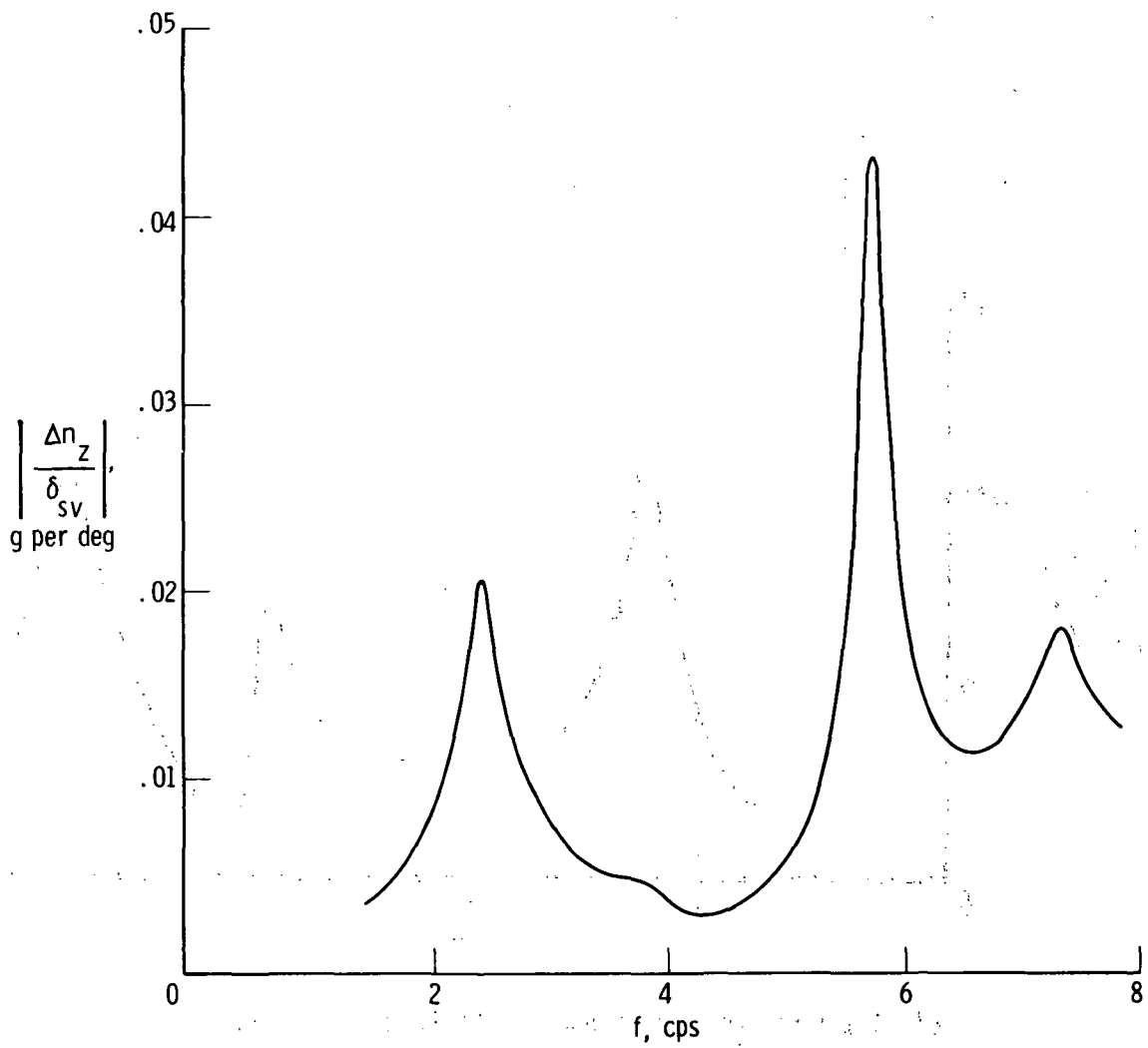
(e) Wing accelerometer; FS 56.18 m (2212 in.); BP 7.11 m (280 in.).
