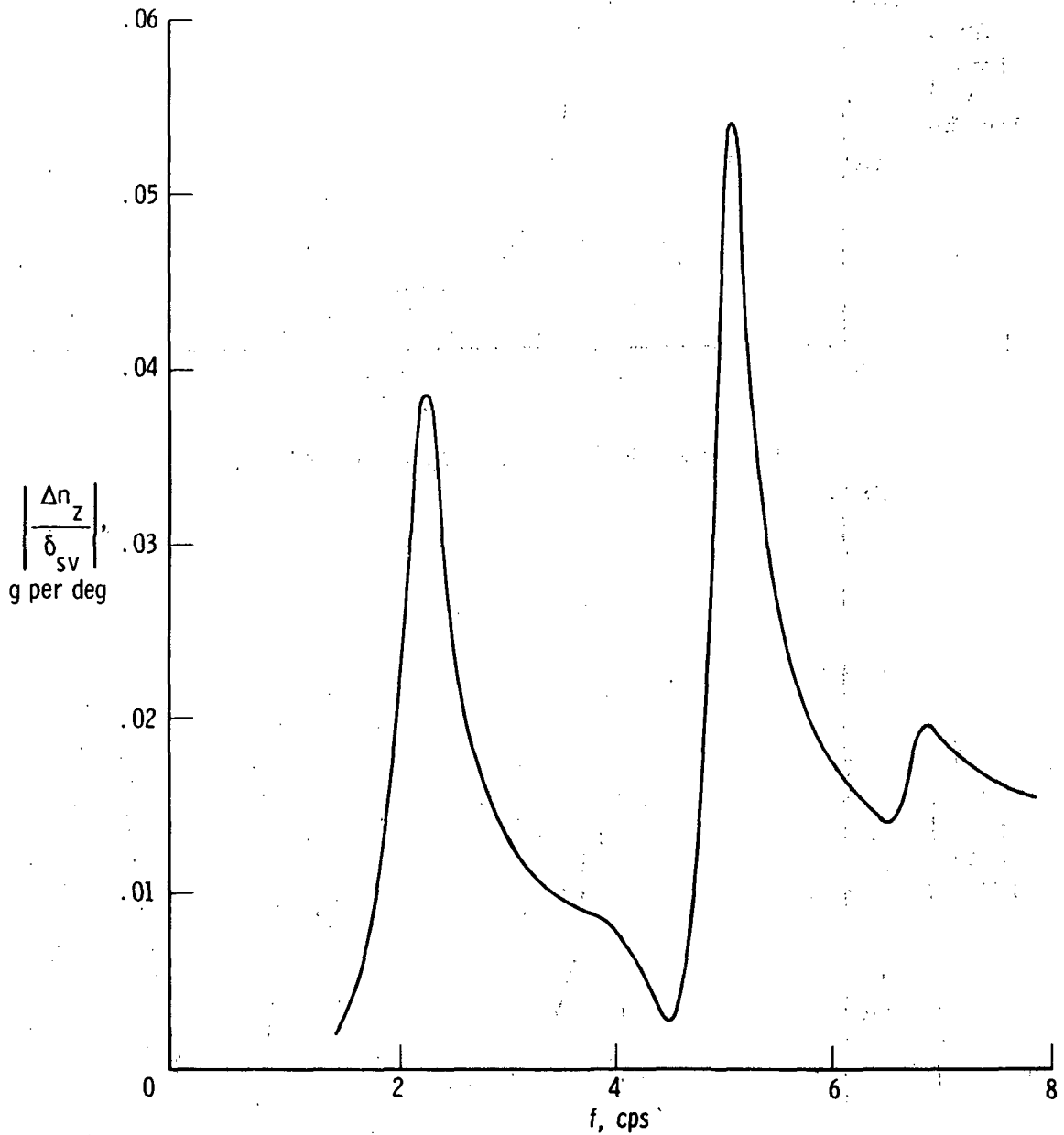
(b) Pilot's station; FS 11.12 m (438 in.).
