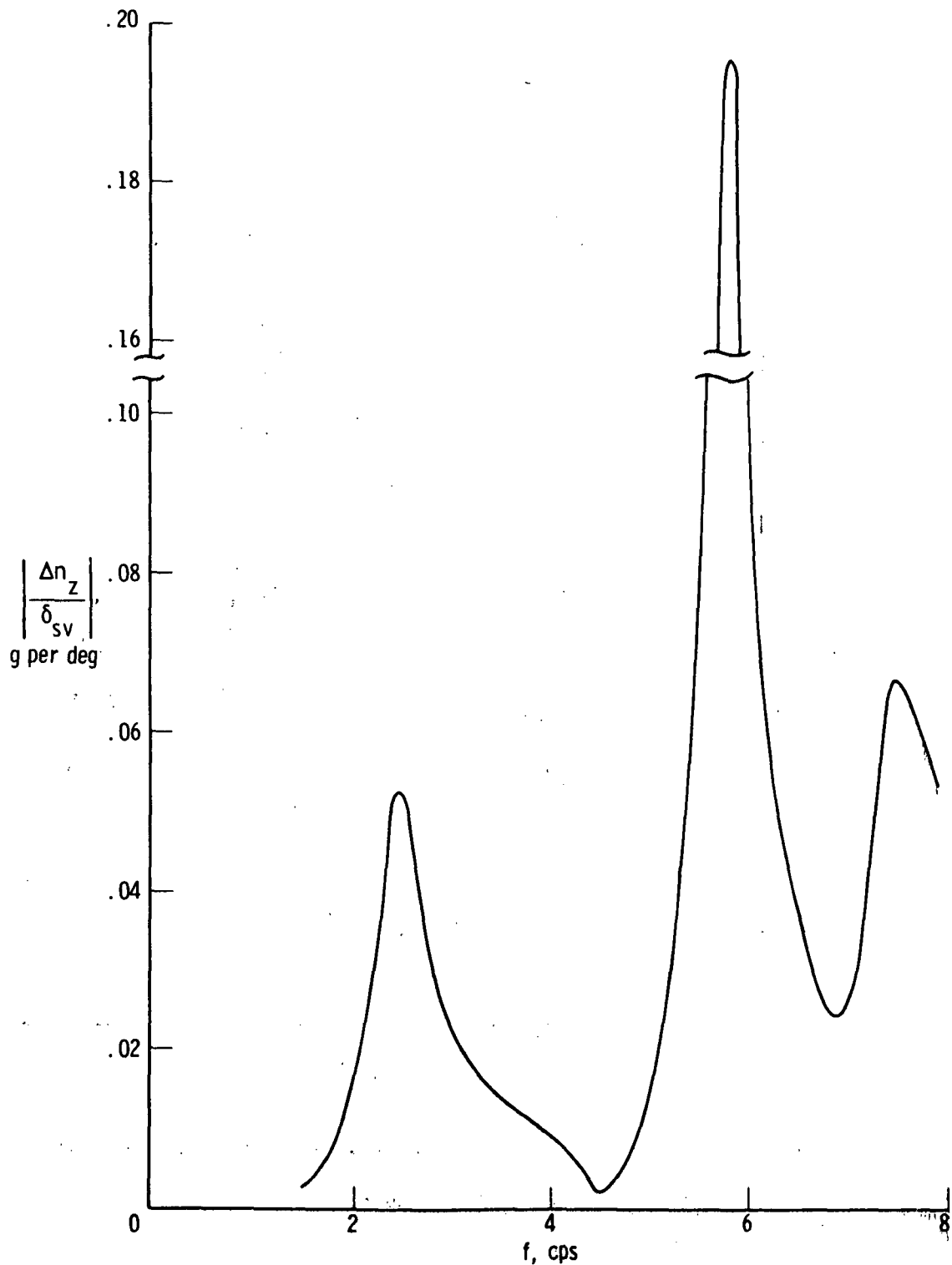
(a) Fuselage nose; FS 3.68 m (145 in.).
