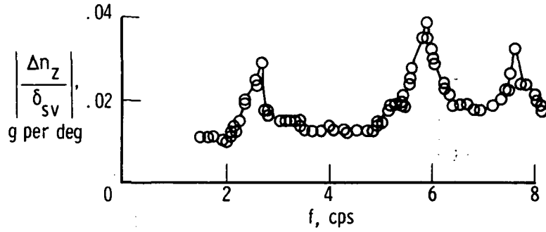
(h) Left wing; FS 56.18 m (2212 in.); BP 7.11 m (280 in.).
