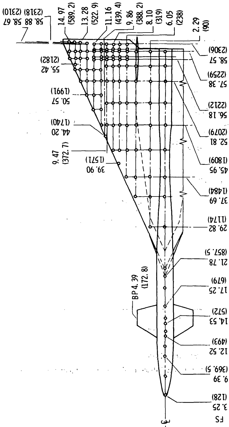
Figure 27. Control point geometry for XB-70 118-point grid system. Dimensions in meters (inches).
