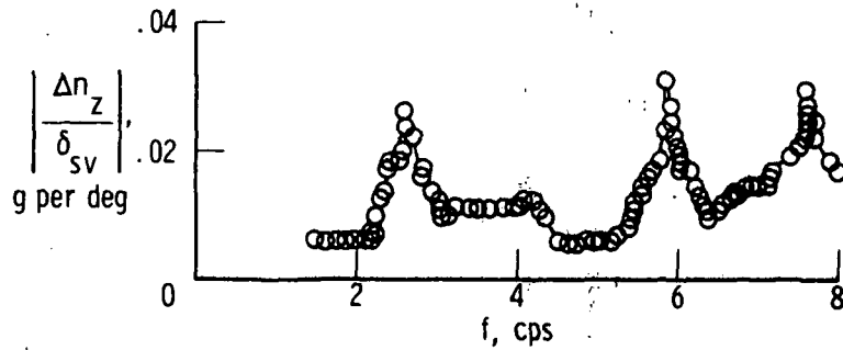
(m) Right wing; FS 55.17 m (2172 in.); BP 9.53 m (375 in.).
