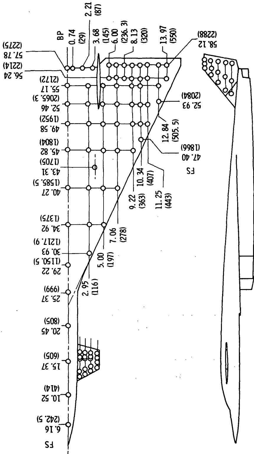
(a) Fuselage-wing. Dimensions in meters (inches).
