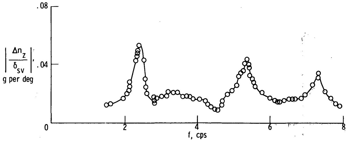
(f) Left wing; FS 56.18 m (2212 in.); BP 7.11 m (280 in.).
