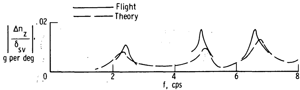
(b) Center of gravity; FS 41.99 m (1653 in.).
