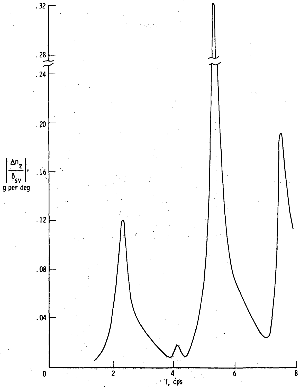
(a) Fuselage nose; FS 4.95 m (194.75 in.).
