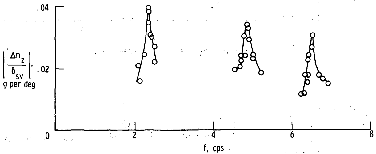
(f) Right wing; FS 56.18 m (2212 in.), BP 7.11 m (280 in.).
