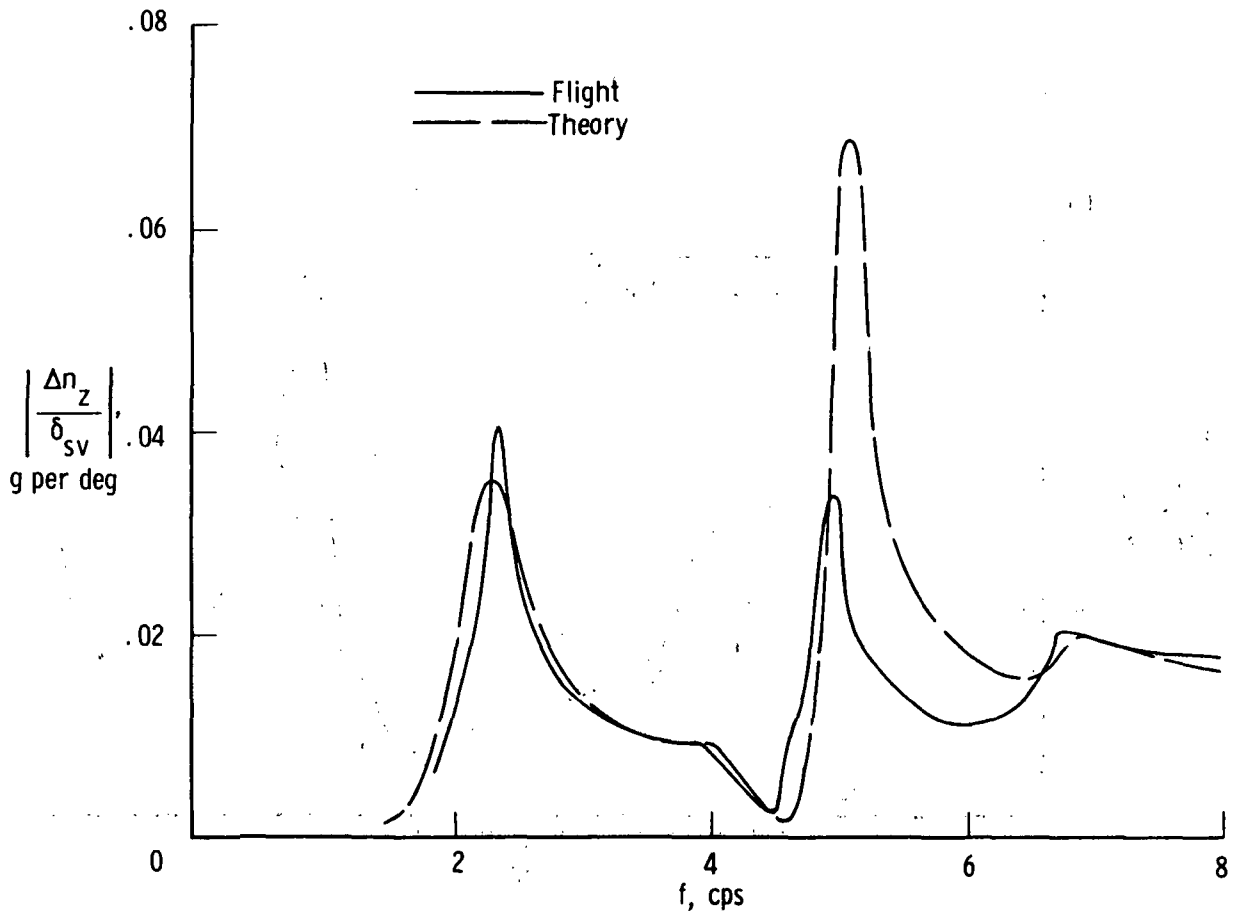
(a) Heavyweight; M = 0.87 ; h_p = 7620 m (25,000 ft); \delta_t = 25^\circ .
