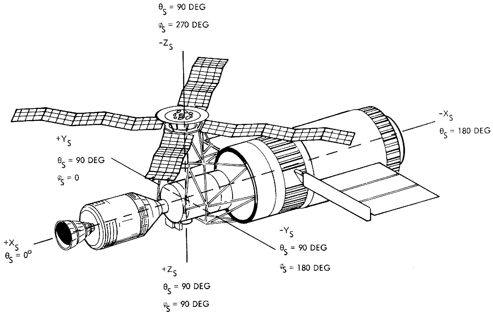
Figure 2. Skylab OA Coordinate System (MDAC \theta , \phi Convention)
