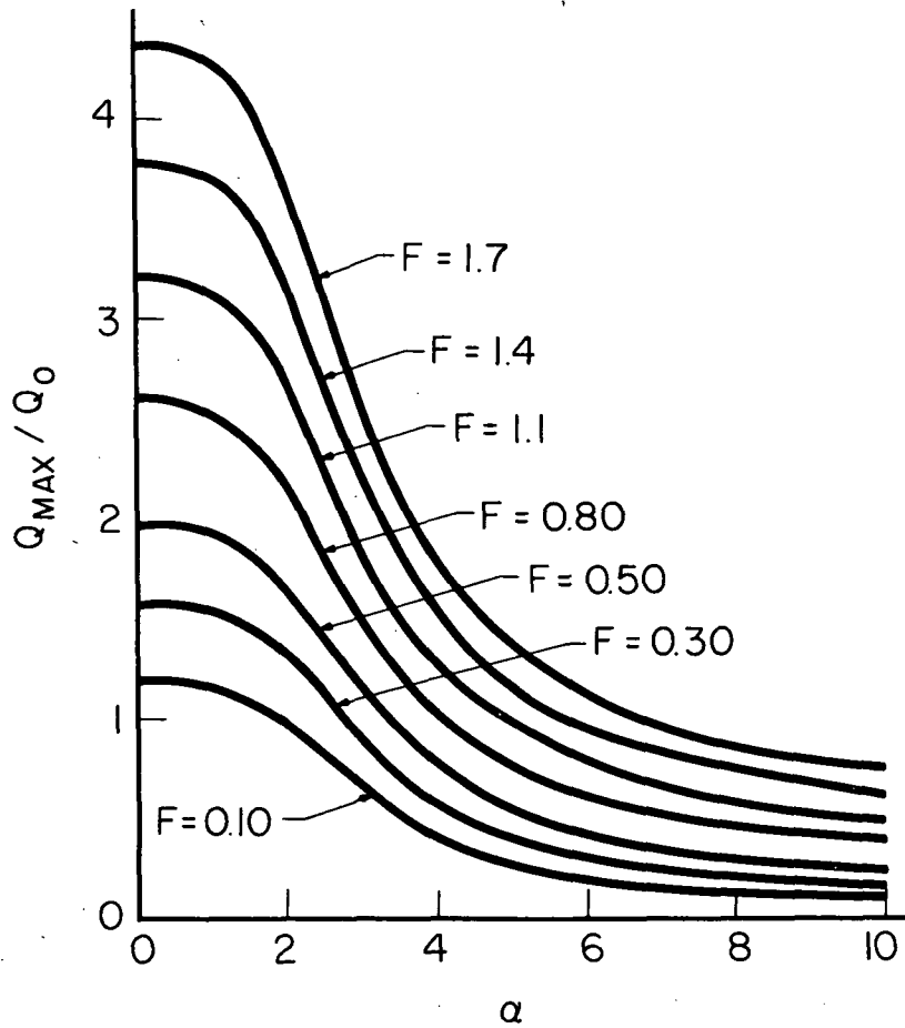
Fig. 5 - Mass Flow Magnitude in Pulsatile Flow With In-Phase Simusoidal Pressure Gradient and Wall Motion, \phi = 0^\circ
