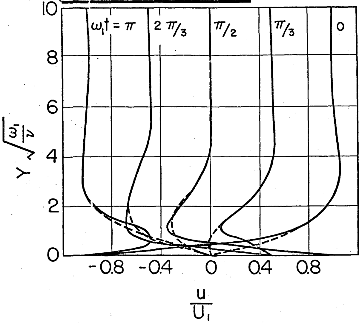
Fig. 4 - Typical Pulsatile Flow Velocity Profiles With and Without Vibration as Calculated from Equation (3)
