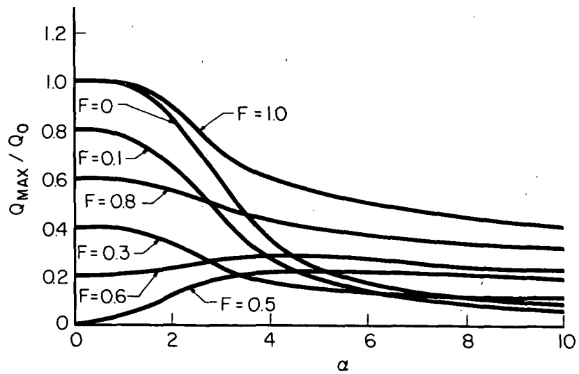
Fig. 6 - Mass Flow Magnitude in Pulsatile Flow for Simusoidal Pressure Gradient and Wall Motion Acting in Opposition, \phi = 180^\circ
