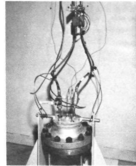
Reaction Chamber for Evaluating Behavior of Nonmetal Materials When Heated in Hydrogen
