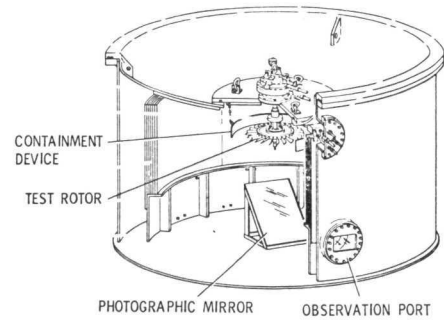
Facility to Study Ways of Containing Fragments and Typical Test Results
