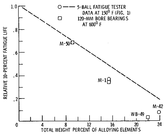
Figure 2. - Effect of total weight percent of alloying elements on fatigue life of 120-mm bore bearings at 600° F. CS-67903
