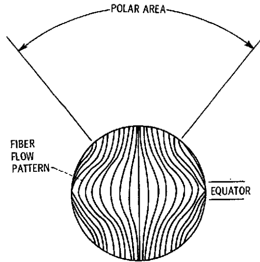
Figure 13. - Fiber orientation in a bearing ball.
