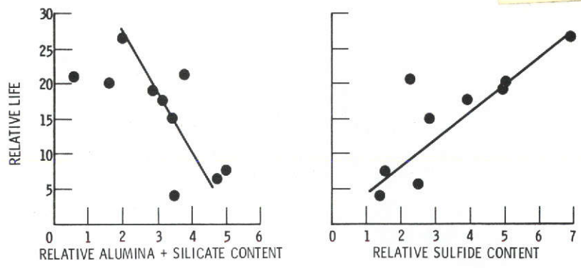
Figure 5. - Relationship between life and inclusion content.
