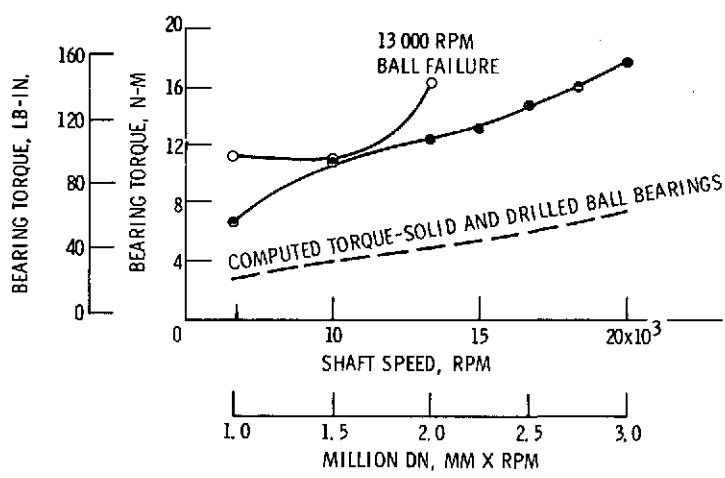
(b) BEARING TORQUE.
