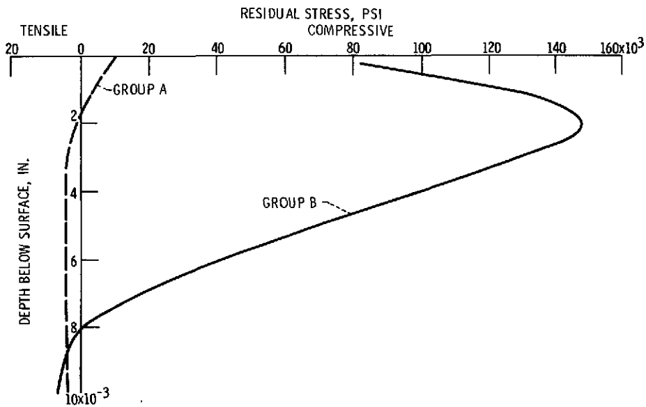
Figure 20. - Tangential residual stress patterns for two groups of 40 mm bore-size bearing races. CS-67908
