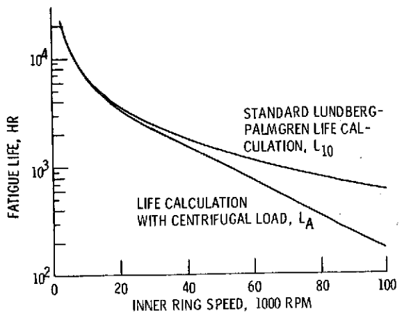
Figure 21. - Comparison of fatigue life of 20-mm-bore ball bearings with 100-lb radial load with and without centrifugal effects considered. CS-67893
