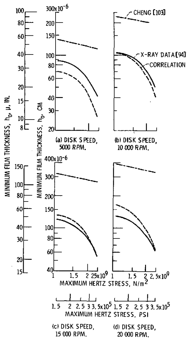
Figure 24. - Comparison of predicted minimum film thickness with X-ray data for a synthetic paraffinic oil at T_0 = 339 K (150° F). GS-67914
