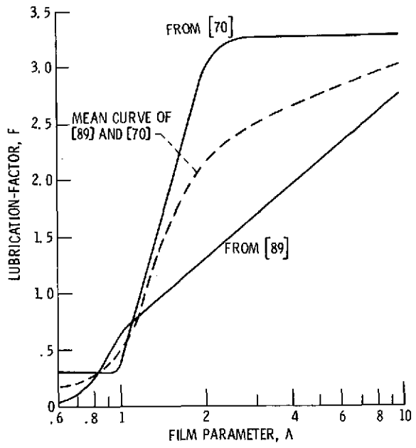
Figure 23. - Lubrication factor, F as function of film parameter, lambda. CS-67909
