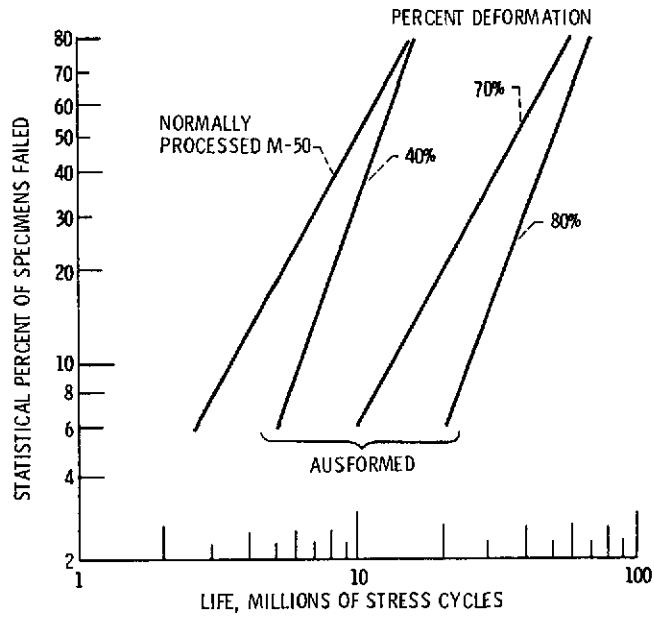
Figure 19. - Effect of ausforming on fatigue life for M-50 bearing steel. CS-67907
