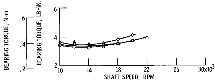
(b) OIL JET LUBRICATION AT 0.95 POUNDS PER MINUTE.
