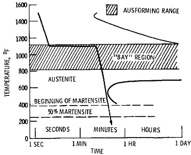
Figure 18. - Time temperature-transformation curve for a typical "M"1-type bearing steel ("Bay" or hold region makes this type of steel suitable for ausforming. Arrow indicates ausforming cycle.)
