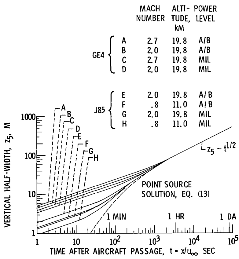
Figure 1. - Exhaust plume vertical half-width for GE4 and J85 engines at several flight conditions: D = 2 \times 10^{-4} \text{ M}^2/\text{sec}^3 ; K_z = 1 \text{ M}^2/\text{sec} ; A/B = maximum afterburning; MIL = maximum power without afterburning.
