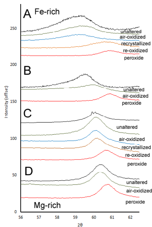
Figure 2. XRD (060) region for four ferrous smectites and their oxidative products. Peaks shift to higher 2\theta with oxidation, indicating a contracting octahedral shell.
