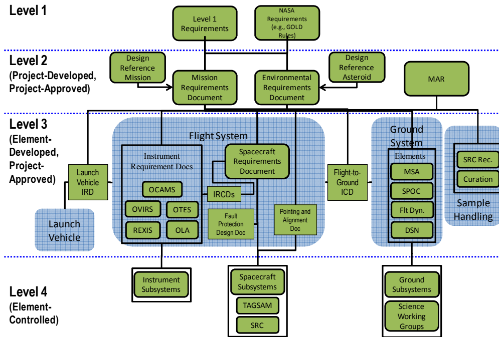
Figure 1 - Requirements Flow-down
