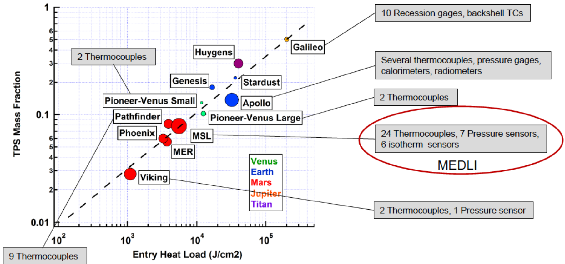
Chart credit: Deepak Bose/ARC. Circle sizes represent relative vehicle diameter. EFT-1 not shown.
