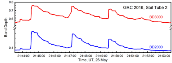
Figure 4. Enlargement of the orange rectangle in bottom of Fig. 3 showing the percussive activity.
