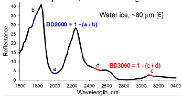
Figure 2. Ice parameters for monitoring water ice.
