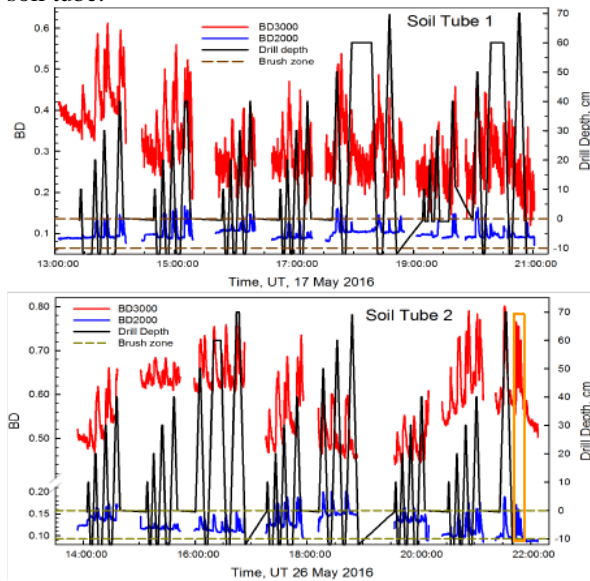
Figure 3. Volatile parameters (BD 2000 and BD3000) are shown for ST1 (top panel) and ST2 (bottom panel) along with the drill depth. Negative drill depths are above the soil surface where the bottom 10 cm of the drill stem is being actively brushed.
