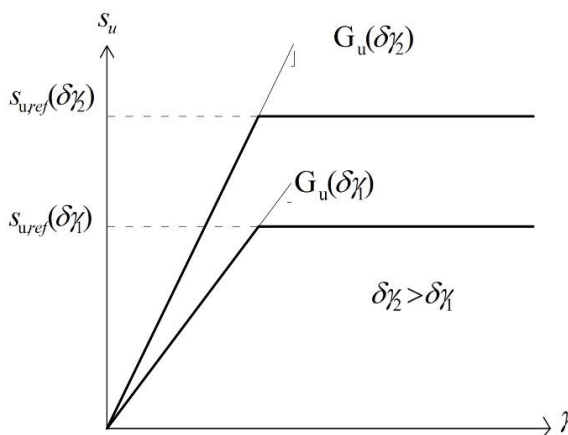
Fig. 2. Mohr-Coulomb model extended with strain-rate effect at a constant water content with strain rate with \delta\gamma_2 > \delta\gamma_1 .
