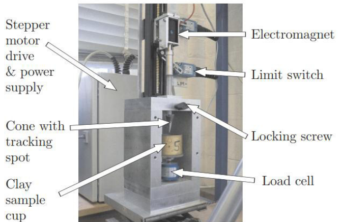
Fig. 1. Free-fall cone test experiment [7].
