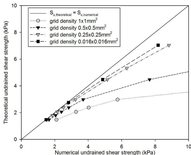
Fig. 5. Numerical errors investigation.
