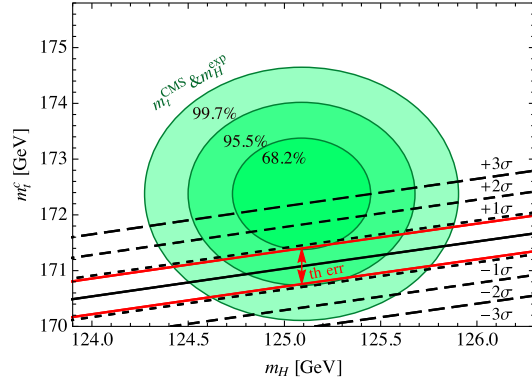
FIG. 4. Lines for which the Higgs potential develops a second degenerate minimum at high energy. The solid line corresponds to the central value of \alpha_s^{(5)} ; the dashed lines are obtained by varying \alpha_s^{(5)} in its experimental range, up to 3\sigma . The (red) arrow represents the theoretical error in the position of the lines. The (green) shaded regions are the covariance ellipses obtained combining m_t^{\text{CMS}} = 172.38 \pm 0.66 GeV [49] and m_H^{\text{exp}} = 125.09 \pm 0.24 GeV.
