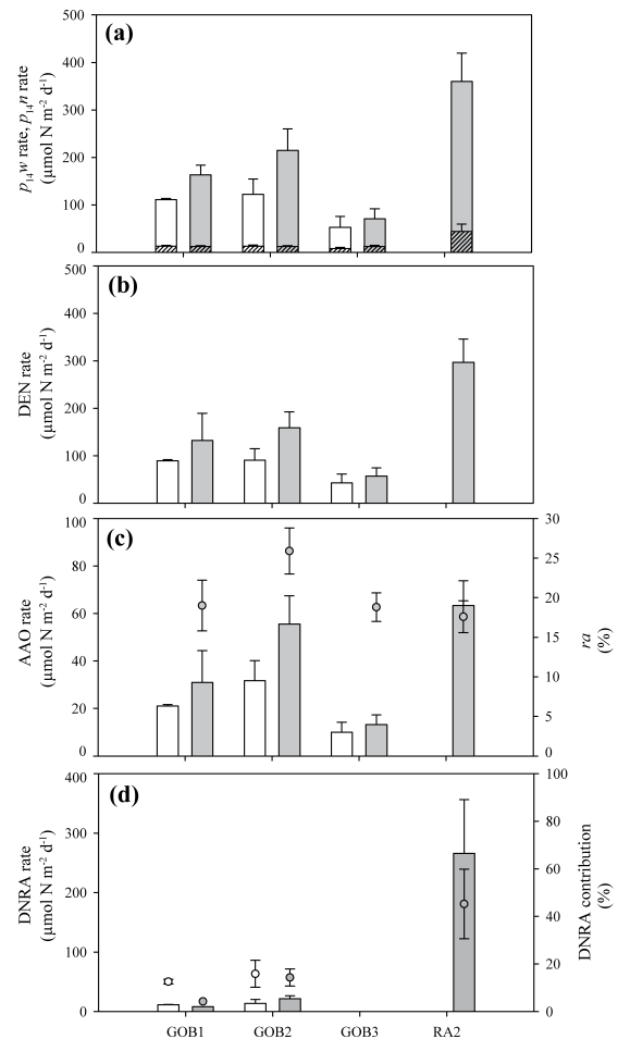
Figure 6. Average rates of NO 3 - -reducing processes measured at the four stations by in situ incubations with benthic chamber landers amended with 15 N-nitrate, where white and grey bars represent 2013 and 2014 rates, respectively, with associated standard errors: (a) hatched bars represent rates of N 2 production depending on the water column nitrate ( p_{14w} ), while unhatched bars represent rates of N 2 production coupled to nitrification ( p_{14n} ); (b) bars represent total denitrification (DEN) rates; (c) bars represent total anammox (AAO) rates and refer to the left y axis, while grey dots represent percentages of ra and refer to the right y axis; and (d) bars represent total DNRA rates and refer to the left y axis. White and grey dots represent contribution of DNRA to total nitrate reduction (DEN rate + DNRA rate) and refer to the right y axis for year 2013 and 2014, respectively. DNRA rates at GOB3 were not significant.
