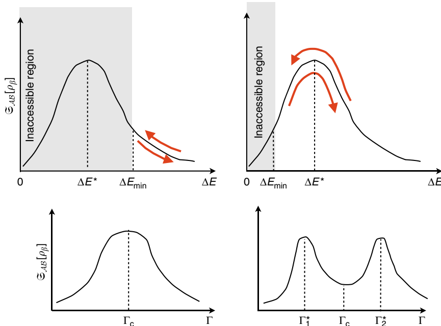
Figure 5 | Heat capacity in the Landau-Zener model. The emergence of extremal points in the behaviour of \mathfrak{S}_{AB}[\rho_\beta] as a function of increasing control parameter \Gamma is associated to the relative size of \Delta E_{\min} with respect to \Delta E^* . The red arrows denote the changing of \Delta E during a typical Landau-Zener protocol. One realizes that, if \Delta E_{\min} > \Delta E^* one peak will appear (left), whereas if \Delta E_{\min} < \Delta E^* two peaks will appear (right).
