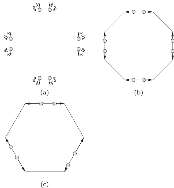
Fig. 1 (a) A Biangular configuration, with local axes oriented in such a way that all robots have the same view. (b) The correct way to resolve a Biangular configuration. (c) A generic Pre-regular configuration with its supporting polygon, which remains invariant as the robots move according to the arrows.
