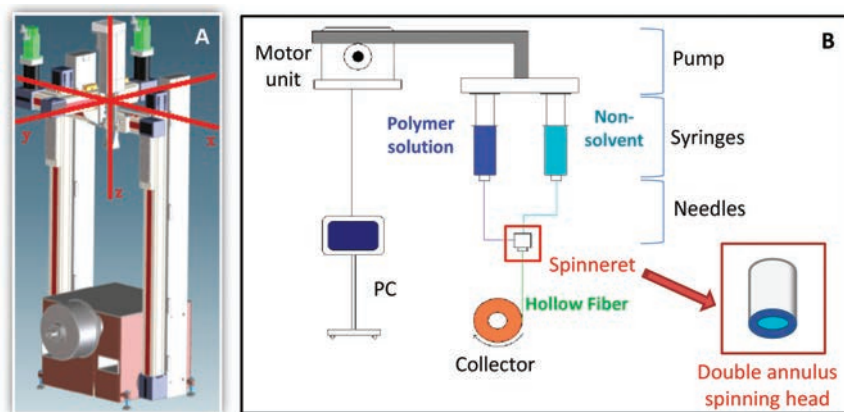
Figure 1. Scheme of the dry-wet spinning system and process: A) 3D drawing showing the spinning system and its moving axes; B) sketch representing the spinning process and key components.
