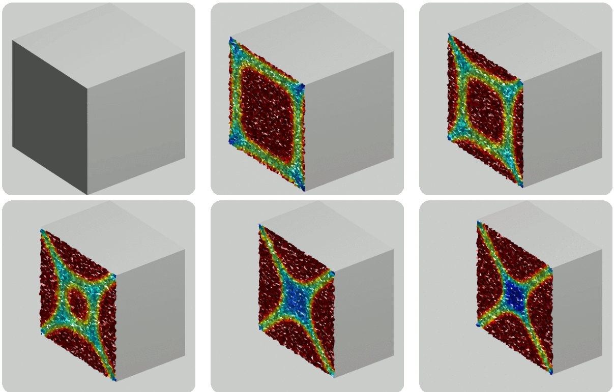
Figure 5: Tomographic view of the optimal solution defined in a cube for m = 5 . The free boundary is visible in light color and is very close to the cut locus of the cube
