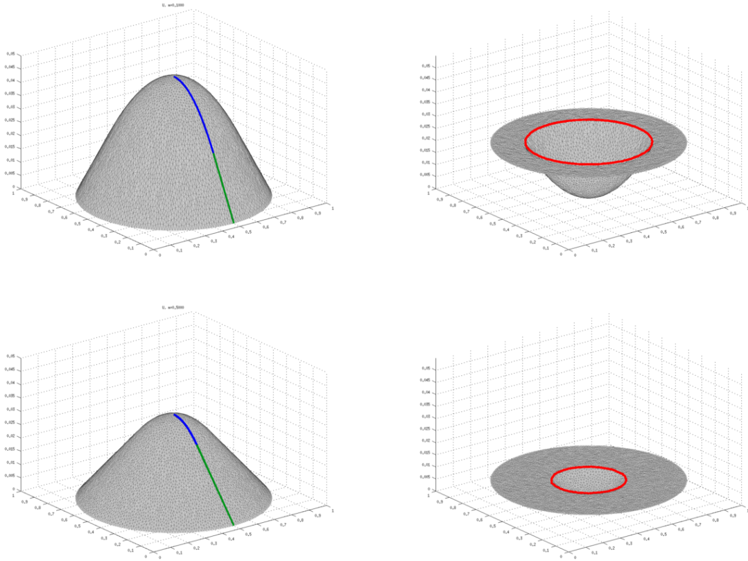
Figure 1: Optimization on a disk for m = 0.1, 0.5
