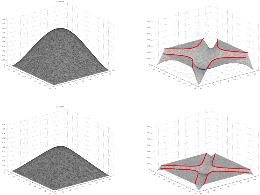
Figure 2: Optimization on a square for m = 0.1, 0.5
