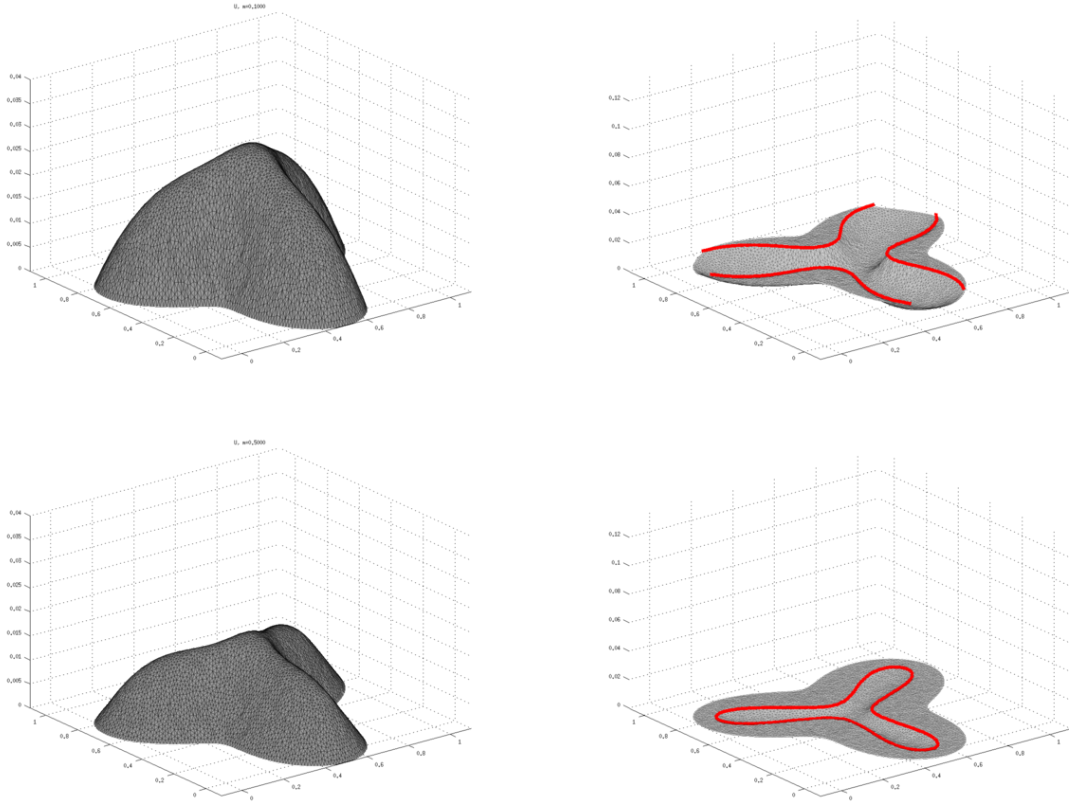
Figure 4: Optimization on a trefoil for m = 0.1, 0.5
