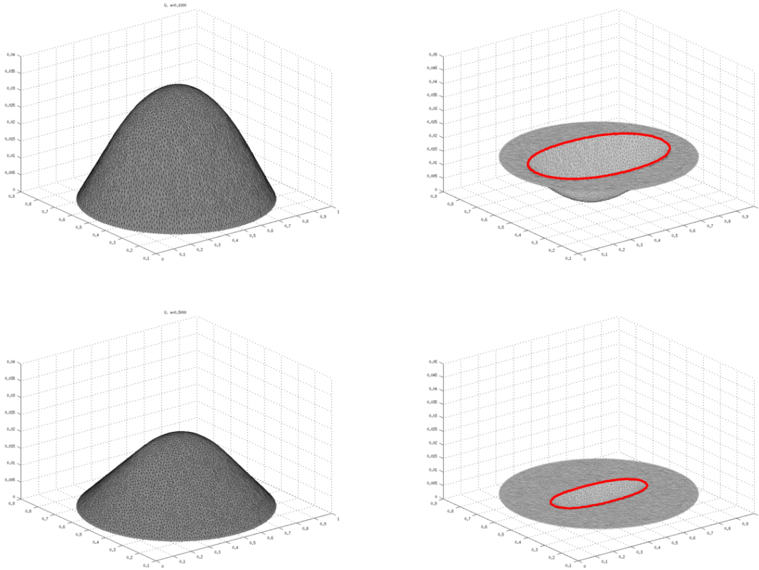
Figure 3: Optimization on an ellipse for m = 0.1, 0.5
