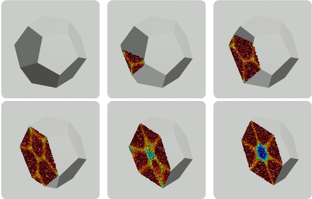
Figure 6: Tomographic view of the optimal solution defined in a dodecahedron for m = 5 . The free boundary is visible in light color and is very close to the cut locus of the dodecahedron
