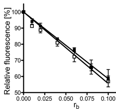
Fig. 6 Ethidium bromide fluorescence. Dependences of the EtBr fluorescence on r_b for CT DNA modified by platinum complexes in 10 mM NaClO 4 at 37 °C for 24 h. Open symbols, cis -PtI 2 (NH 3 ) 2 ; closed symbols, cisplatin.
