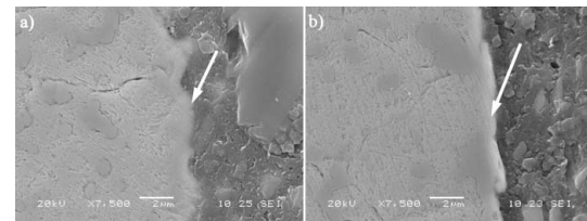
Fig.8: SEM micrograph of section of the \mu\text{-EDM} drilled hole samples where a recast layer of about 1-2 \mu\text{m} is clearly visible (see arrows).
