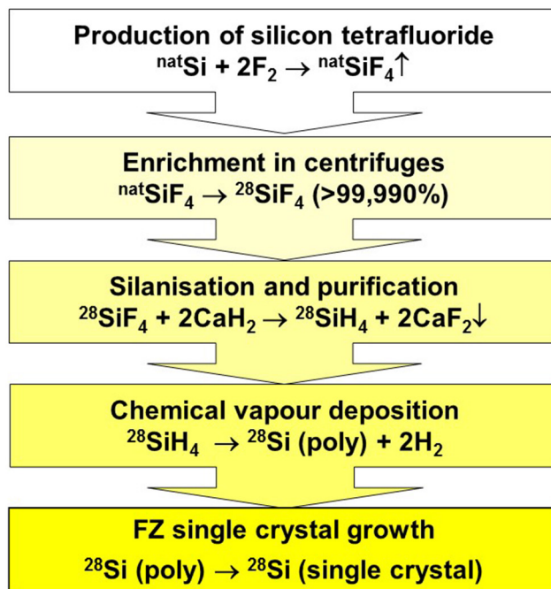
Figure 3. Flow chart showing the production of a 28 Si-enriched silicon single crystal ( nat Si: silicon with natural isotopic composition, poly: polycrystal).
