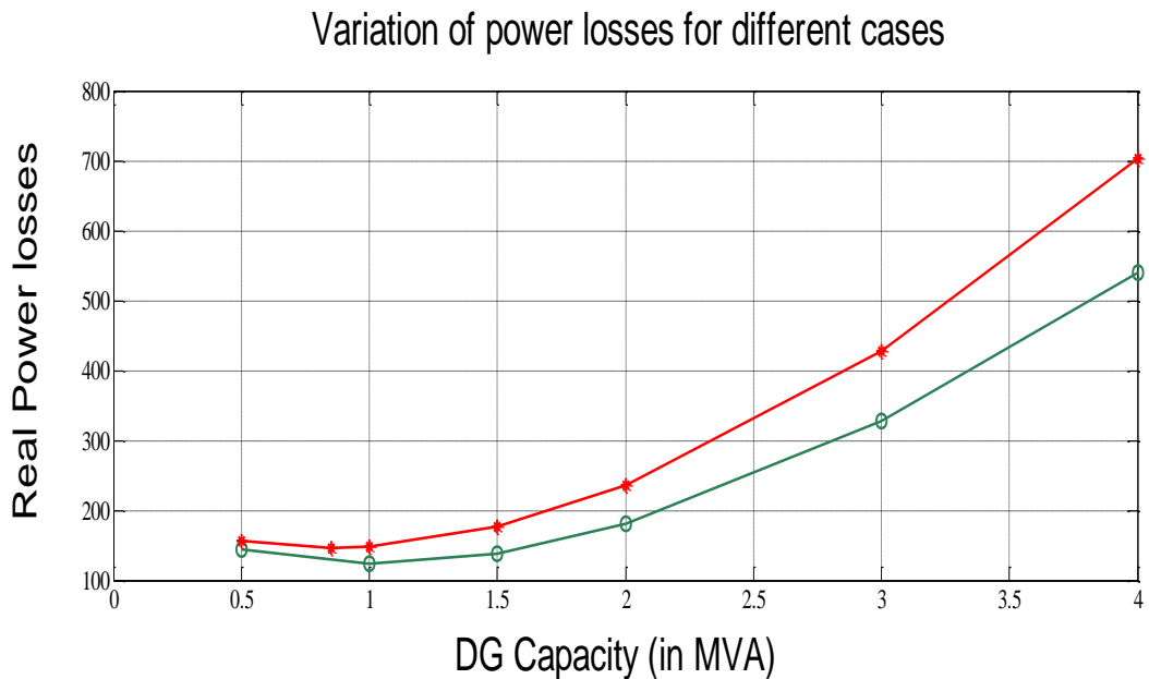
Figure 6.6: Variation of Power Losses for Different Cases for 33 Bus
