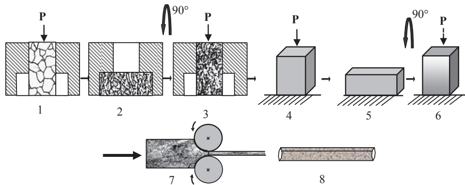
FIGURE 1. Isothermal multi-axial forging scheme and further rolling of samples: 1—initial sample (arrow shows the direction of the imposed load during compaction in a pressing mold); 2—the sample after the first compaction; 3—pressing repetition with the rotation of deformation axis in pressing mold; 4—sample before free isothermal multi-axial forging (arrow shows the direction of the imposed load during compaction out of the pressing mold); 5—the sample after the first free isothermal multi-axial forging; 6—isothermal multi-axial forging of samples out of a press-mold; 7—rolling using grooved rolls; 8—sample bar after rolling
