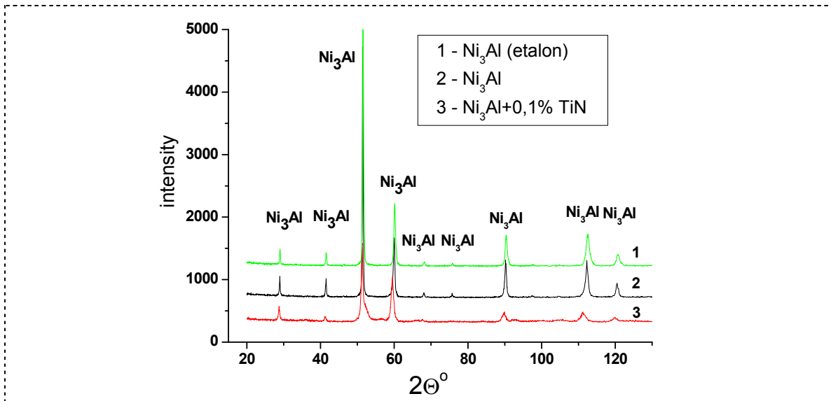
Figure 2. Diffractograms obtained from the reference specimen (1), from the patterns synthesized under pressure (2), and from the patterns synthesized under pressure with a 0.1 % of nanosized particles of a titanium nitride adding (3) of Ni 3 Al intermetallic compound.
