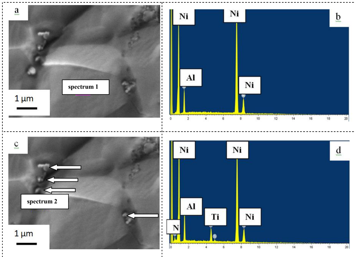
Figure 4. Fracture surface of a synthesized under pressure Ni 3 Al intermetallic compound with TiN nanoparticles (marked with arrows) (a, c) and energy spectra of a grain body element compound (b), and titanium nitride particles at the grain boundary (d).
