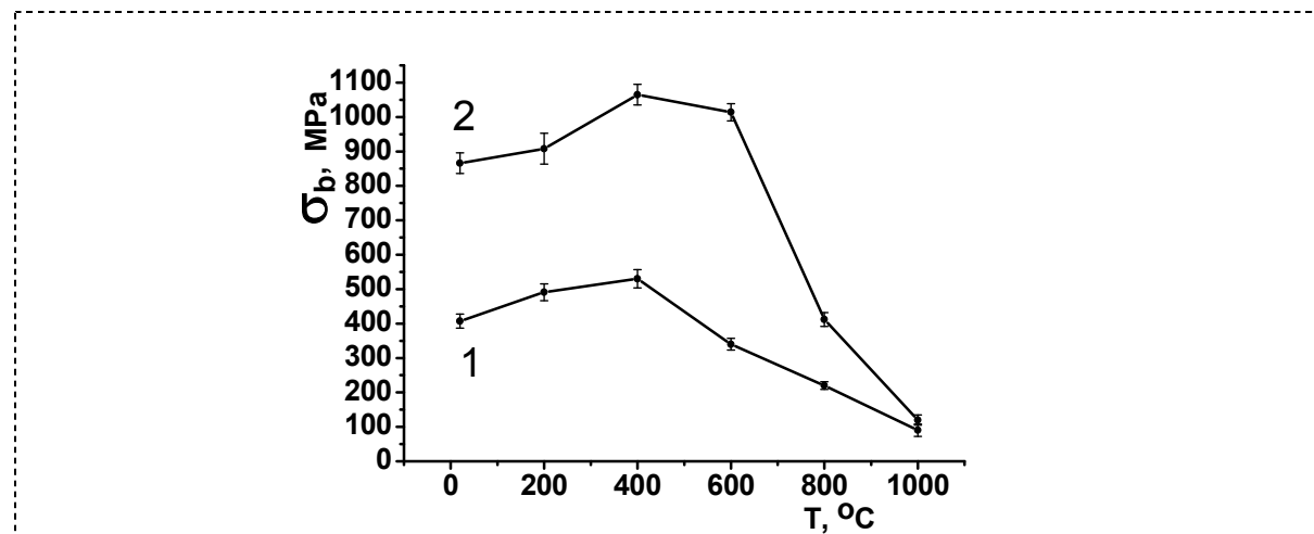
Fig.6. Temperature dependences of a Ni 3 Al intermetallic compound strength (1) and a Ni 3 Al intermetallic compound with 0.1% of TiN nanoparticles adding (2).
